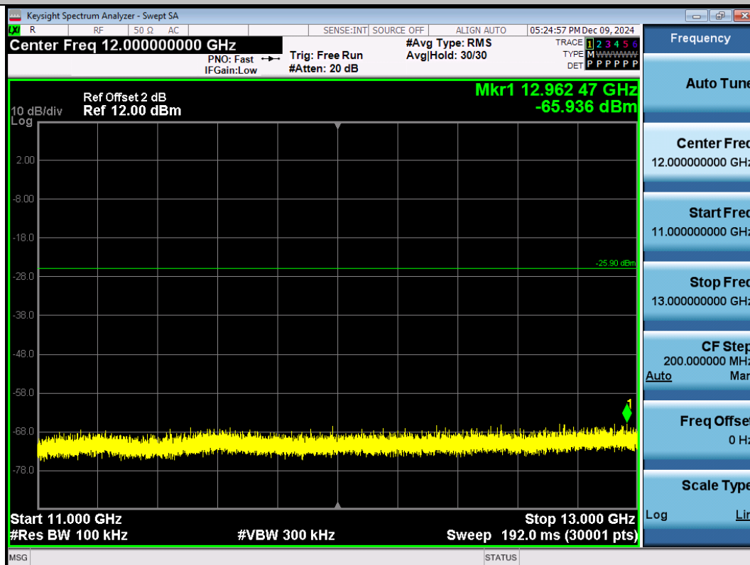
11N20SISO-Ant1-2437-11000~13000-PASS
