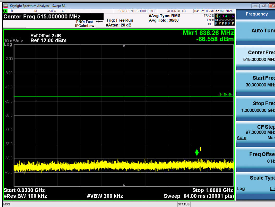
11G-Ant1-2412-30-1000-PASS
