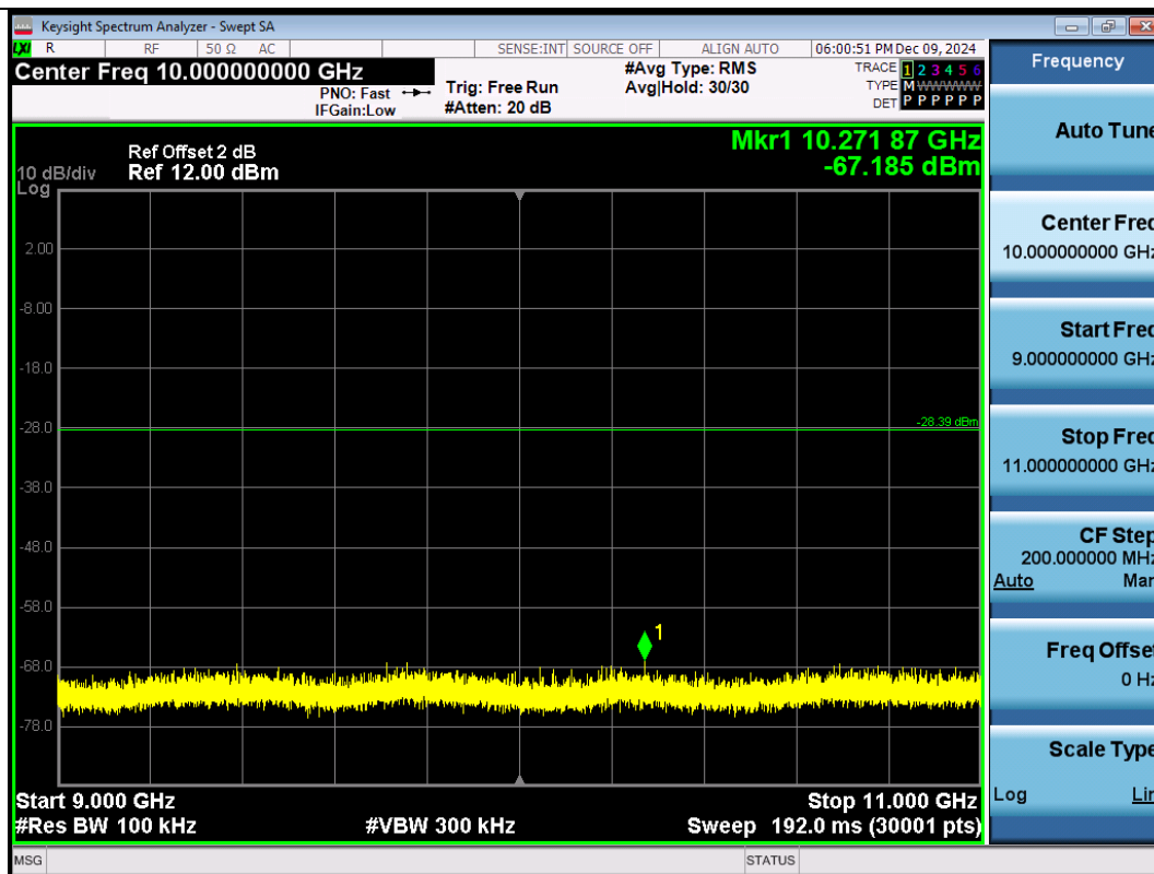
11N40SISO-Ant1-2422-9000~11000-PASS
