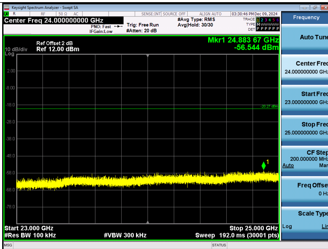
11B-Ant1-2462-23000-25000-PASS
