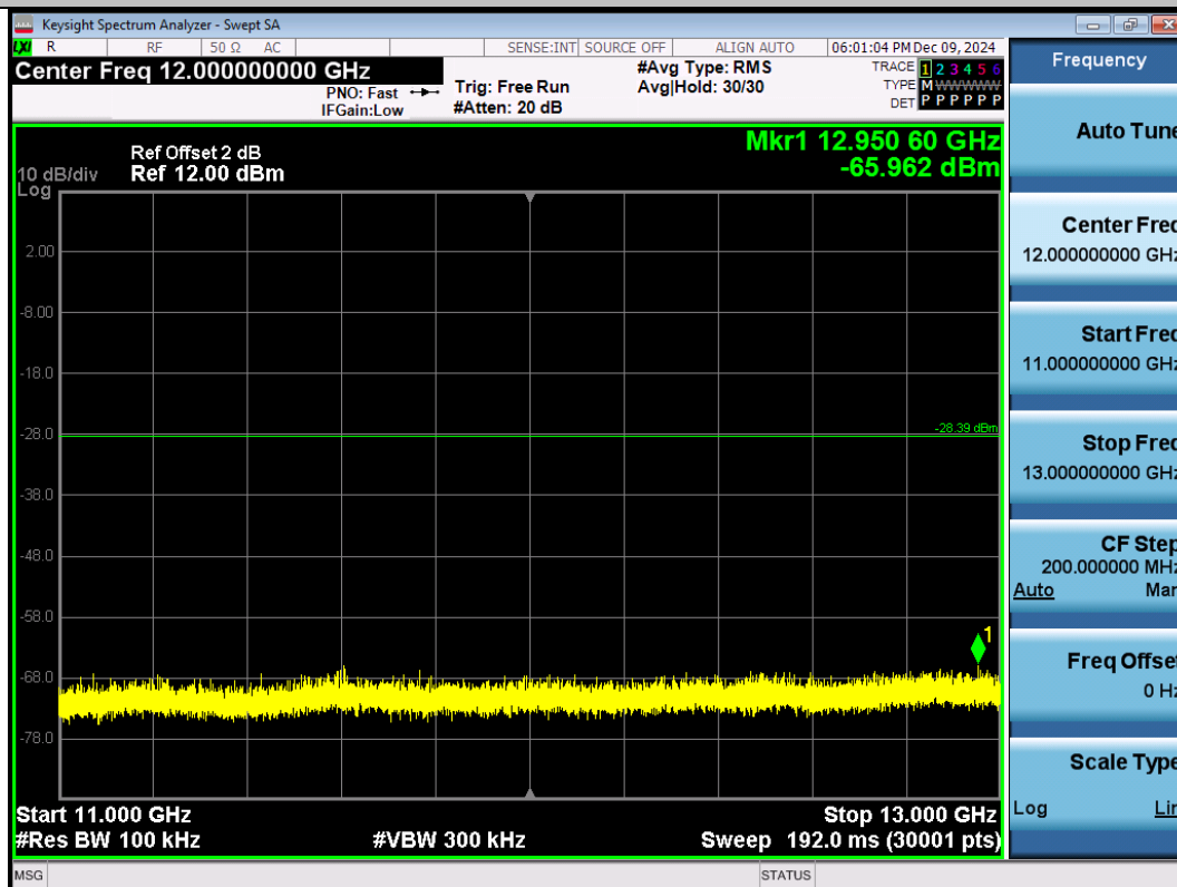
11N40SISO-Ant1-2422-11000~13000-PASS
