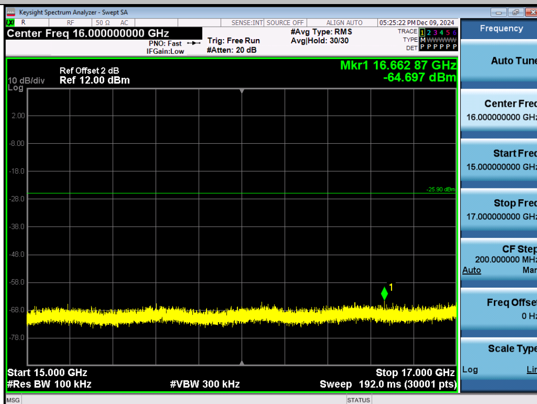
11N20SISO-Ant1-2437-15000~17000-PASS
