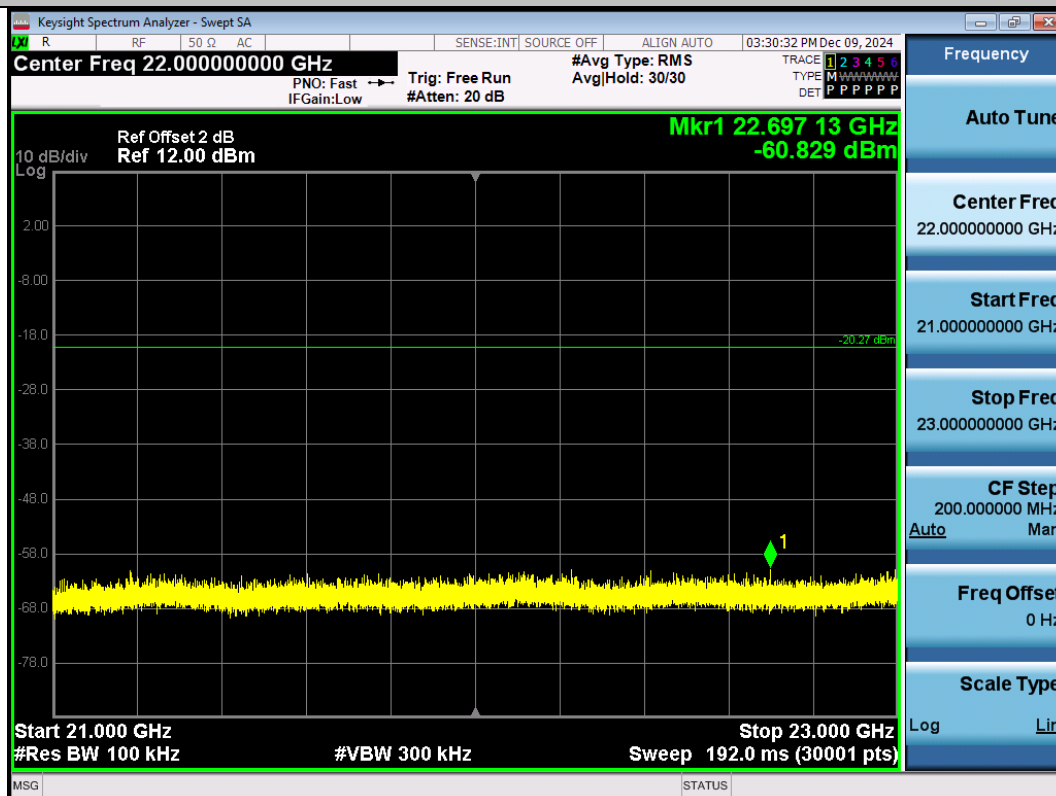
11B-Ant1-2462-21000~23000-PASS
