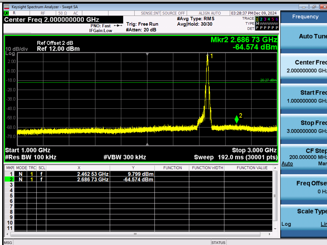
11B-Ant1-2462-1000~3000-PASS
