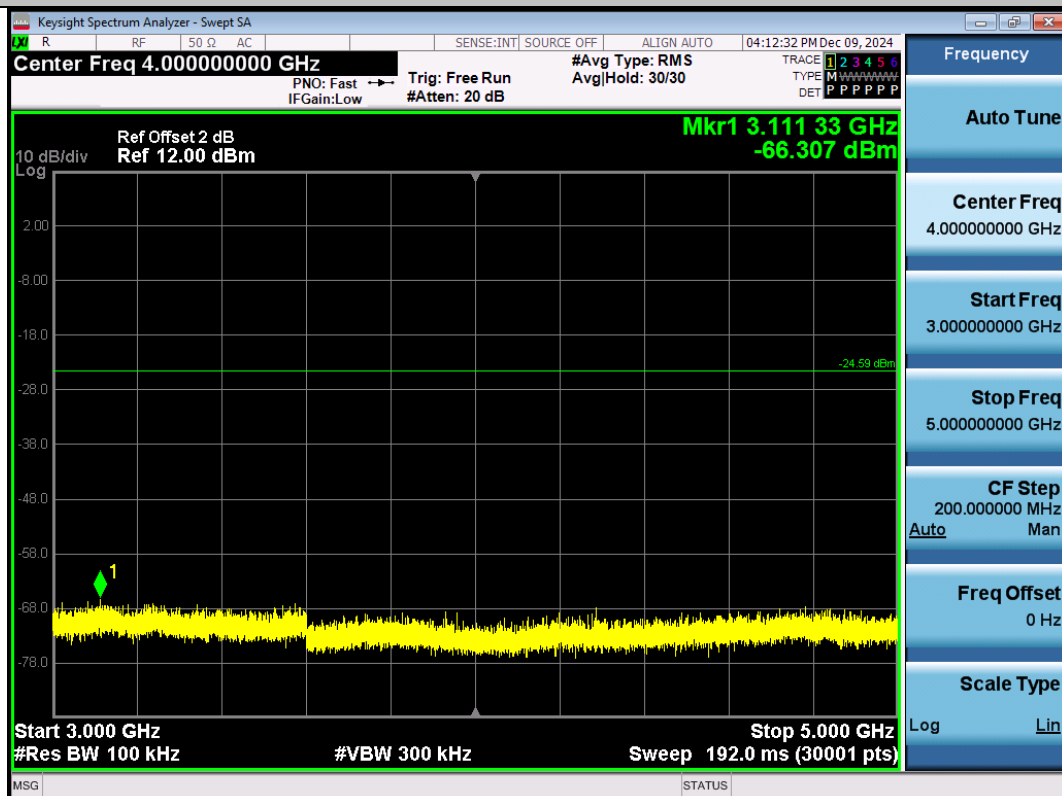
11G-Ant1-2412-3000~5000-PASS
