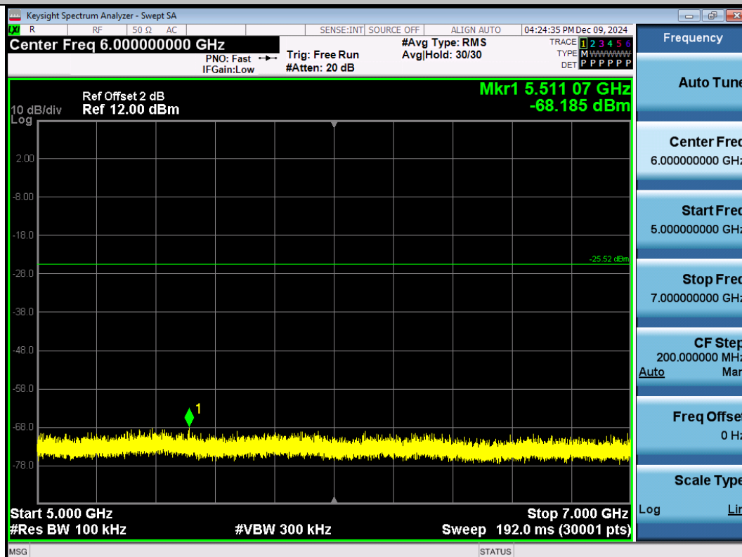
11G-Ant1-2437-5000~7000-PASS
