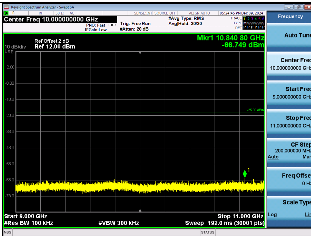
11N20SISO-Ant1-2437-9000~11000-PASS
