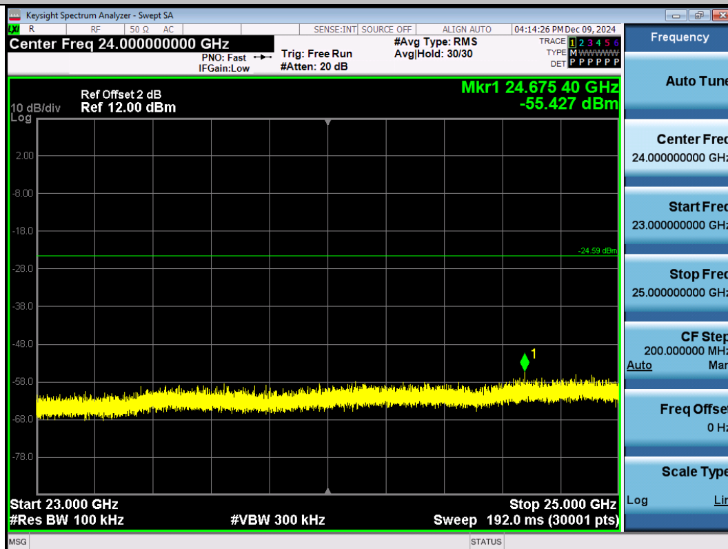
11G-Ant1-2412-23000~25000-PASS
