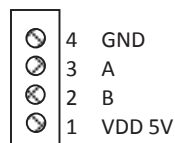
J13 RS-485 connector
