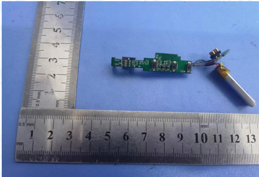
Photo 13 Appearance of PCB
