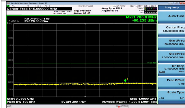
Band41_15MHz_16QAM_41165_1RB#0_30~1000_30~10 00
