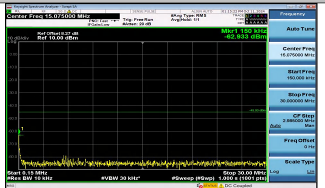
Band41_20MHz_QPSK_40340_1RB#0_0.15~30_0.15~30
