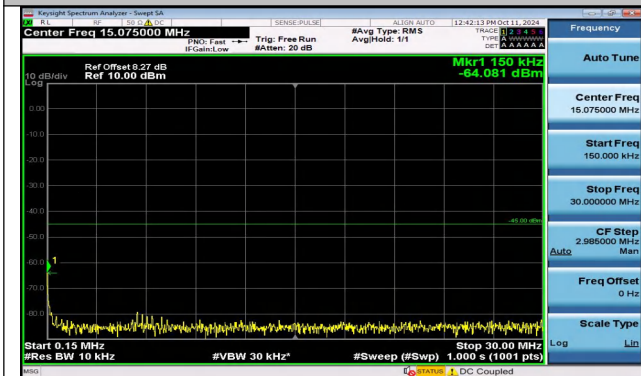
Band41_15MHz_QPSK_41165_1RB#74_0.15~30_0.15~3 0
