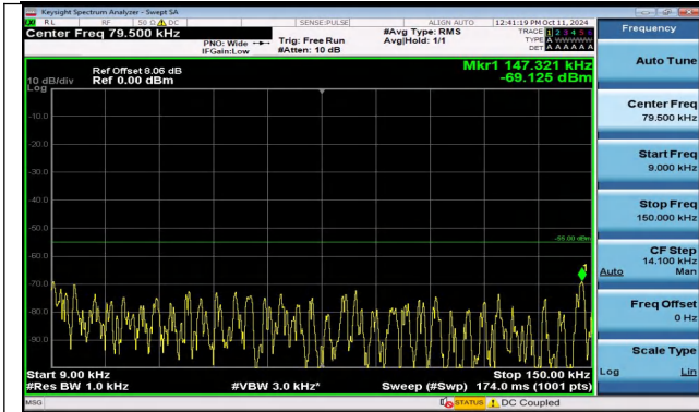
Band41_15MHz_16QAM_41165_1RB#0_0.009~0.15_0.00 9~0.15
