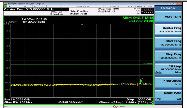
Band41_15MHz_QPSK_41165_1RB#74_30~1000_30~10 00
