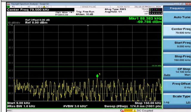
Band41_20MHz_QPSK_40340_1RB#0_0.009~0.15_0.009~0.15
