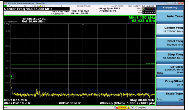
Band41_15MHz_16QAM_41165_1RB#0_0.15~30_0.15~3 0
