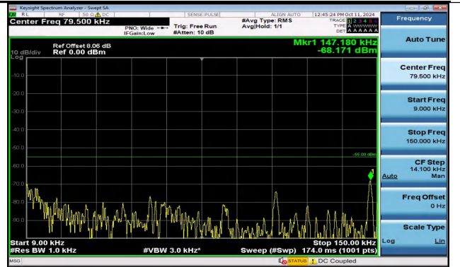
Band41_15MHz_QPSK_41165_75RB#0_0.009~0.15_0.009~0.15
