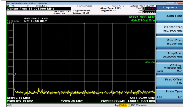
Band41_15MHz_QPSK_41165_75RB#0_0.15~30_0.15~30
