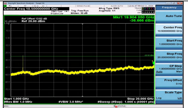
Band41_15MHz_16QAM_41165_1RB#0_1000~20000_10 00~20000
