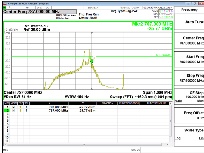
NB_IoT_Band13_15kHz_QPSK_1_0_CH23181
