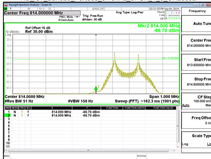
NB_IoT_Band26_Part90s_3.75kHz_BPSK_1_0_CH26692
