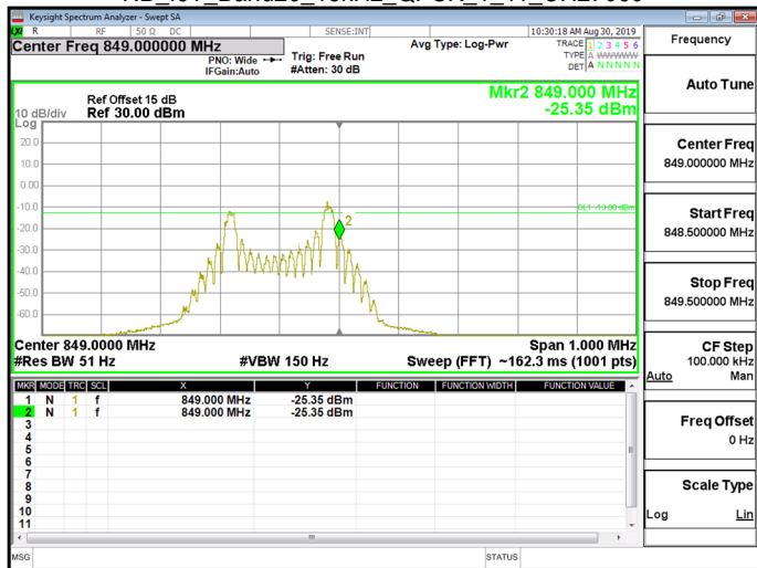
NB_IoT_Band26_15kHz_QPSK_1_11_CH27039
