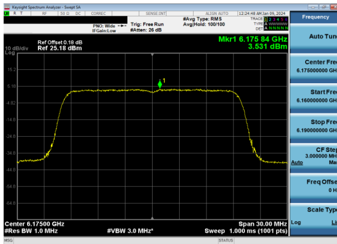
Plot 7-342. Power Spectral Density Plot Antenna WF2a Standard Power (20MHz 802.11ax (UNII Band 5) – Ch. 45, MCS4)
