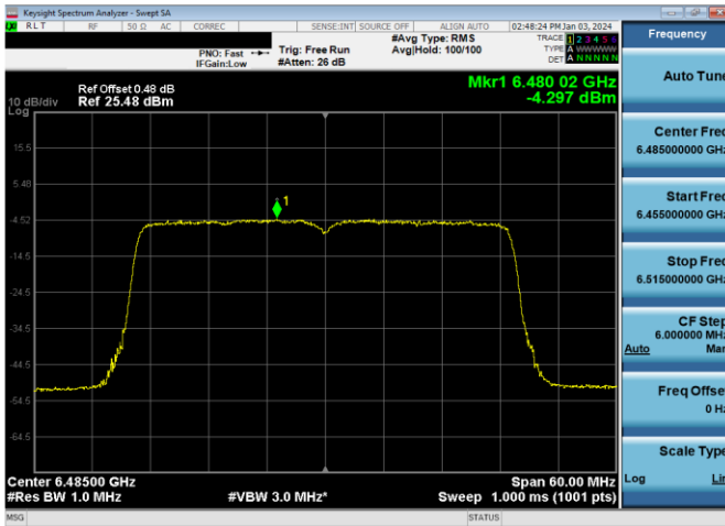
Plot 7-404. Power Spectral Density Plot Antenna WF7b LPI (40MHz 802.11ax (UNII Band 6) – Ch. 107, MCS11)
