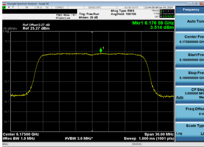
Plot 7-352. Power Spectral Density Plot Antenna WF2a Standard Power (20MHz 802.11ax (UNII Band 5) – Ch. 45, MCS11)
