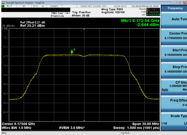
Plot 7-381. Power Spectral Density Plot Antenna WF7b LPI (20MHz 802.11a (UNII Band 5) – Ch. 45, 24Mbps)
