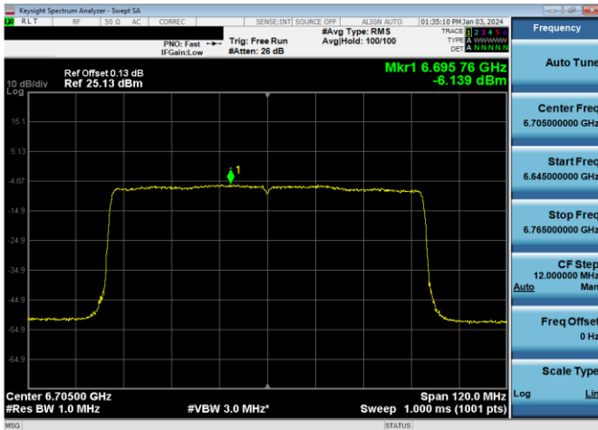
Plot 7-374. Power Spectral Density Plot Antenna WF7b LPI (80MHz 802.11ax (UNII Band 7) – Ch. 151, MCS2)
