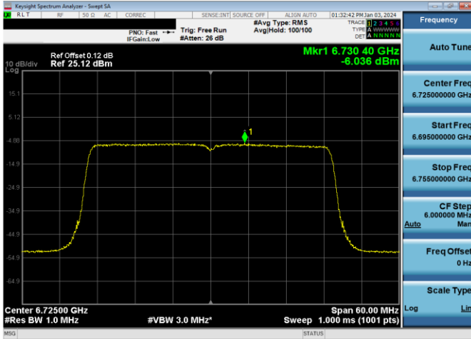
Plot 7-373. Power Spectral Density Plot Antenna WF7b LPI (40MHz 802.11ax (UNII Band 7) – Ch. 155, MCS2)
