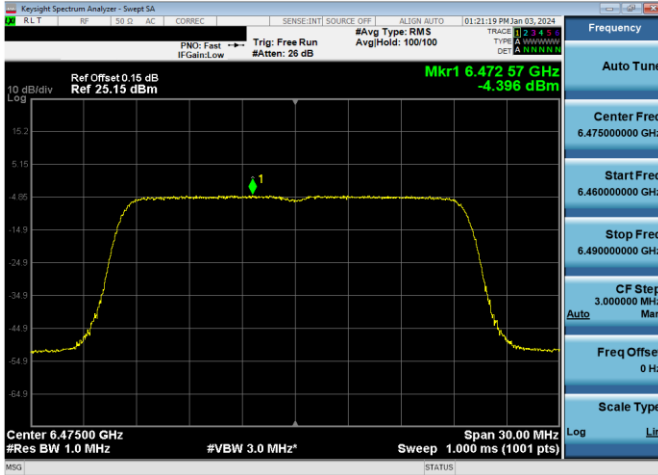
Plot 7-367. Power Spectral Density Plot Antenna WF7b LPI (20MHz 802.11ax (UNII Band 6) – Ch. 105, MCS2)
