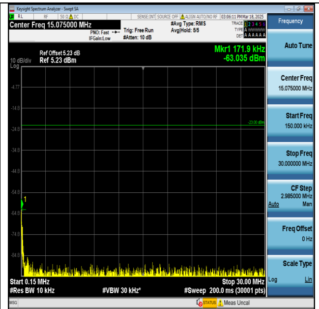
Band26(824-849)-15MHz-QPSK-26915-PASS1_Low
