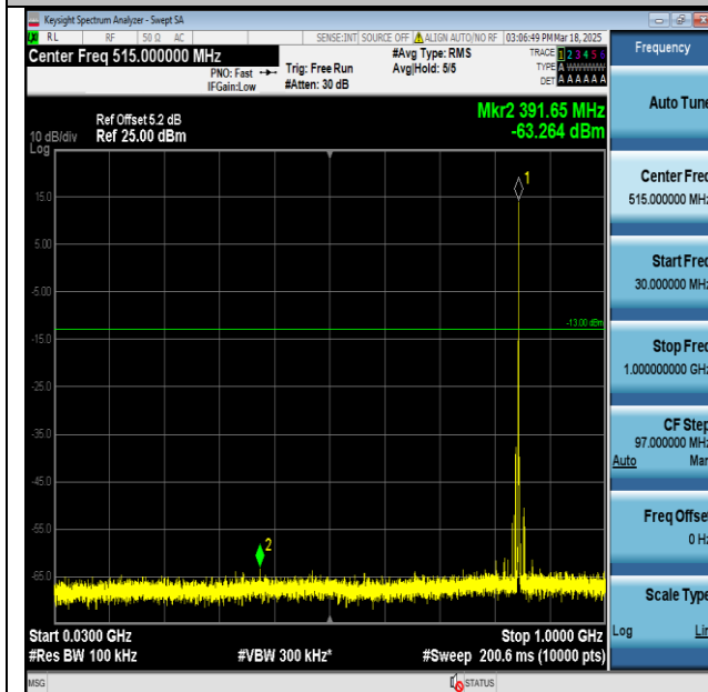
Band26(824-849)-15MHz-QPSK-26965-PASS_1_High
