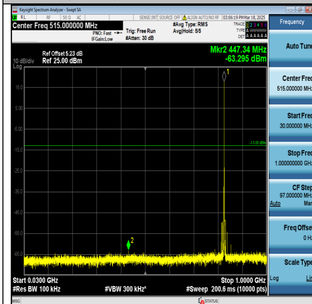
Band26(824-849)-15MHz-QPSK-26915-PASS1_Low
