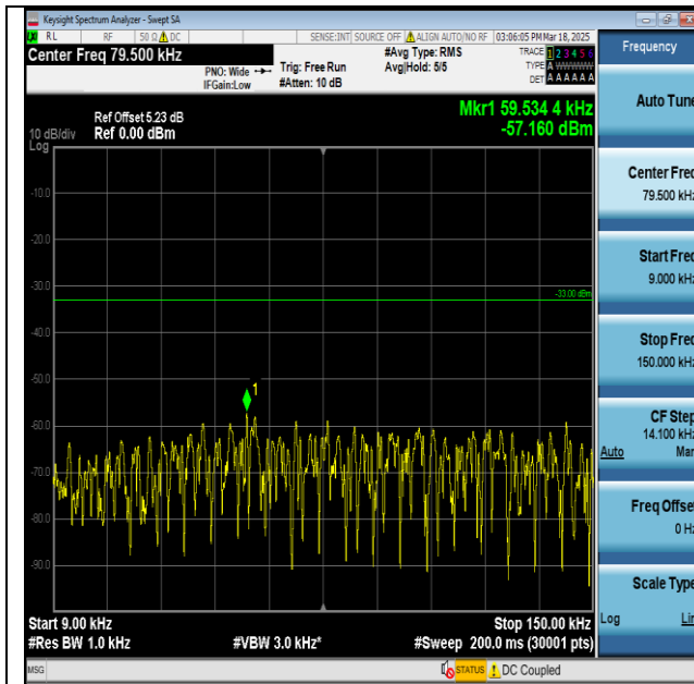
Band26(824-849)-15MHz-QPSK-26915-PASS1_Low
