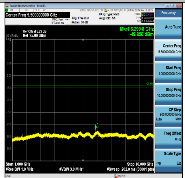
Band26(824-849)-15MHz-QPSK-26915-PASS1_Low
