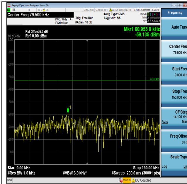
Band26(824-849)-15MHz-QPSK-26965-PASS_1_High
