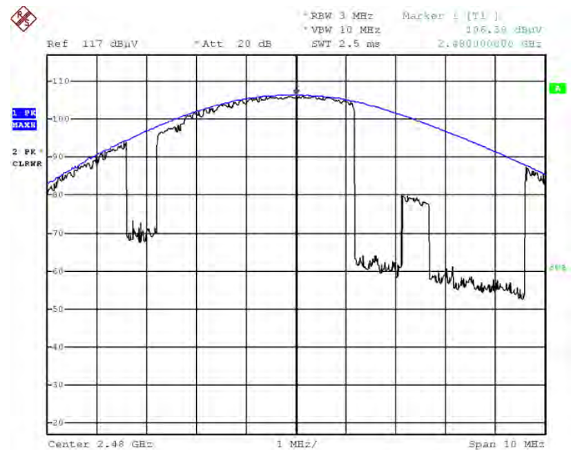
Radiated Power plot ( \pi /4QPSK, Ch78)
