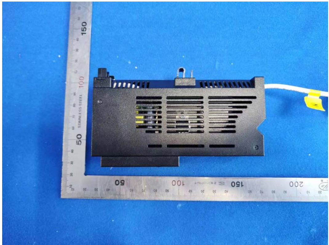
FIGURE 7 QO FORWARD PHASE DIMMER, PIGTAIL (M/N: GPM-Q2FPD05-21) BOTTOM
