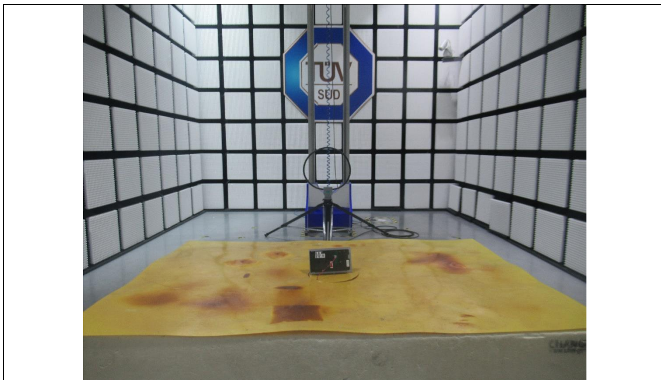
Radiated Emission test (9kHz to 30MHz)
