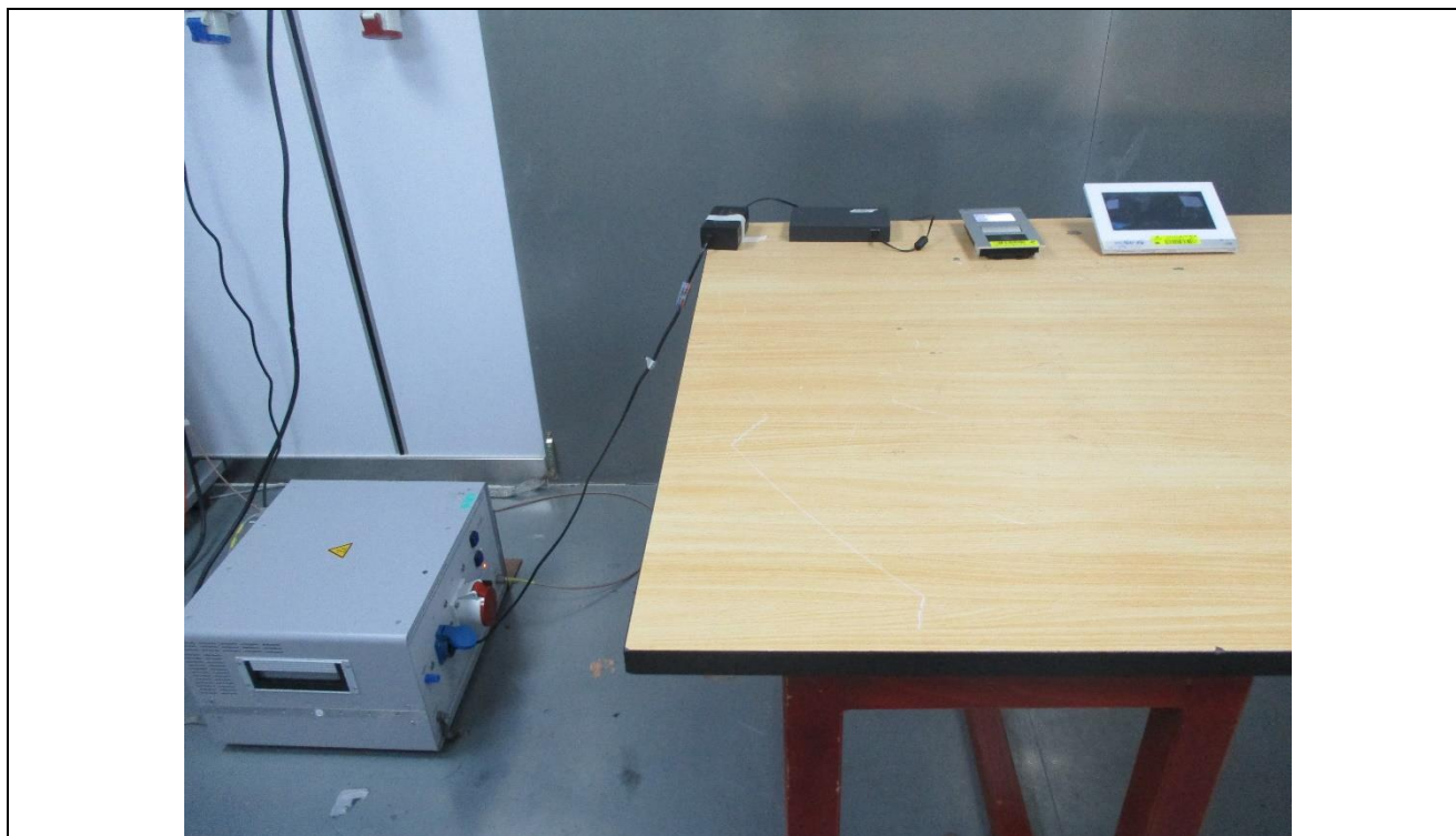
Conducted Emission test
