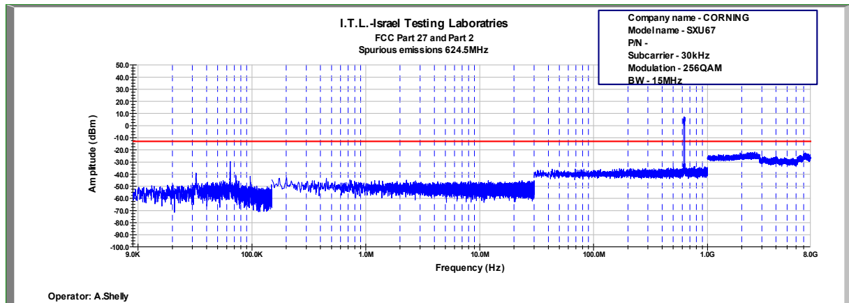
Figure 707: Spurious Emissions at Antenna Terminal 256QAM, 624.5MHz, B.W. 15MHz, Sub Carrier 30kHz
