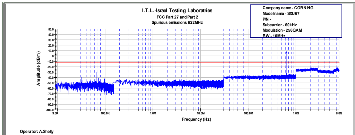
Figure 701: Spurious Emissions at Antenna Terminal 256QAM, 622.0MHz, B.W. 10MHz, Sub Carrier 60kHz
