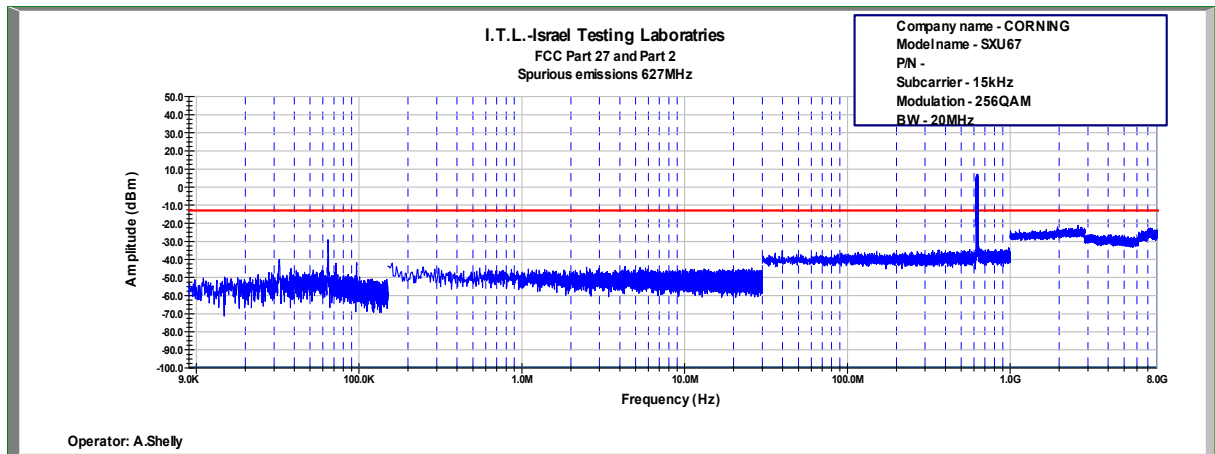
Figure 713: Spurious Emissions at Antenna Terminal 256QAM, 627.0MHz, B.W. 20MHz, Sub Carrier 15kHz
