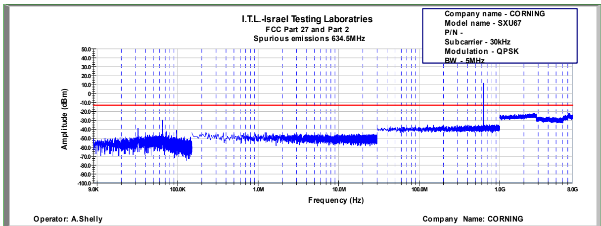
Figure 726: Spurious Emissions at Antenna Terminal QPSK, 634.5MHz, B.W. 5MHz, Sub Carrier 30kHz
