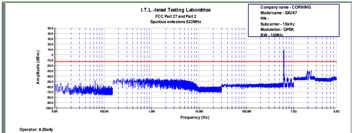
Figure 728: Spurious Emissions at Antenna Terminal QPSK, 622.0MHz, B.W. 10MHz, Sub Carrier 15kHz
