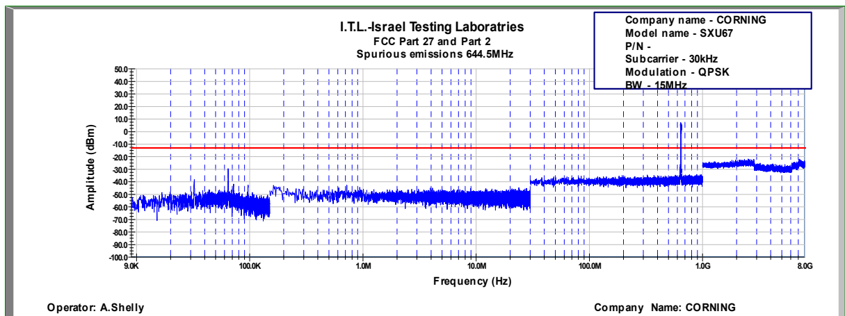
Figure 742: Spurious Emissions at Antenna Terminal QPSK, 644.5MHz, B.W. 15MHz, Sub Carrier 30kHz
