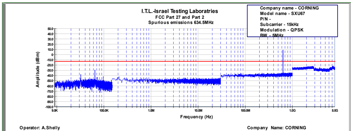
Figure 723: Spurious Emissions at Antenna Terminal QPSK, 634.5MHz, B.W. 5MHz, Sub Carrier 15kHz
