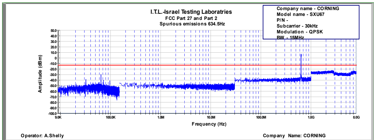
Figure 741: Spurious Emissions at Antenna Terminal QPSK, 634.5MHz, B.W. 15MHz, Sub Carrier 30kHz
