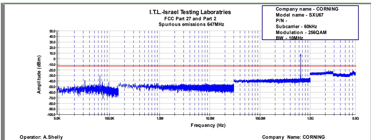
Figure 703: Spurious Emissions at Antenna Terminal 256QAM, 647.0MHz, B.W. 10MHz, Sub Carrier 60kHz
