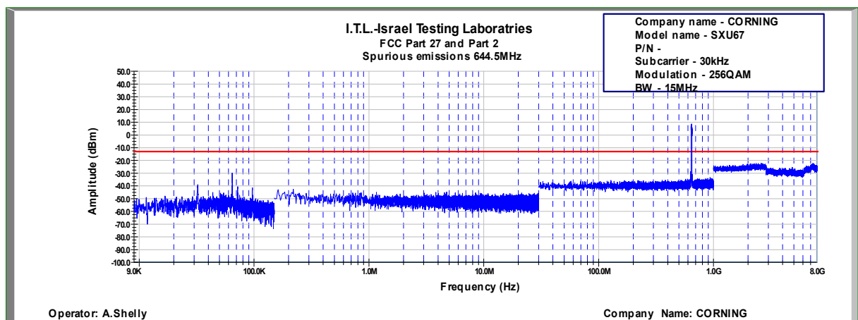
Figure 709: Spurious Emissions at Antenna Terminal 256QAM, 644.5MHz, B.W. 15MHz, Sub Carrier 30kHz
