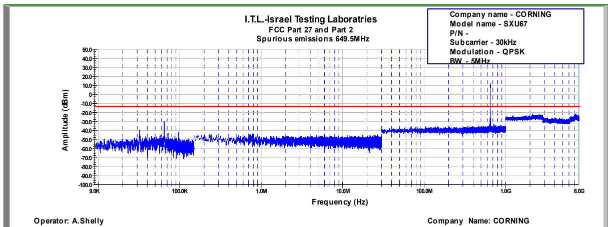
Figure 727: Spurious Emissions at Antenna Terminal QPSK, 649.5MHz, B.W. 5MHz, Sub Carrier 30kHz
