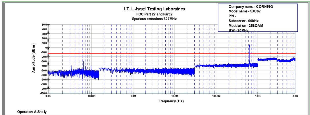
Figure 719: Spurious Emissions at Antenna Terminal 256QAM, 627.0MHz, B.W. 20MHz, Sub Carrier 60kHz
