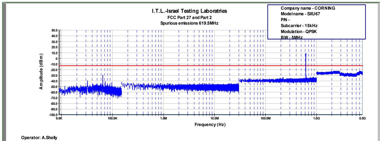
Figure 722: Spurious Emissions at Antenna Terminal QPSK, 619.5MHz, B.W. 5MHz, Sub Carrier 15kHz
