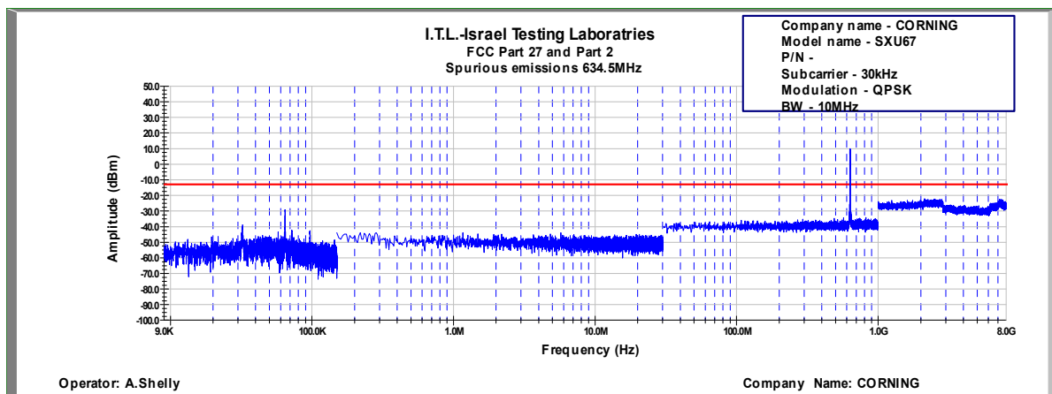
Figure 732: Spurious Emissions at Antenna Terminal QPSK, 634.5MHz, B.W. 10MHz, Sub Carrier 30kHz
