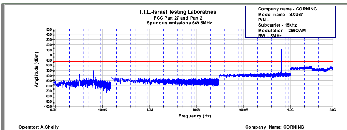
Figure 691: Spurious Emissions at Antenna Terminal 256QAM, 649.5MHz, B.W. 5MHz, Sub Carrier 15kHz
