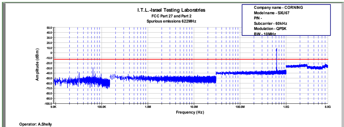
Figure 734: Spurious Emissions at Antenna Terminal QPSK, 622.0MHz, B.W. 10MHz, Sub Carrier 60kHz
