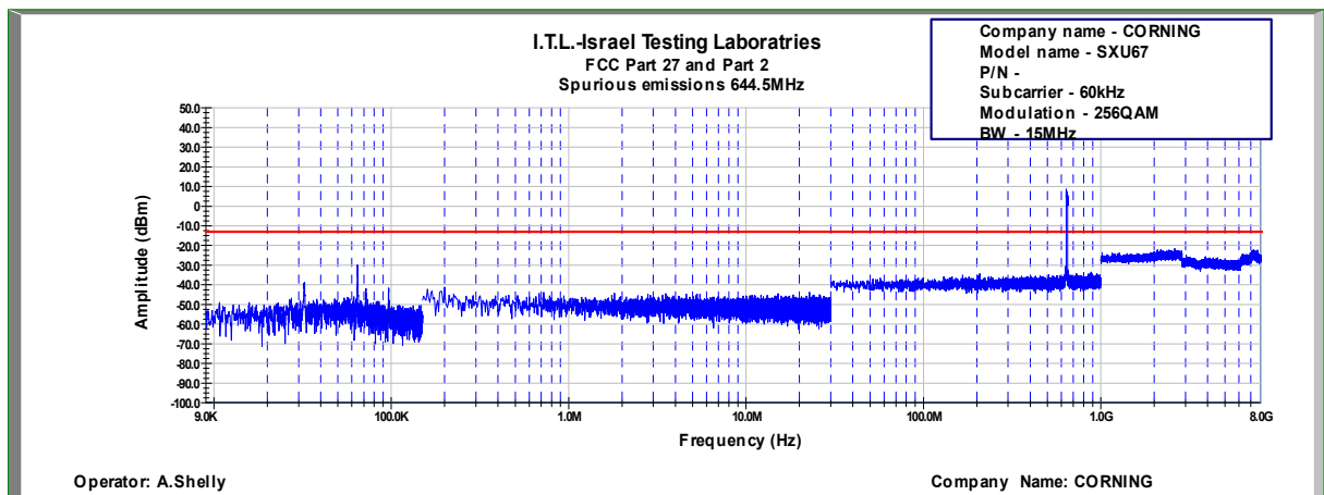
Figure 712: Spurious Emissions at Antenna Terminal 256QAM, 644.5MHz, B.W. 15MHz, Sub Carrier 60kHz
