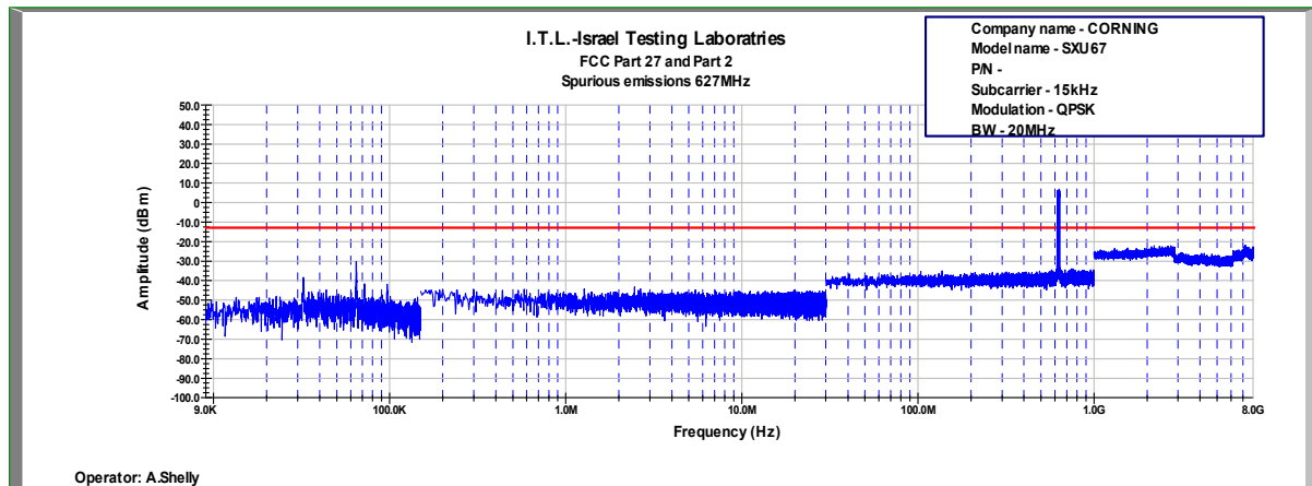
Figure 746: Spurious Emissions at Antenna Terminal QPSK, 627.0MHz, B.W. 20MHz, Sub Carrier 15kHz
