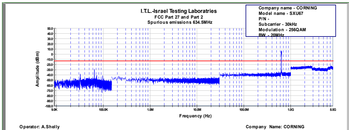
Figure 717: Spurious Emissions at Antenna Terminal 256QAM, 634.5MHz, B.W. 20MHz, Sub Carrier 30kHz
