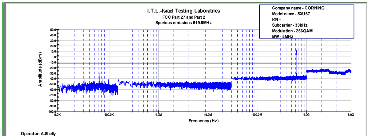
Figure 692: Spurious Emissions at Antenna Terminal 256QAM, 619.5MHz, B.W. 5MHz, Sub Carrier 30kHz
