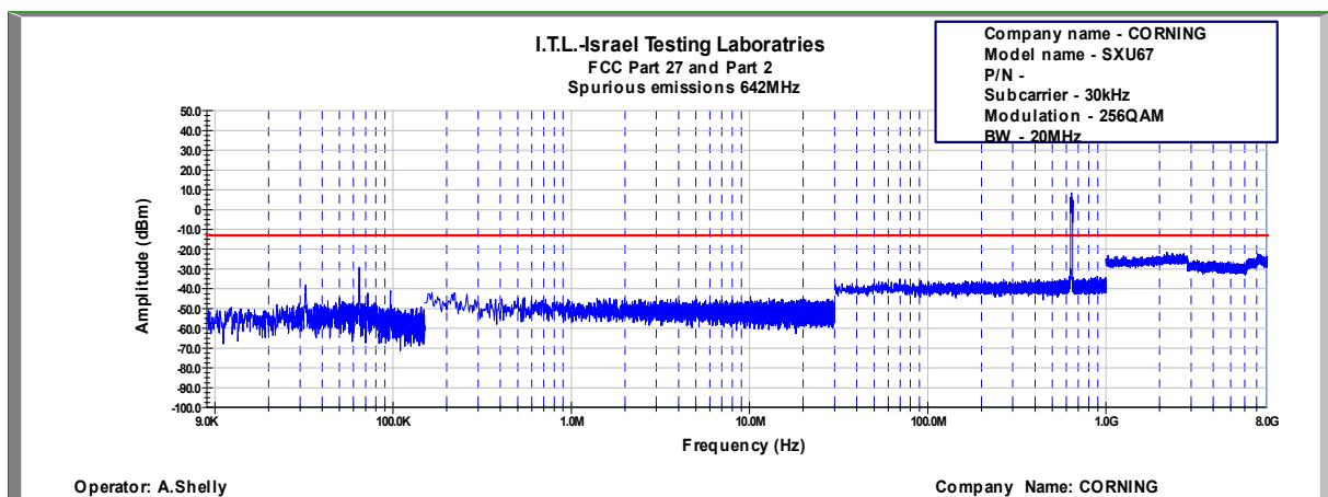
Figure 718: Spurious Emissions at Antenna Terminal 256QAM, 642.0MHz, B.W. 20MHz, Sub Carrier 30kHz
