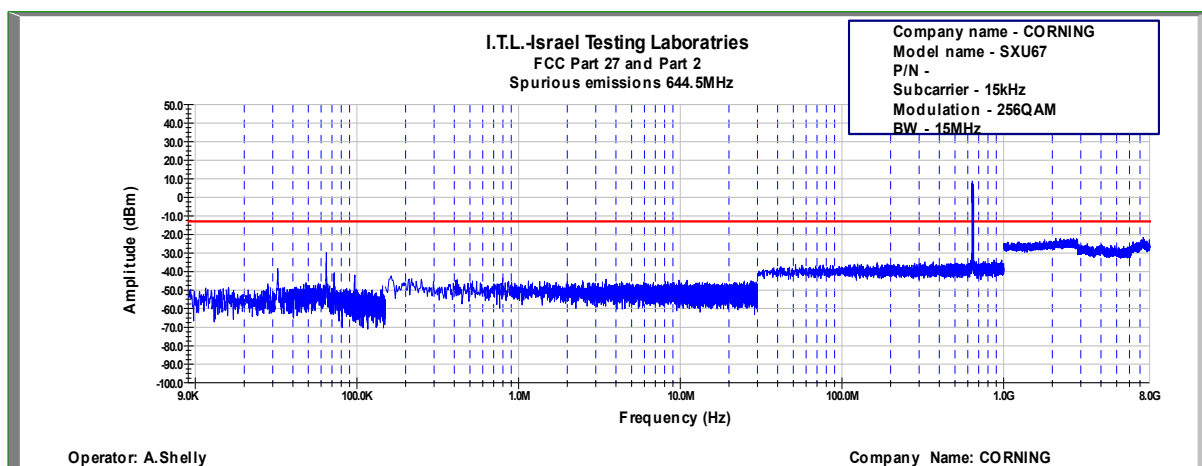
Figure 706: Spurious Emissions at Antenna Terminal 256QAM, 644.5MHz, B.W. 15MHz, Sub Carrier 15kHz
