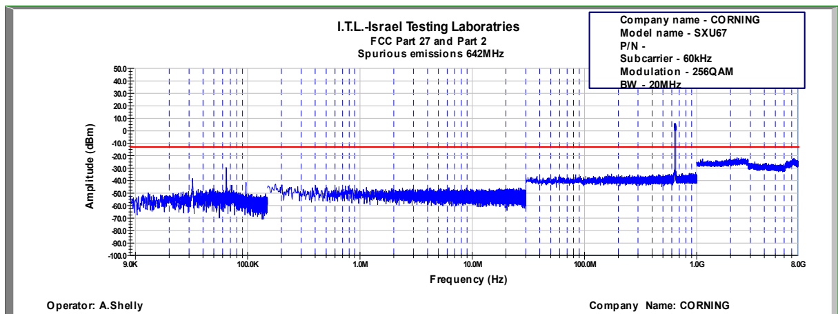
Figure 721: Spurious Emissions at Antenna Terminal 256QAM, 642.0MHz, B.W. 20MHz, Sub Carrier 60kHz
