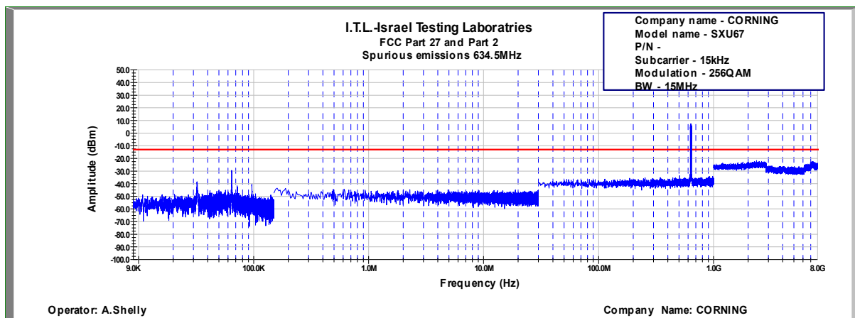
Figure 705: Spurious Emissions at Antenna Terminal 256QAM, 634.5MHz, B.W. 15MHz, Sub Carrier 15kHz
