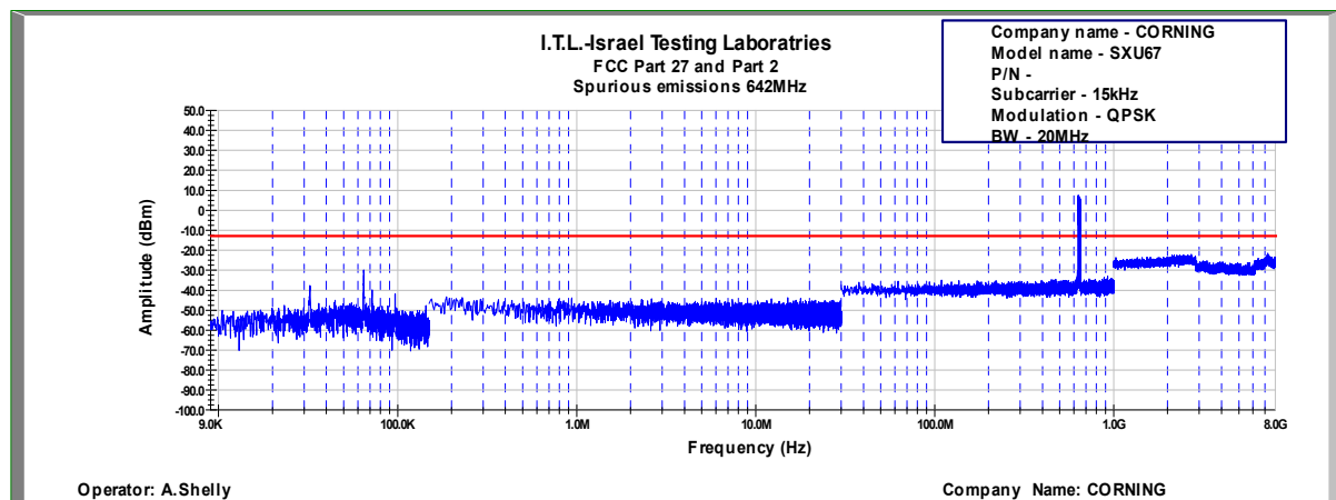
Figure 748: Spurious Emissions at Antenna Terminal QPSK, 642.0MHz, B.W. 20MHz, Sub Carrier 15kHz
