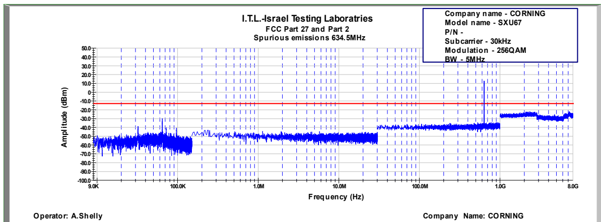
Figure 693: Spurious Emissions at Antenna Terminal 256QAM, 634.5MHz, B.W. 5MHz, Sub Carrier 30kHz
