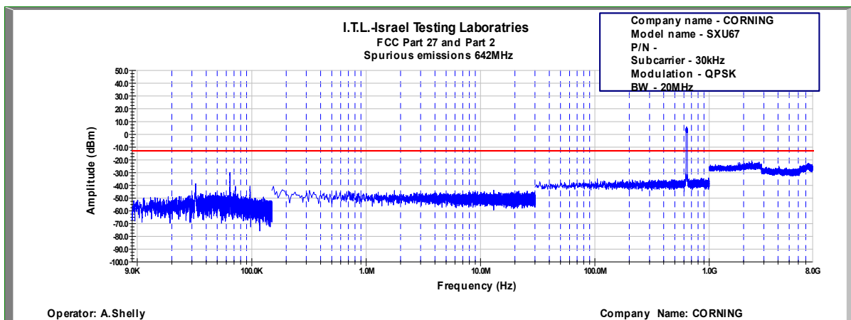
Figure 751: Spurious Emissions at Antenna Terminal QPSK, 642.0MHz, B.W. 20MHz, Sub Carrier 30kHz
