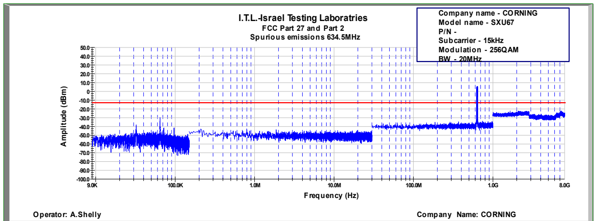
Figure 714: Spurious Emissions at Antenna Terminal 256QAM, 634.5MHz, B.W. 20MHz, Sub Carrier 15kHz
