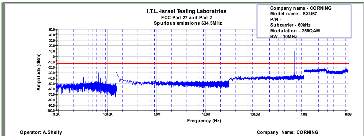
Figure 702: Spurious Emissions at Antenna Terminal 256QAM, 634.5MHz, B.W. 10MHz, Sub Carrier 60kHz
