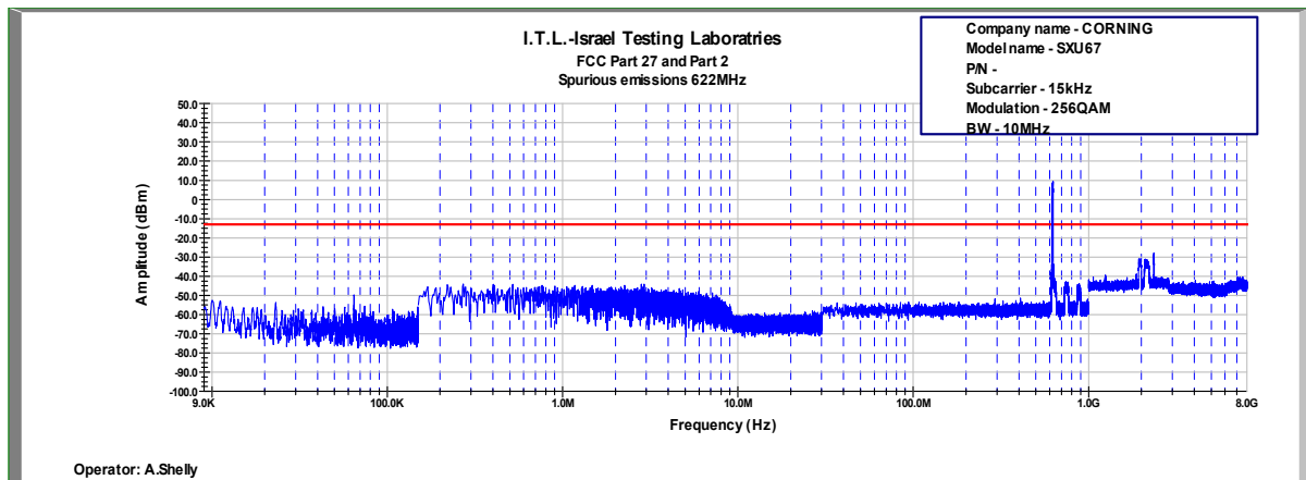
Figure 695: Spurious Emissions at Antenna Terminal 256QAM, 622.0MHz, B.W. 10MHz, Sub Carrier 15kHz
