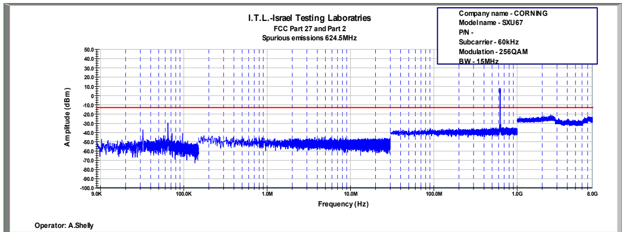
Figure 710: Spurious Emissions at Antenna Terminal 256QAM, 624.5MHz, B.W. 15MHz, Sub Carrier 60kHz
