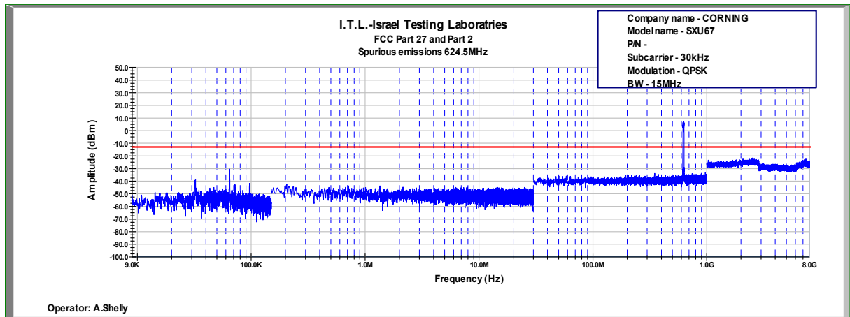
Figure 740: Spurious Emissions at Antenna Terminal QPSK, 624.5MHz, B.W. 15MHz, Sub Carrier 30kHz
