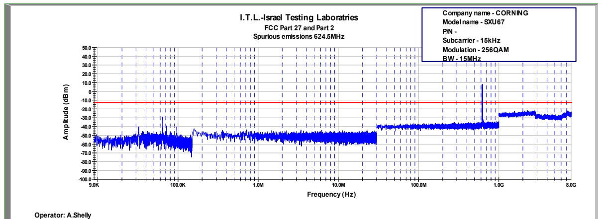
Figure 704: Spurious Emissions at Antenna Terminal 256QAM, 624.5MHz, B.W. 15MHz, Sub Carrier 15kHz
