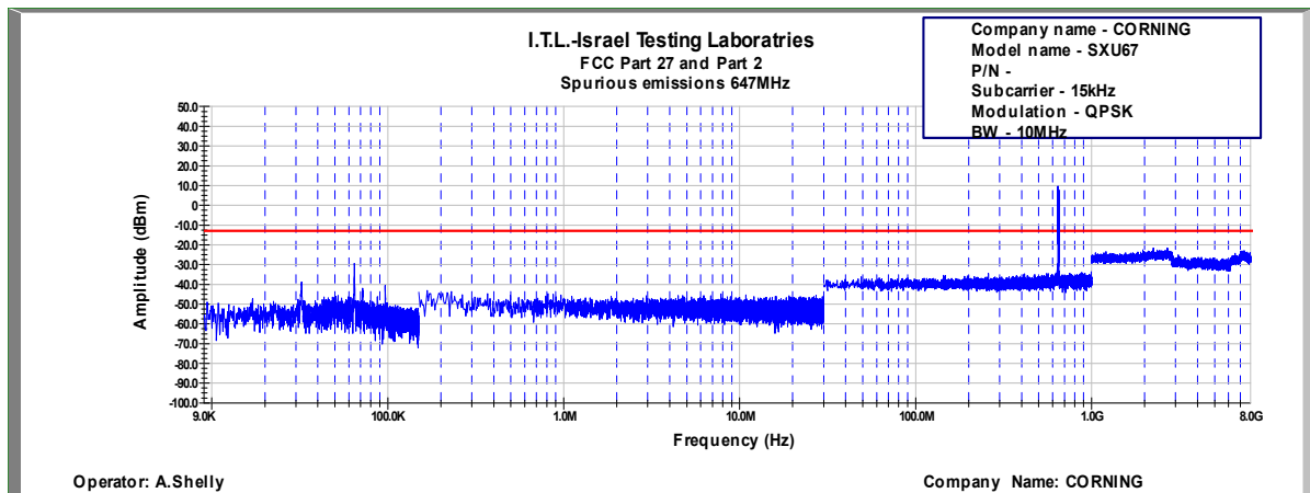
Figure 730: Spurious Emissions at Antenna Terminal QPSK, 647.0MHz, B.W. 10MHz, Sub Carrier 15kHz
