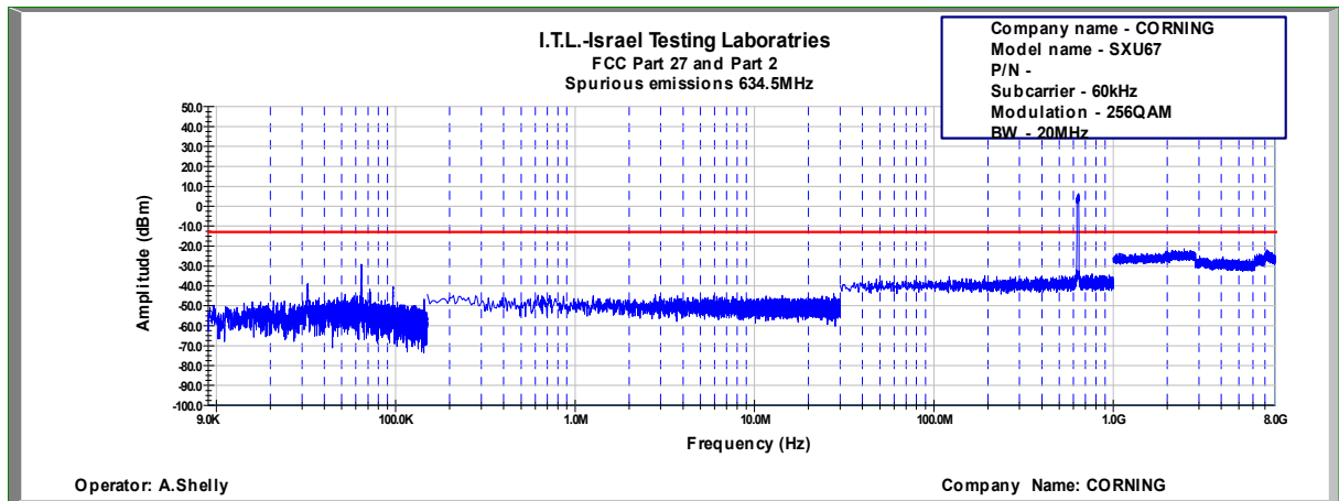
Figure 720: Spurious Emissions at Antenna Terminal 256QAM, 634.5MHz, B.W. 20MHz, Sub Carrier 60kHz
