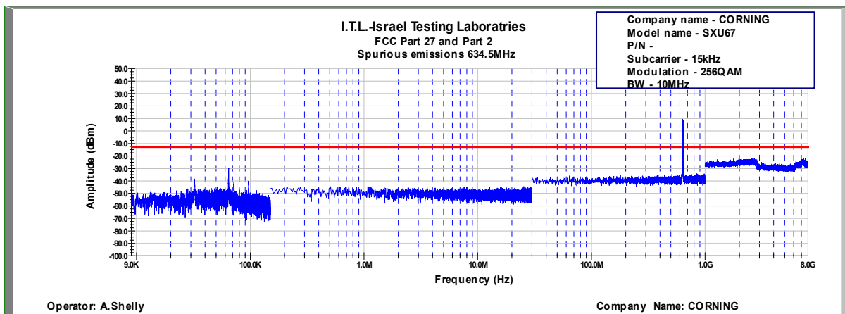
Figure 696: Spurious Emissions at Antenna Terminal 256QAM, 634.5MHz, B.W. 10MHz, Sub Carrier 15kHz
