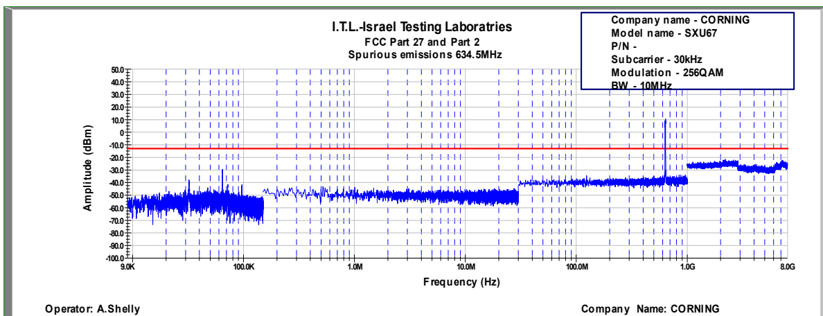
Figure 699: Spurious Emissions at Antenna Terminal 256QAM, 634.5MHz, B.W. 10MHz, Sub Carrier 30kHz
