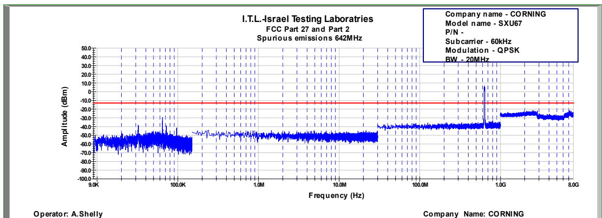
Figure 754: Spurious Emissions at Antenna Terminal QPSK, 642.0MHz, B.W. 20MHz, Sub Carrier 60kHz
