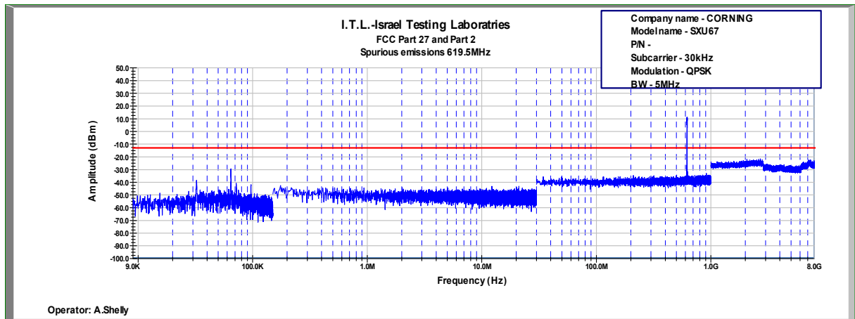
Figure 725: Spurious Emissions at Antenna Terminal QPSK, 619.5MHz, B.W. 5MHz, Sub Carrier 30kHz
