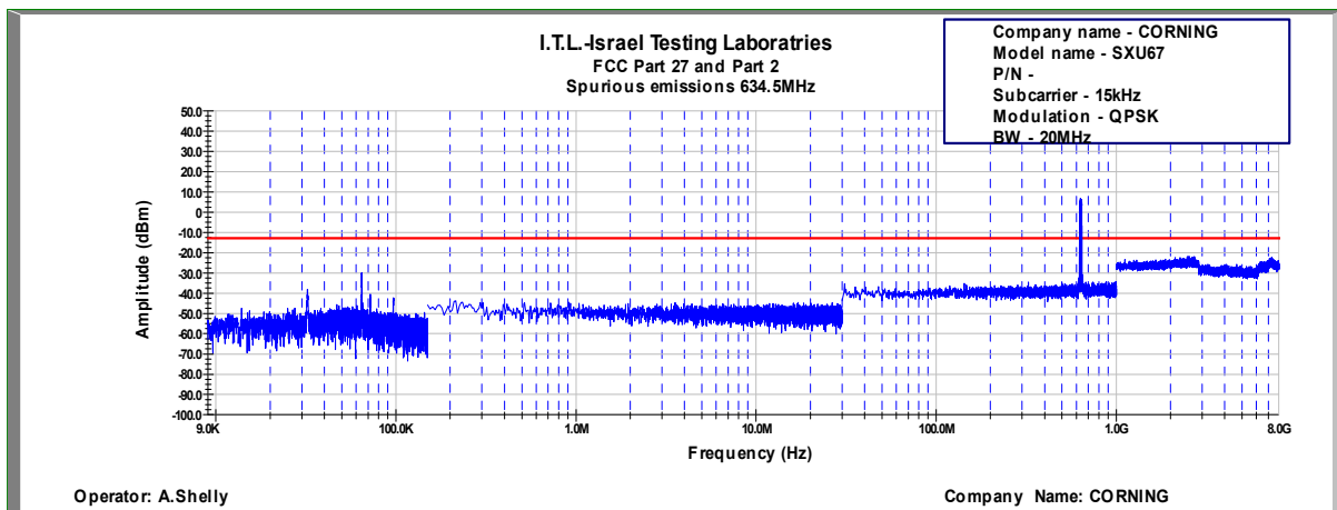
Figure 747: Spurious Emissions at Antenna Terminal QPSK, 634.5MHz, B.W. 20MHz, Sub Carrier 15kHz
