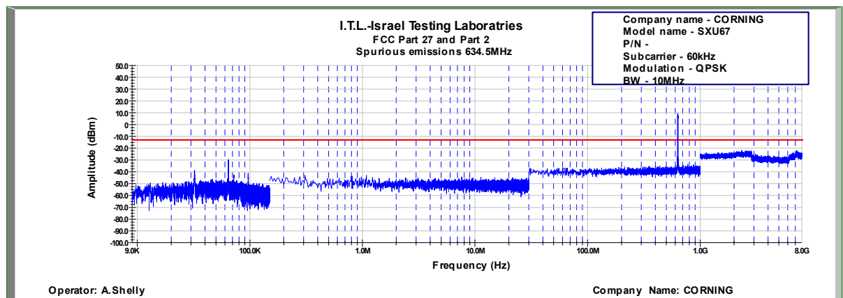
Figure 735: Spurious Emissions at Antenna Terminal QPSK, 634.5MHz, B.W. 10MHz, Sub Carrier 60kHz
