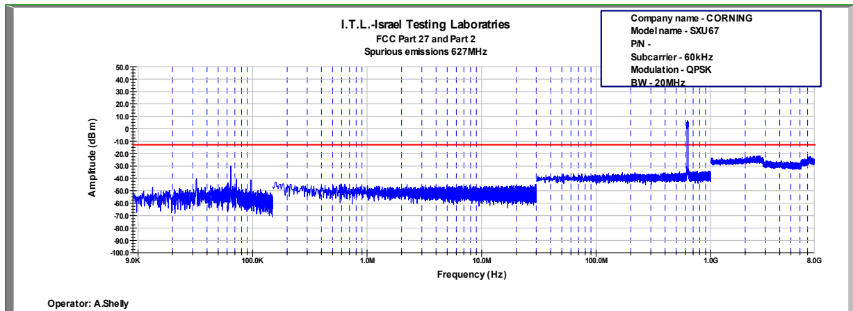
Figure 752: Spurious Emissions at Antenna Terminal QPSK, 627.0MHz, B.W. 20MHz, Sub Carrier 60kHz
