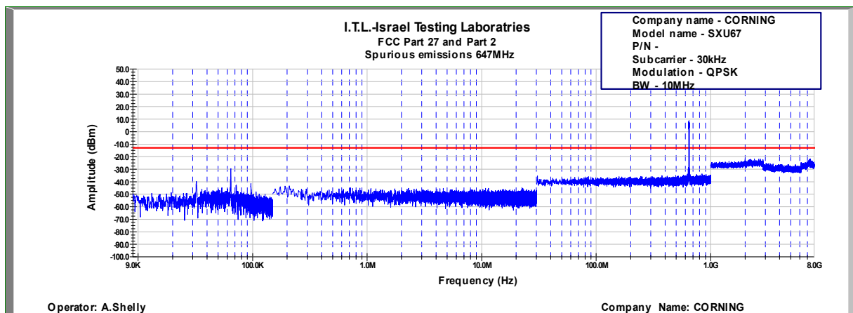
Figure 733: Spurious Emissions at Antenna Terminal QPSK, 647.0MHz, B.W. 10MHz, Sub Carrier 30kHz
