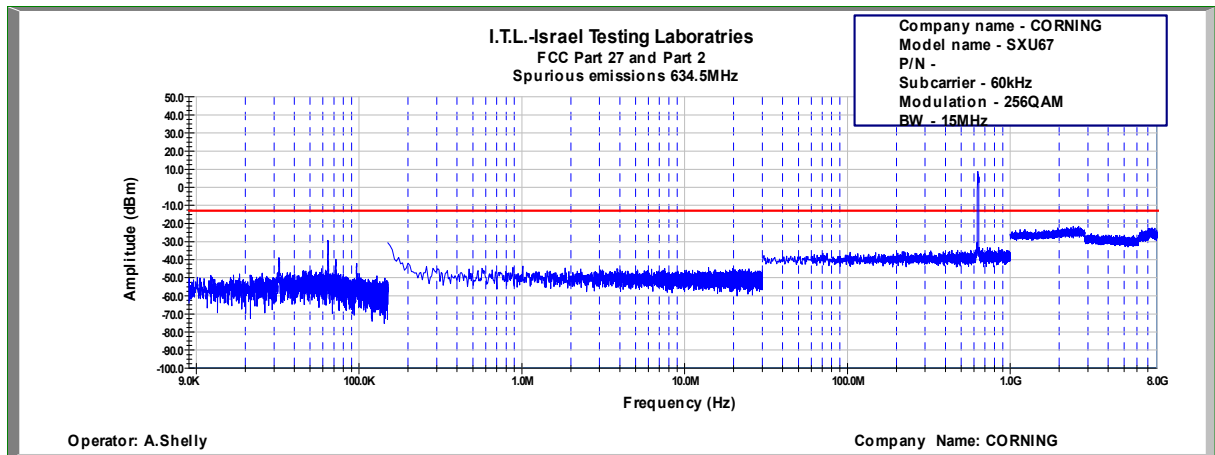
Figure 711: Spurious Emissions at Antenna Terminal 256QAM, 634.5MHz, B.W. 15MHz, Sub Carrier 60kHz
