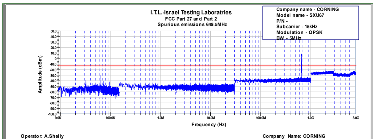
Figure 724: Spurious Emissions at Antenna Terminal QPSK, 649.5MHz, B.W. 5MHz, Sub Carrier 15kHz
