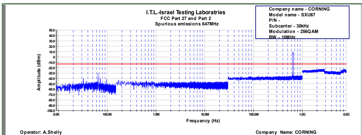
Figure 700: Spurious Emissions at Antenna Terminal 256QAM, 647.0MHz, B.W. 10MHz, Sub Carrier 30kHz
