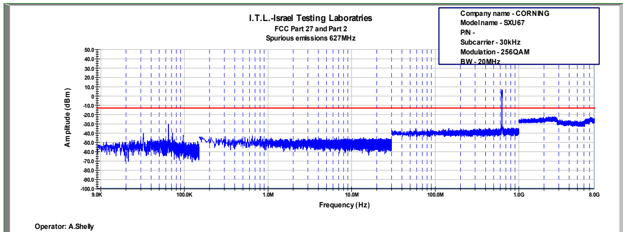
Figure 716: Spurious Emissions at Antenna Terminal 256QAM, 627.0MHz, B.W. 20MHz, Sub Carrier 30kHz
