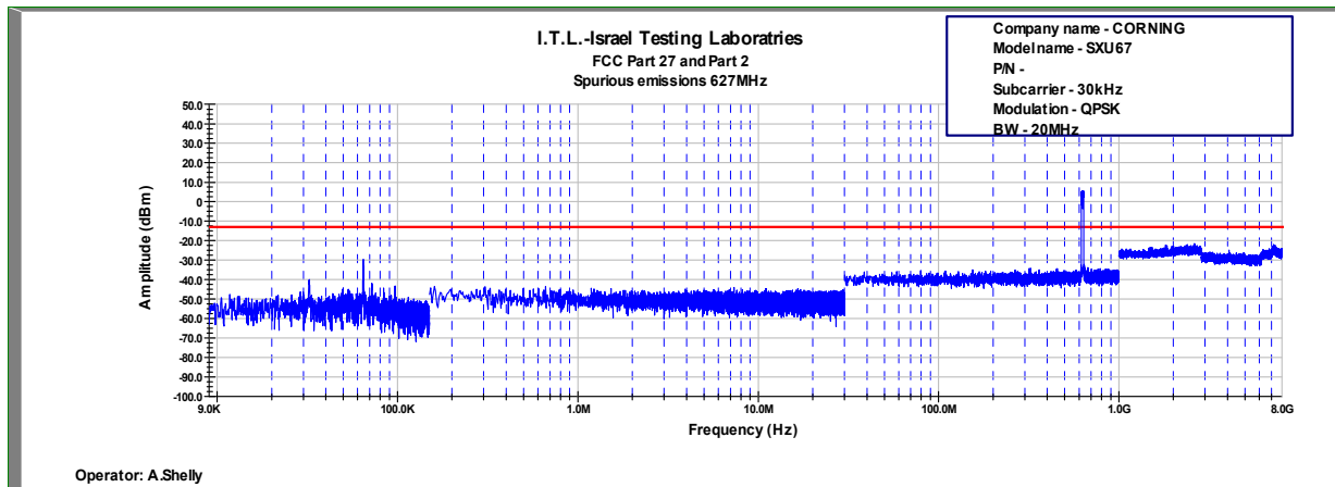
Figure 749: Spurious Emissions at Antenna Terminal QPSK, 627.0MHz, B.W. 20MHz, Sub Carrier 30kHz
