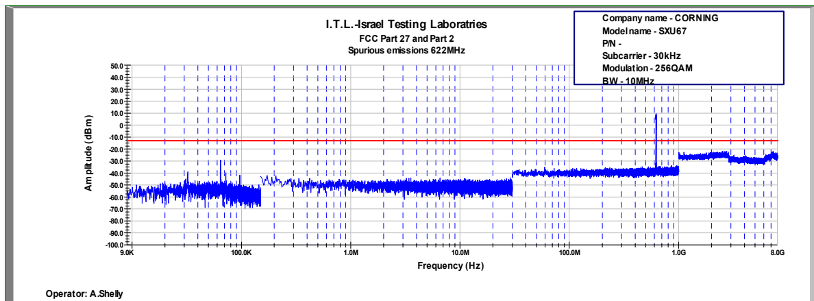
Figure 698: Spurious Emissions at Antenna Terminal 256QAM, 622.0MHz, B.W. 10MHz, Sub Carrier 30kHz
