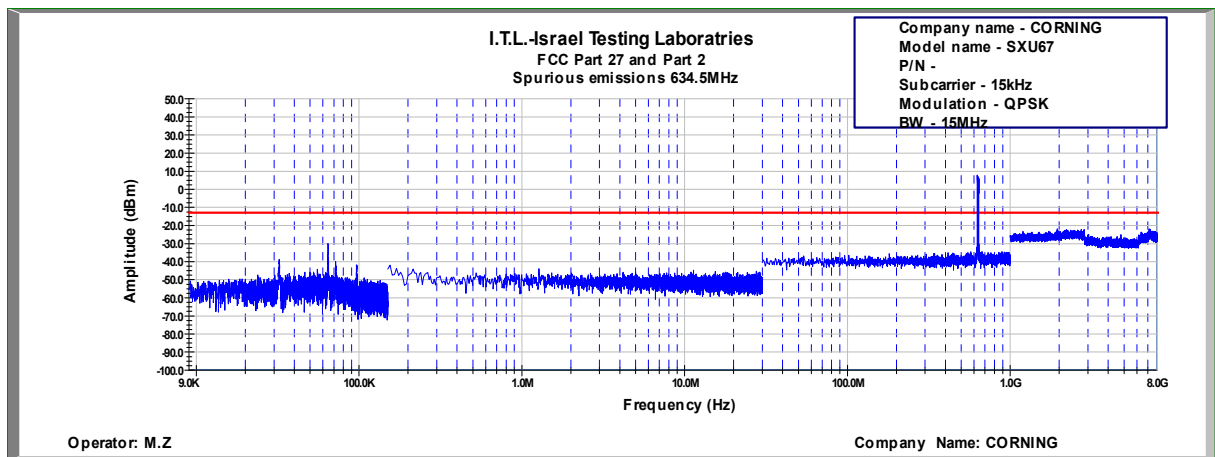
Figure 738: Spurious Emissions at Antenna Terminal QPSK, 634.5MHz, B.W. 15MHz, Sub Carrier 15kHz
