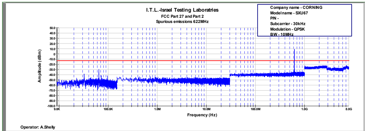
Figure 731: Spurious Emissions at Antenna Terminal QPSK, 622.0MHz, B.W. 10MHz, Sub Carrier 30kHz
