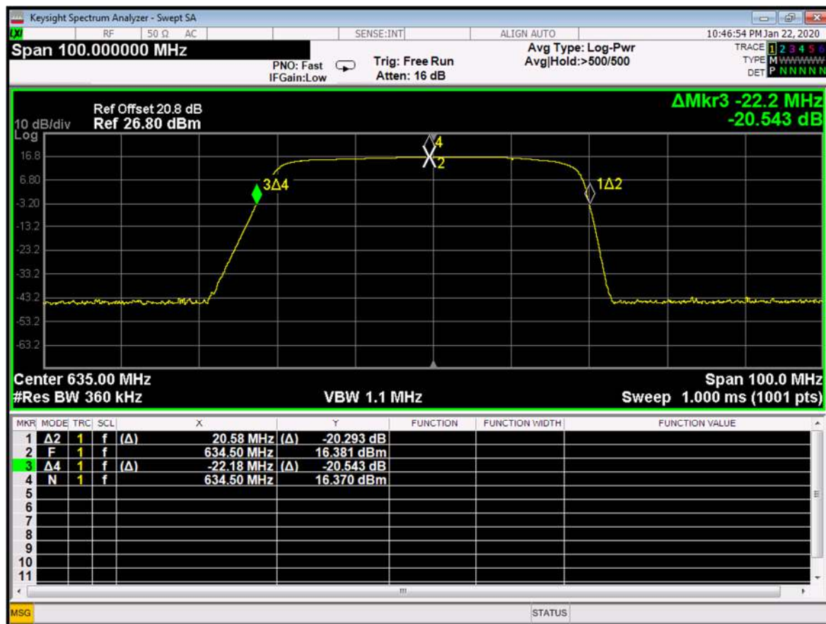
Figure 755. — Out-of-Band Rejection Plot
