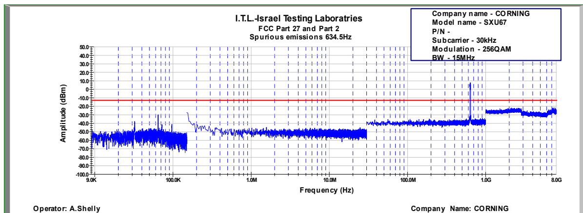
Figure 708: Spurious Emissions at Antenna Terminal 256QAM, 634.5MHz, B.W. 15MHz, Sub Carrier 30kHz
