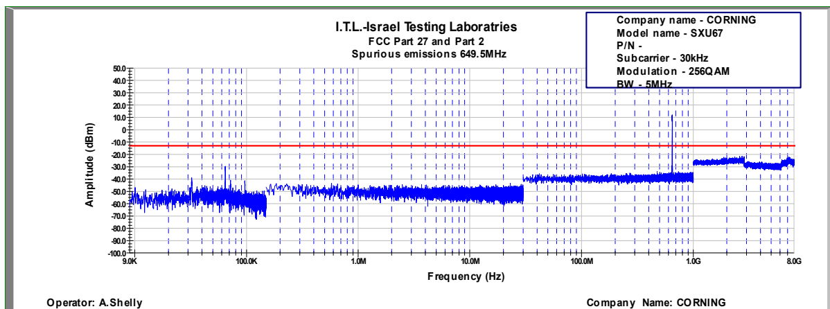
Figure 694: Spurious Emissions at Antenna Terminal 256QAM, 649.5MHz, B.W. 5MHz, Sub Carrier 30kHz
