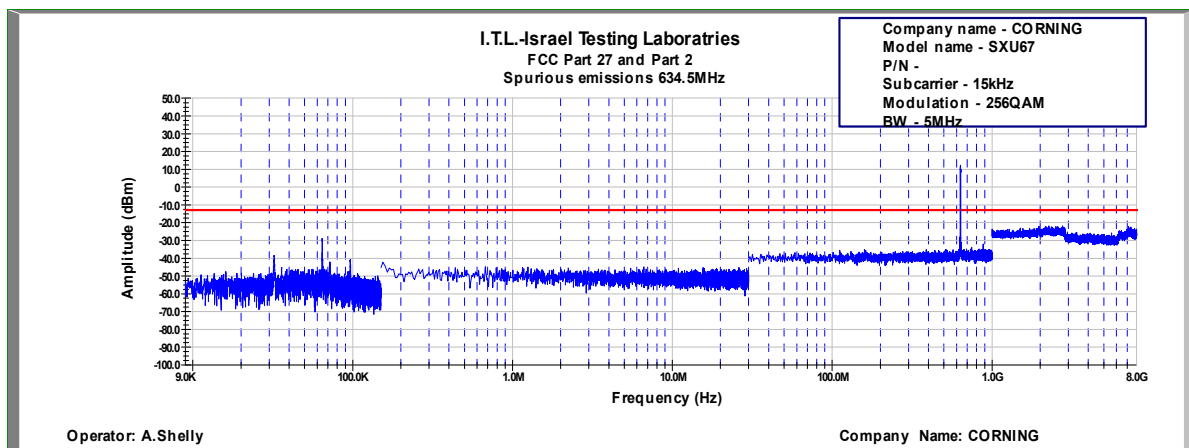
Figure 690: Spurious Emissions at Antenna Terminal 256QAM, 634.5MHz, B.W. 5MHz, Sub Carrier 15kHz
