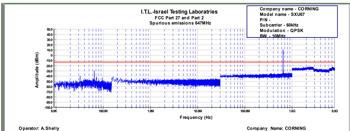
Figure 736: Spurious Emissions at Antenna Terminal QPSK, 647.0MHz, B.W. 10MHz, Sub Carrier 60kHz
