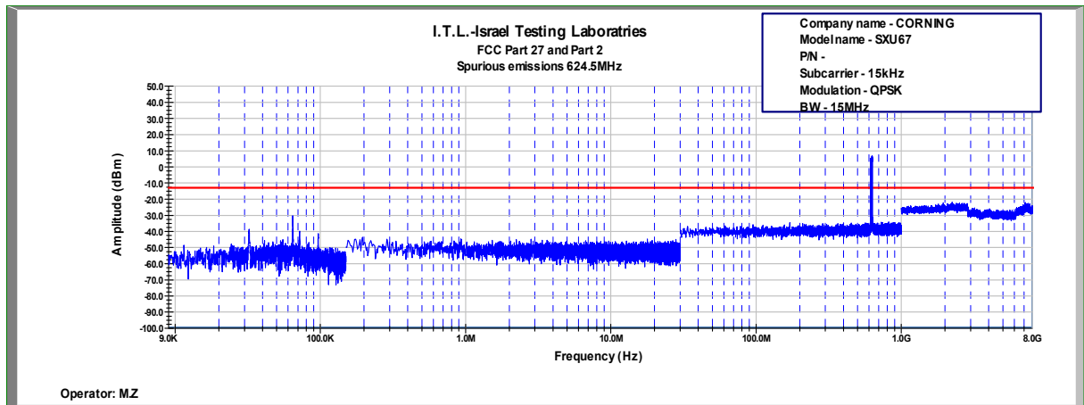
Figure 737: Spurious Emissions at Antenna Terminal QPSK, 624.5MHz, B.W. 15MHz, Sub Carrier 15kHz
