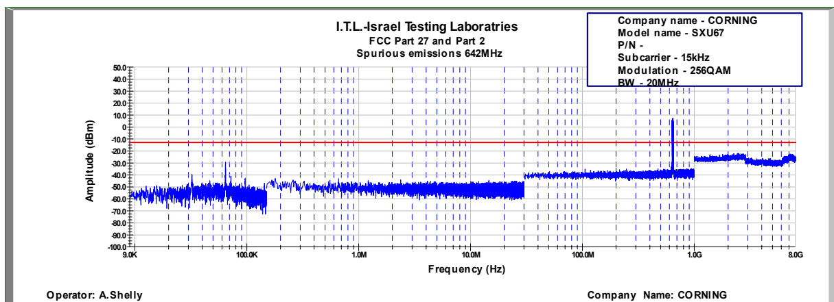
Figure 715: Spurious Emissions at Antenna Terminal 256QAM, 642.0MHz, B.W. 20MHz, Sub Carrier 15kHz
