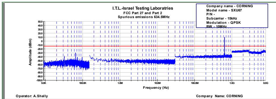
Figure 729: Spurious Emissions at Antenna Terminal QPSK, 634.5MHz, B.W. 10MHz, Sub Carrier 15kHz
