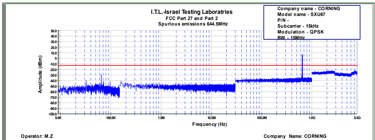
Figure 739: Spurious Emissions at Antenna Terminal QPSK, 644.5MHz, B.W. 15MHz, Sub Carrier 15kHz
