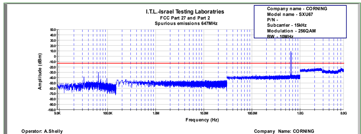
Figure 697: Spurious Emissions at Antenna Terminal 256QAM, 647.0MHz, B.W. 10MHz, Sub Carrier 15kHz
