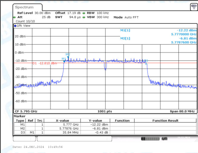
11AC40SISO-Ant1-5795-PASS
