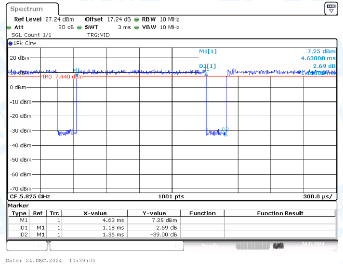
NTNV-11AC20SISO-Ant1-5825
