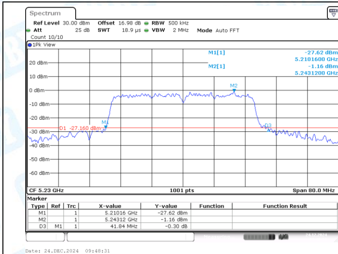
11AC40SISO-Ant1-5230
