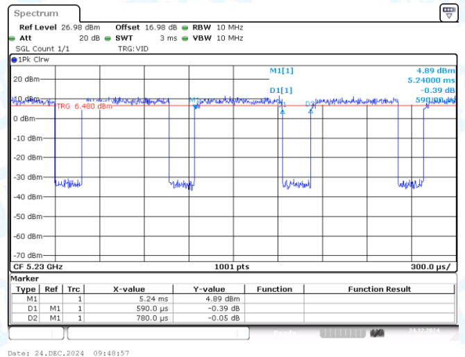
NTNV-11AC40SISO-Ant1-5230
