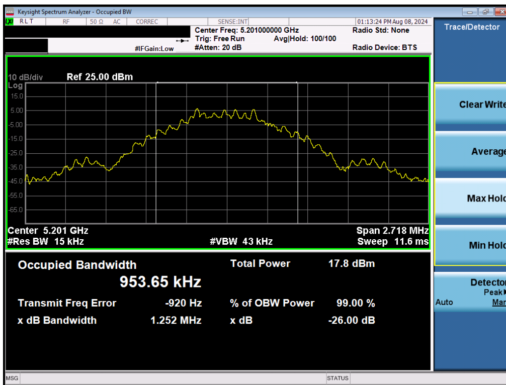
Plot 7-2. 26dB BW & 99% OBW (NB UNII BDR – 5201MHz)
