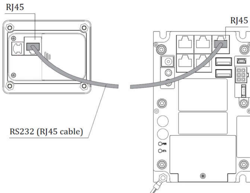
Figure 6: Connecting the IM700 to an IM300 unit
