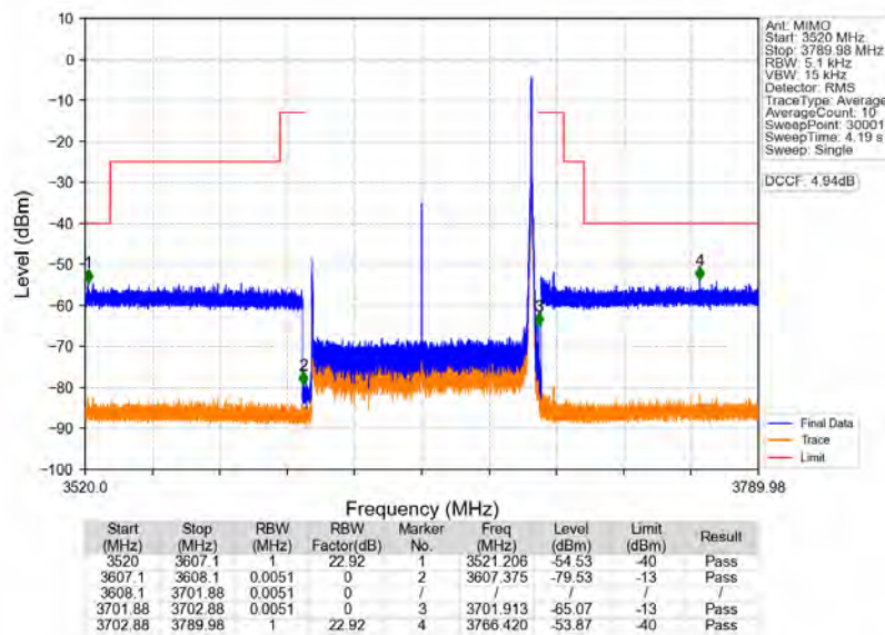
n78d_30kHz_MIMO_NTNV_90MHz_CP-OFDM_QPSK_3654.99MHz_Edge_1RB_Right
