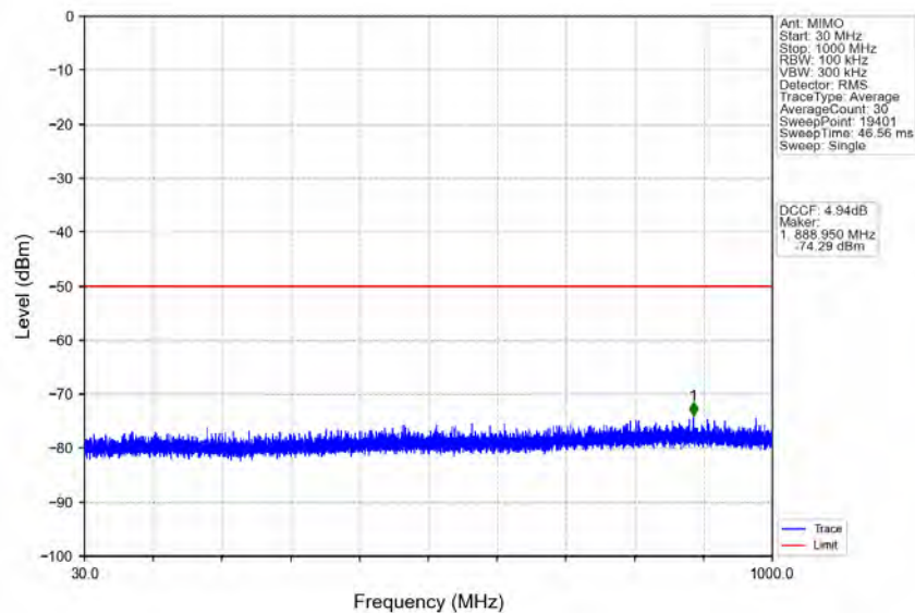
n78d_30kHz_MIMO_NTNV_90MHz_CP-OFDM QPSK_3654.99MHz_Edge_1RB_Right
