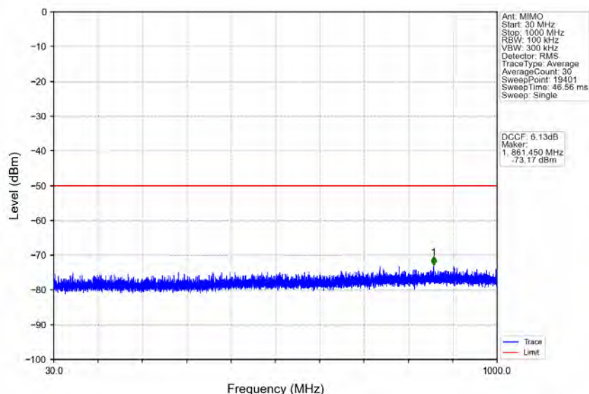
n78d_30kHz_MIMO_NTNV_90MHz_CP-OFDM_QPSK_3595.02MHz_Edge_1RB_Left
