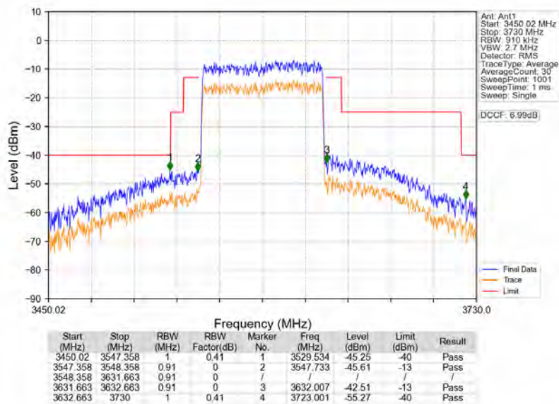
n78d_30kHz_MIMO_NTNV_80MHz_CP-OFDM_QPSK_3590.01MHz_Outer_Full
