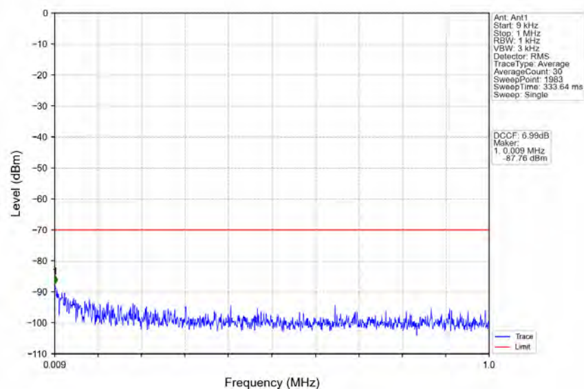
n78d 30kHz MIMO_NTNV_80MHz_CP-OFDM QPSK_3590.01MHz_Edge_1RB_Left
