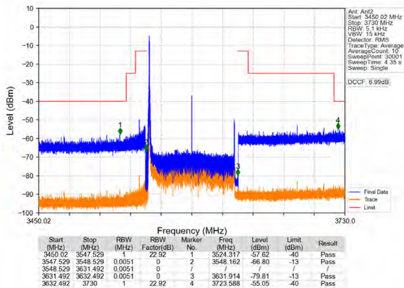
n78d_30kHz_MIMO_NTNV_80MHz_CP-OFDM_QPSK_3590.01MHz_Edge_1RB_Left
