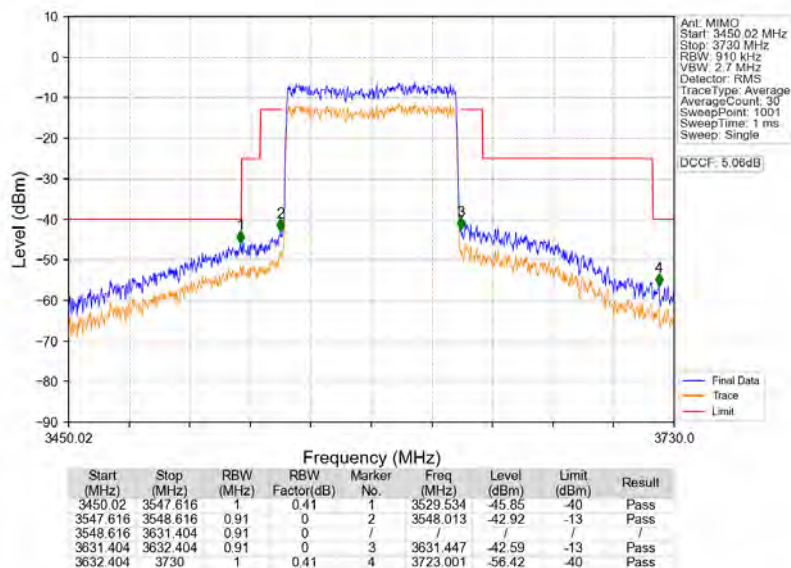
n78d_30kHz_MIMO_NTNV_80MHz_CP-OFDM_QPSK_3590.01MHz_Outer_Full
