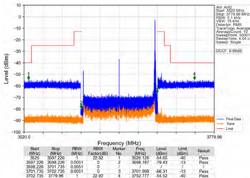
n78d_30kHz_MIMO_NTNV_100MHz_CP-OFDM_QPSK_3649.98MHz_Edge_1RB_Right
