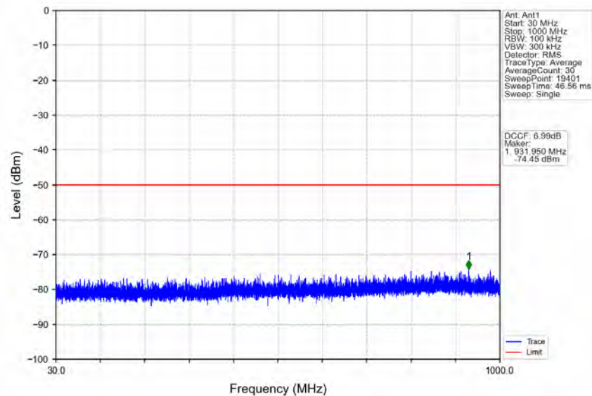
n78d_30kHz_MIMO_NTNV_80MHz_CP-OFDM_QPSK_3590.01MHz_Edge_1RB_Left
