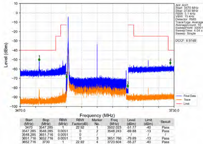
n78d_30kHz_MIMO_NTNV_100MHz_CP-OFDM_QPSK_3600MHz_Edge_1RB_Left
