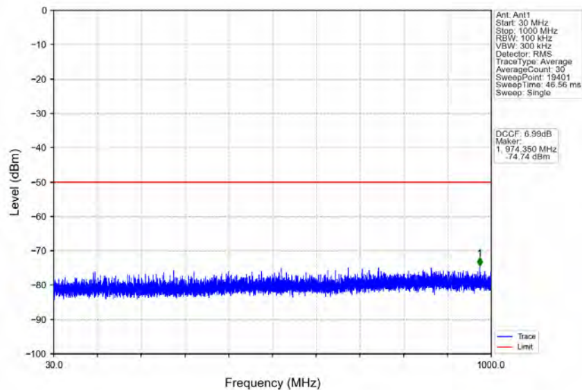
n78d_30kHz_MIMO_NTNV_80MHz_CP-OFDM_QPSK_3590.01MHz_Outer_Full
