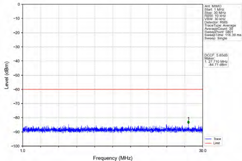
n78d_30kHz_MIMO_NTNV_70MHz_CP-OFDM QPSK_3664.98MHz_Inner_1RB_Right
