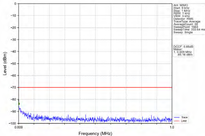
n78d_30kHz_MIMO_NTNV_100MHz_CP-OFDM_QPSK_3649.98MHz_Outer_Full
