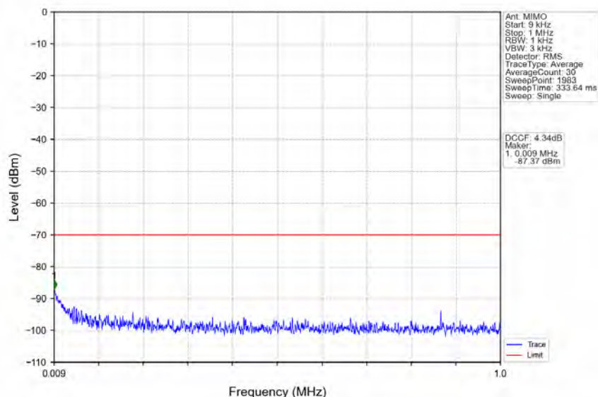
n78d_30kHz_MIMO_NTNV_90MHz_CP-OFDM_QPSK_3654.99MHz_Outer_Full
