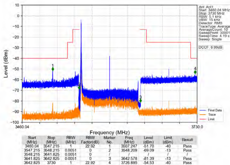
n78d 30kHz MIMO_NTNV_90MHz_CP-OFDM QPSK_3595.02MHz_Edge_1RB_Left
