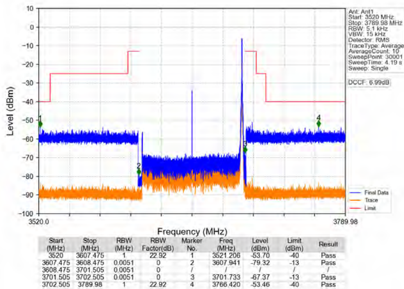
n78d_30kHz_MIMO_NTNV_90MHz_CP-OFDM_QPSK_3654.99MHz_Edge_1RB_Right
