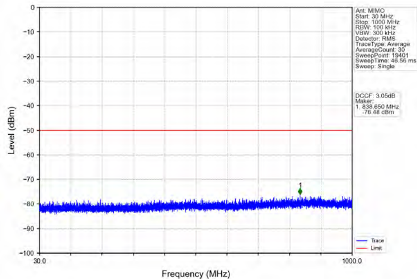
n78d_30kHz_MIMO_NTNV_90MHz_CP-OFDM QPSK_3654.99MHz_Inner_1RB_Right
