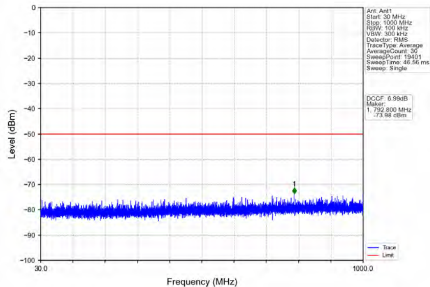
n78d_30kHz_MIMO_NTNV_100MHz_CP-OFDM QPSK_3600MHz_Outer_Full
