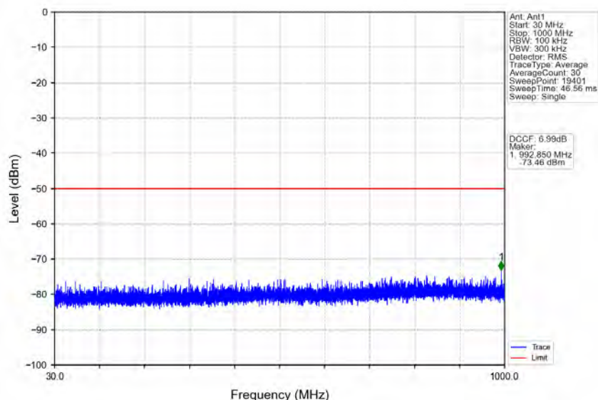
n78d_30kHz_MIMO_NTNV_80MHz_CP-OFDM_QPSK_3590.01MHz_Inner_1RB_Left
