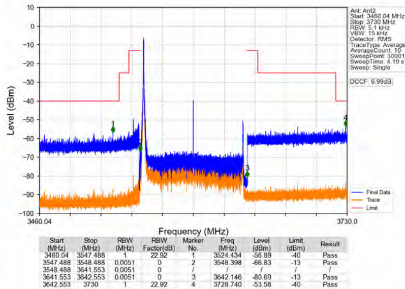
n78d_30kHz_MIMO_NTNV_90MHz_CP-OFDM_QPSK_3595.02MHz_Inner_1RB_Left
