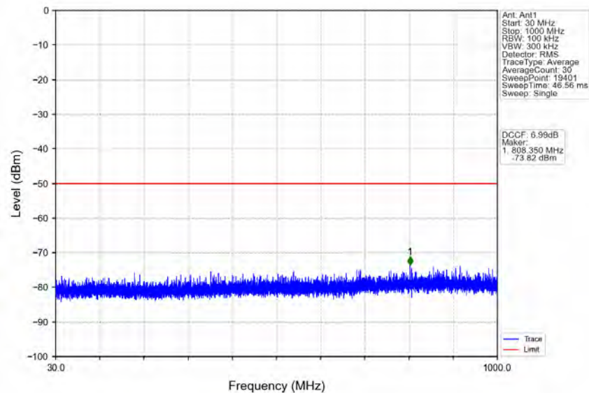
n78d_30kHz_MIMO_NTNV_90MHz_CP-OFDM QPSK_3654.99MHz_Edge_1RB_Right
