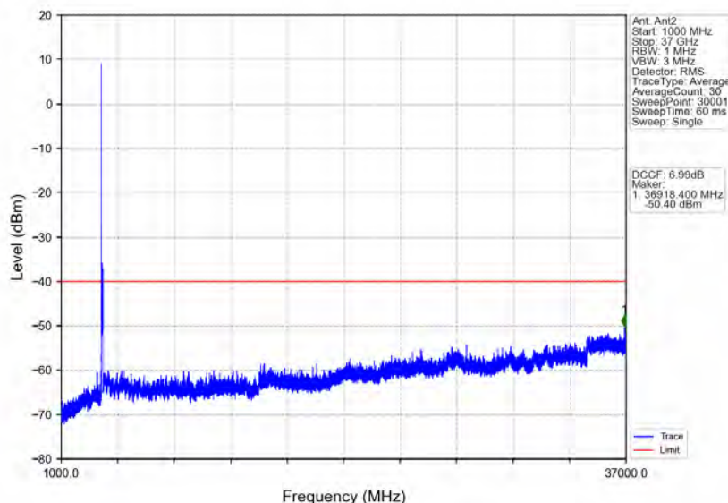
n78d_30kHz_MIMO_NTNV_100MHz_CP-OFDM_QPSK_3600MHz_Inner_1RB_Left
