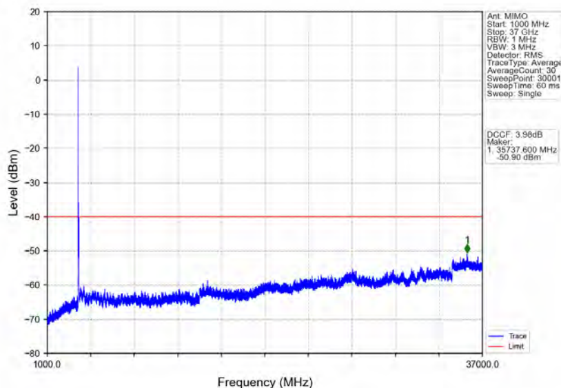
n78d_30kHz_MIMO_NTNV_80MHz_CP-OFDM_QPSK_3590.01MHz_Outer_Full
