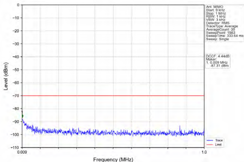
n78d_30kHz_MIMO_NTNV_100MHz_CP-OFDM QPSK_3600MHz_Outer_Full
