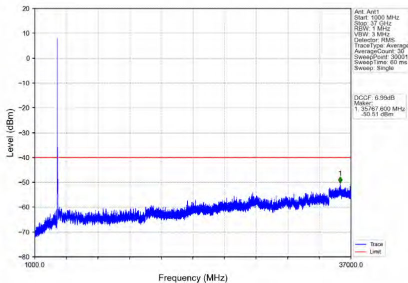
n78d_30kHz_MIMO_NTNV_90MHz_CP-OFDM_QPSK_3595.02MHz_Inner_1RB_Left
