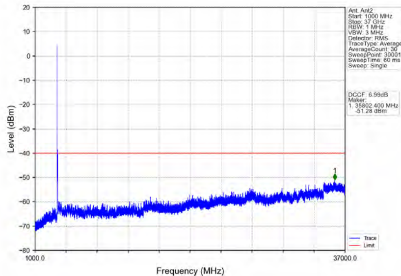
n78d_30kHz_MIMO_NTNV_80MHz_CP-OFDM_QPSK_3590.01MHz_Inner_1RB_Left
