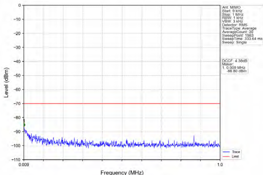
n78d_30kHz_MIMO_NTNV_90MHz_CP-OFDM_QPSK_3595.02MHz_Inner_1RB_Left
