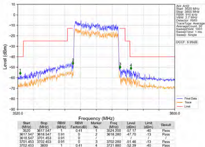
n78d_30kHz_MIMO_NTNV_80MHz_CP-OFDM_QPSK_3660MHz_Outer_Full
