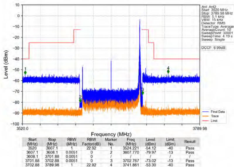
n78d_30kHz_MIMO_NTNV_90MHz_CP-OFDM_QPSK_3654.99MHz_Inner_1RB_Right
