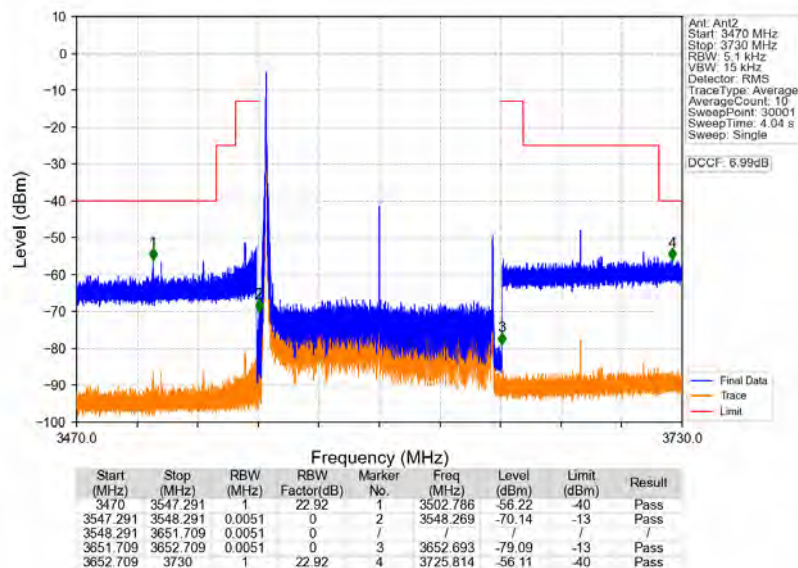
n78d_30kHz_MIMO_NTNV_100MHz_CP-OFDM_QPSK_3600MHz_Inner_1RB_Left
