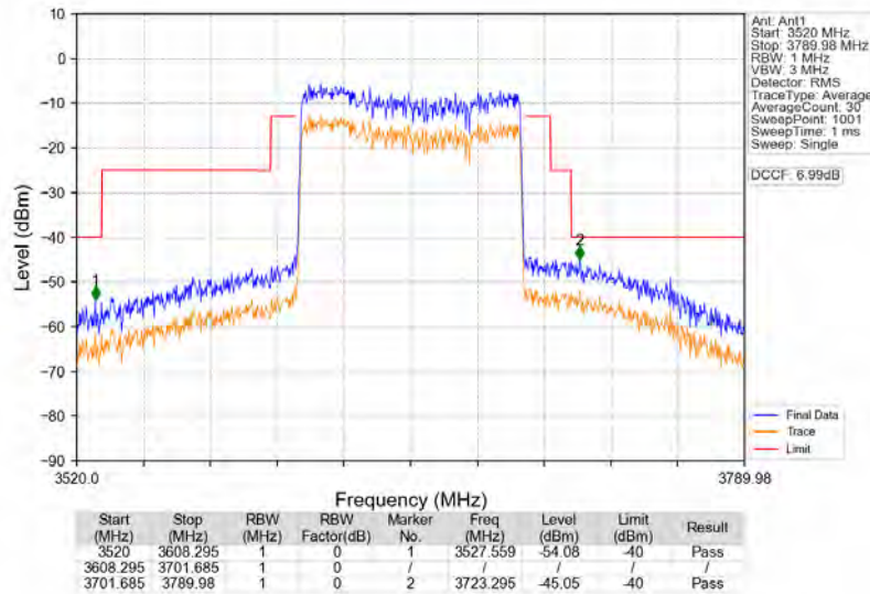
n78d_30kHz_MIMO_NTNV_90MHz_CP-OFDM_QPSK_3654.99MHz_Outer_Full
