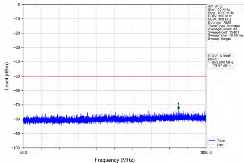
n78d_30kHz_MIMO_NTNV_90MHz_CP-OFDM_QPSK_3595.02MHz_Inner_1RB_Left
