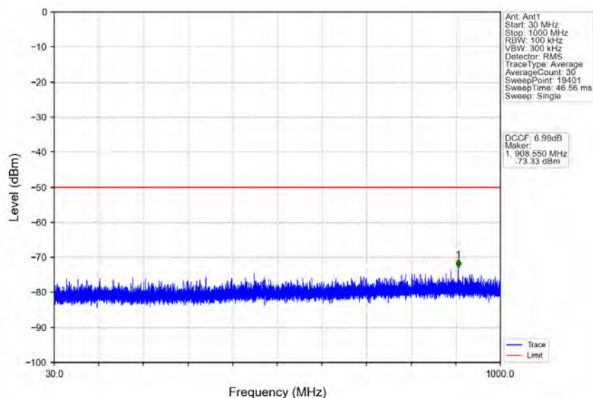
n78d_30kHz_MIMO_NTNV_100MHz_CP-OFDM_QPSK_3649.98MHz_Inner_1RB_Right
