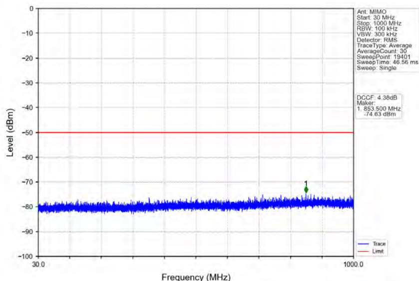
n78d_30kHz_MIMO_NTNV_90MHz_CP-OFDM_QPSK_3595.02MHz_Inner_1RB_Left
