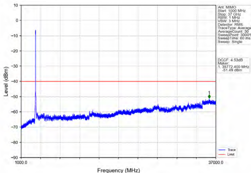
n78d_30kHz_MIMO_NTNV_80MHz_CP-OFDM_QPSK_3660MHz_Inner_1RB_Right
