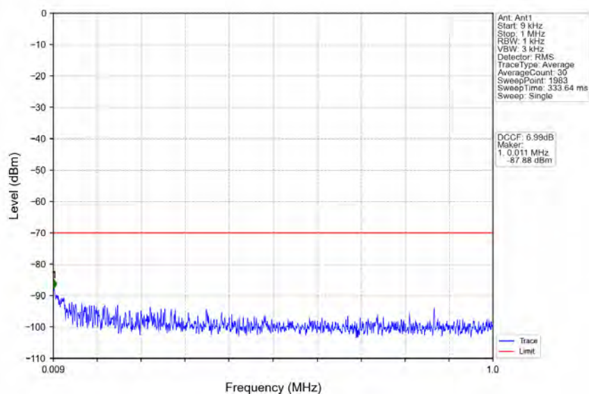
n78d 30kHz MIMO_NTNV_90MHz_CP-OFDM QPSK_3595.02MHz_Edge_1RB_Left
