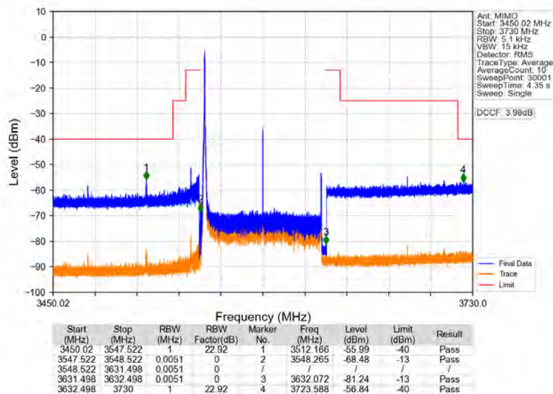
n78d_30kHz_MIMO_NTNV_80MHz_CP-OFDM_QPSK_3590.01MHz_Edge_1RB_Left
