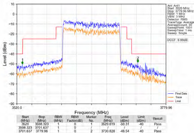
n78d_30kHz_MIMO_NTNV_100MHz_CP-OFDM_QPSK_3649.98MHz_Outer_Full
