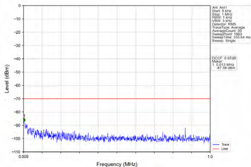
n78d_30kHz_MIMO_NTNV_100MHz_CP-OFDM_QPSK_3600MHz_Edge_1RB_Left
