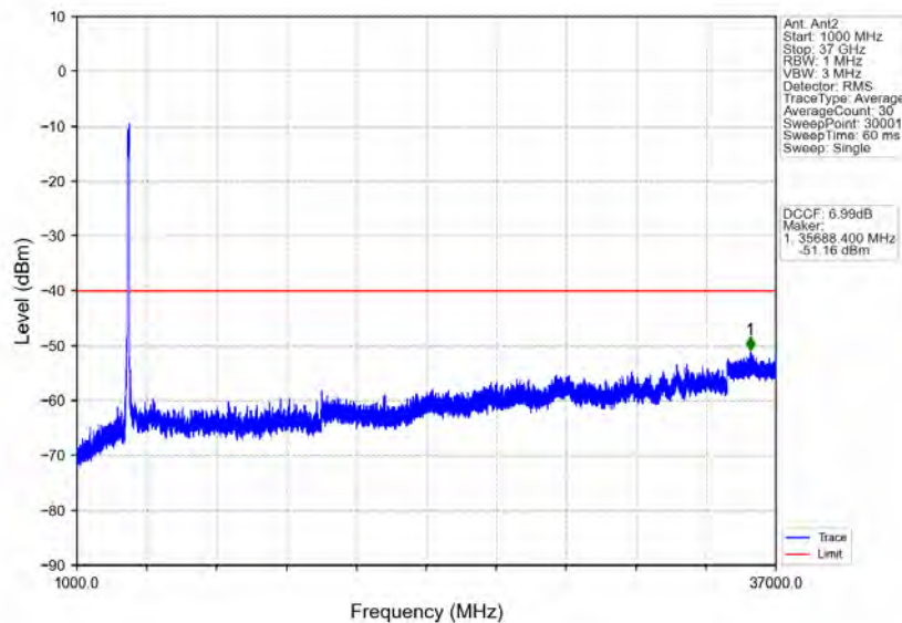
n78d_30kHz_MIMO_NTNV_100MHz_CP-OFDM QPSK_3649.98MHz_Outer_Full
