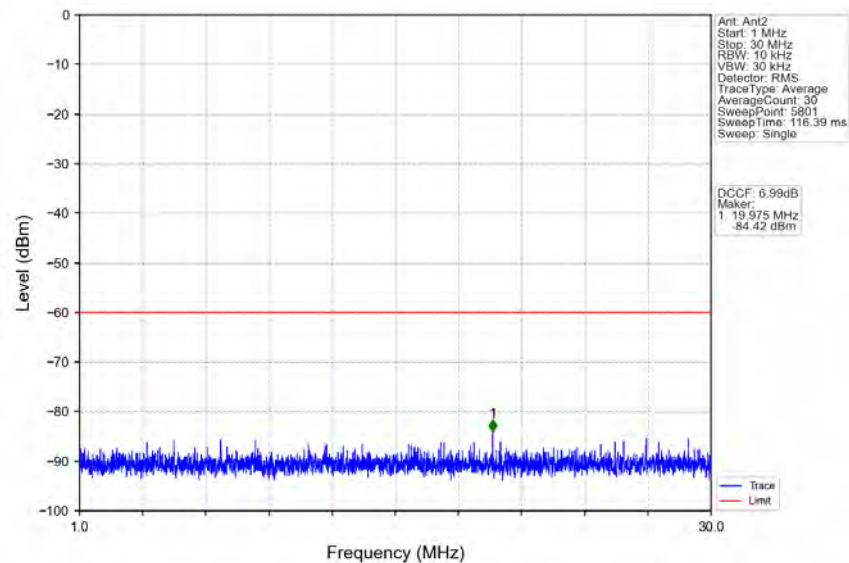
n78d_30kHz_MIMO_NTNV_80MHz_CP-OFDM_QPSK_3660MHz_Outer_Full
