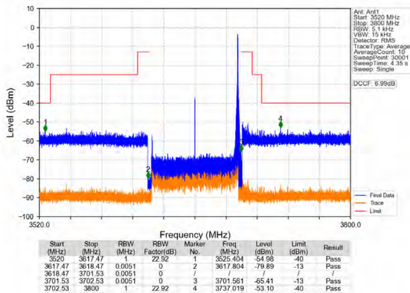
n78d_30kHz_MIMO_NTNV_80MHz_CP-OFDM_QPSK_3660MHz_Inner_1RB_Right
