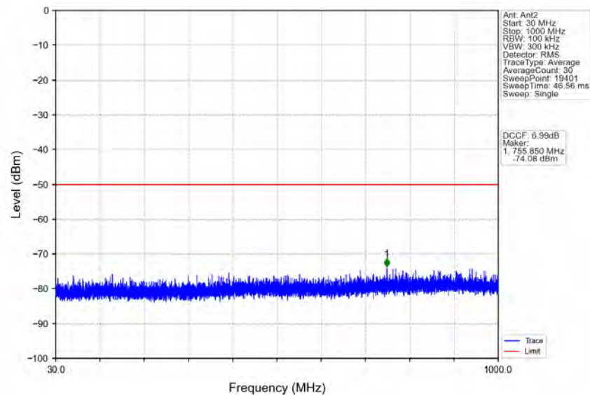
n78d_30kHz_MIMO_NTNV_80MHz_CP-OFDM_QPSK_3590.01MHz_Inner_1RB_Left
