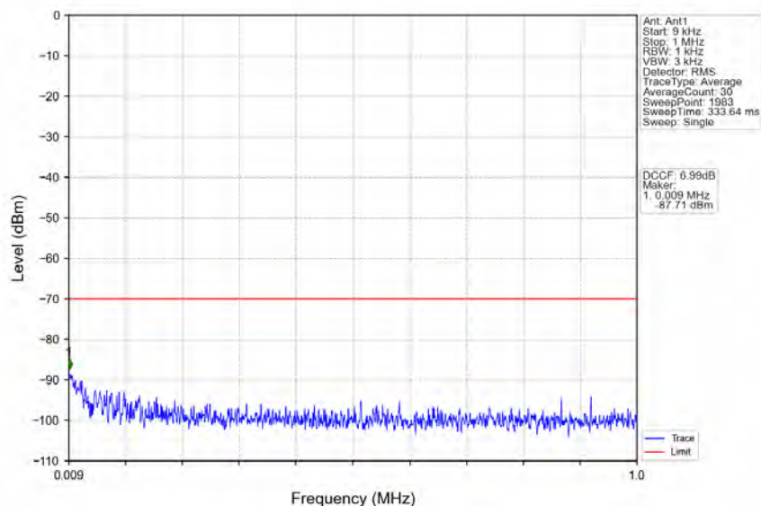
n78d_30kHz_MIMO_NTNV_80MHz_CP-OFDM_QPSK_3660MHz_Inner_1RB_Right
