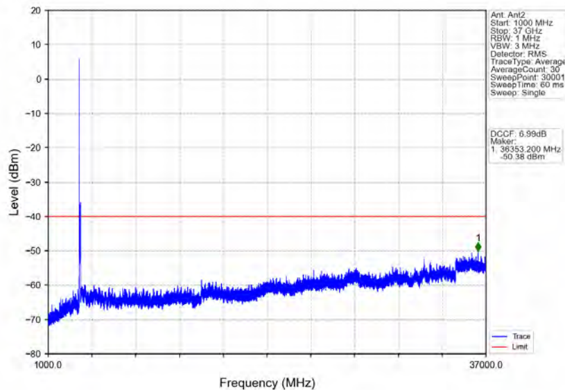
n78d_30kHz_MIMO_NTNV_100MHz_CP-OFDM_QPSK_3600MHz_Edge_1RB_Left
