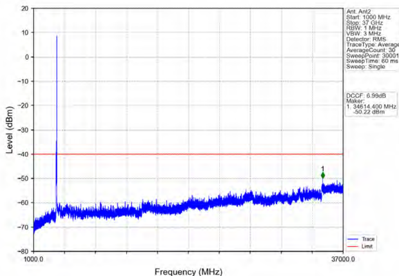
n78d_30kHz_MIMO_NTNV_100MHz_CP-OFDM_QPSK_3649.98MHz_Edge_1RB_Right
