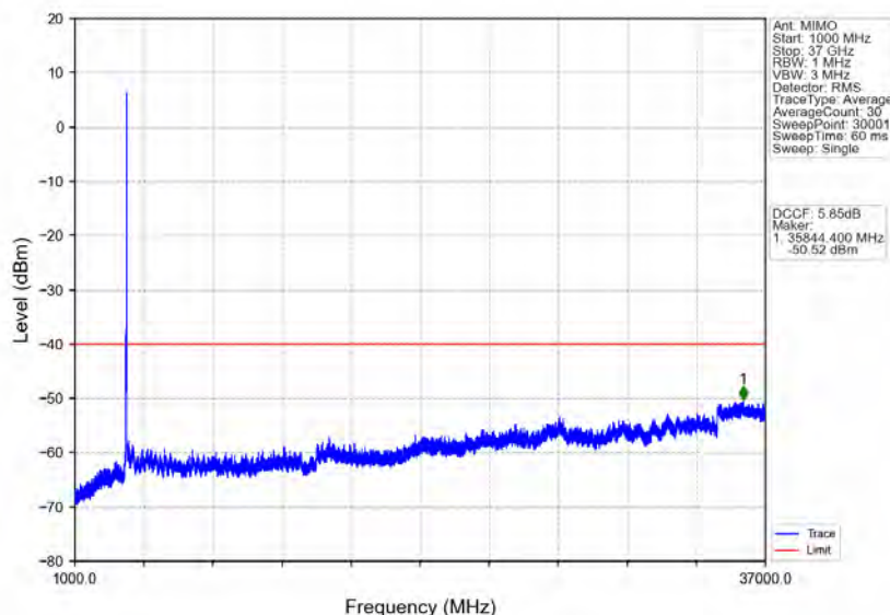
n78d_30kHz_MIMO_NTNV_70MHz_CP-OFDM QPSK_3664.98MHz_Inner_1RB_Right
