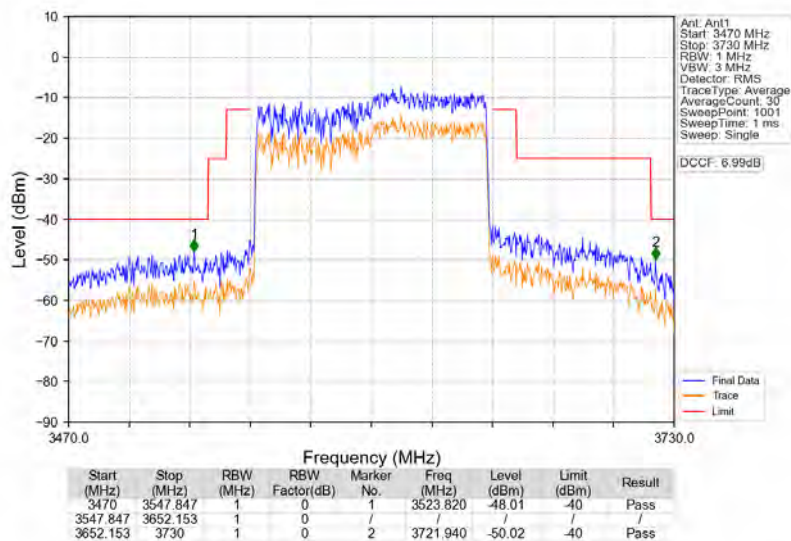
n78d_30kHz_MIMO_NTNV_100MHz_CP-OFDM_QPSK_3600MHz_Outer_Full
