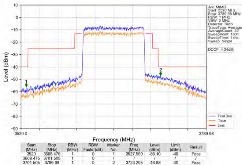
n78d_30kHz_MIMO_NTNV_90MHz_CP-OFDM_QPSK_3654.99MHz_Outer_Full
