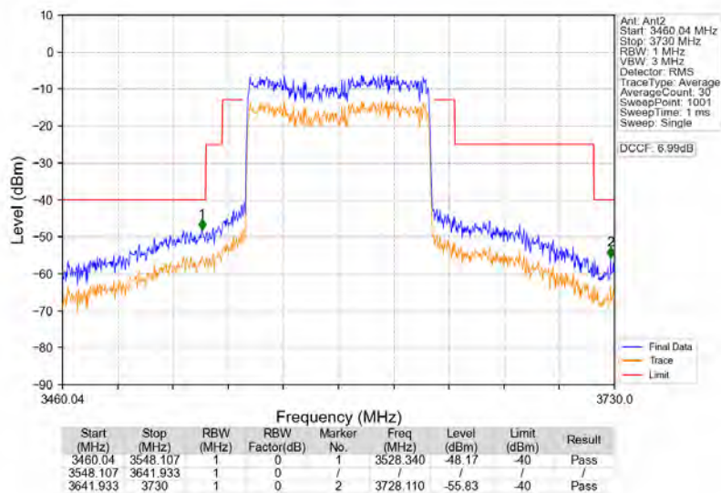
n78d_30kHz_MIMO_NTNV_90MHz_CP-OFDM_QPSK_3595.02MHz_Outer_Full
