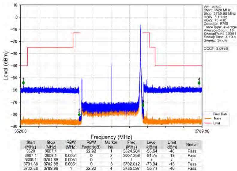
n78d_30kHz_MIMO_NTNV_90MHz_CP-OFDM_QPSK_3654.99MHz_Inner_1RB_Right
