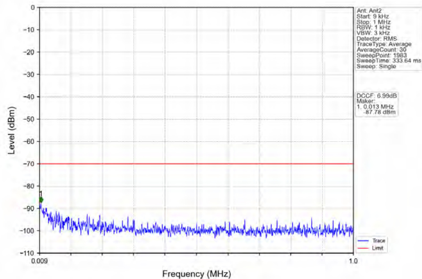
n78d_30kHz_MIMO_NTNV_80MHz_CP-OFDM_QPSK_3590.01MHz_Inner_1RB_Left
