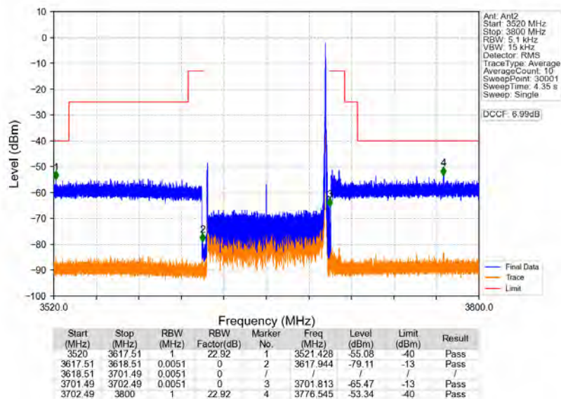
n78d_30kHz_MIMO_NTNV_80MHz_CP-OFDM_QPSK_3660MHz_Edge_1RB_Right
