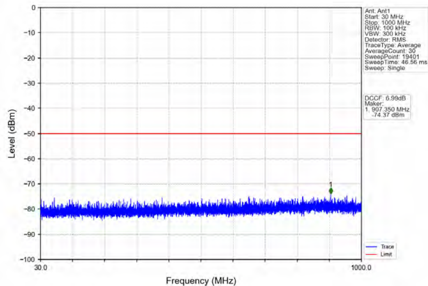
n78d_30kHz_MIMO_NTNV_90MHz_CP-OFDM_QPSK_3595.02MHz_Edge_1RB_Left
