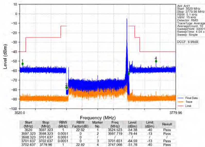
n78d_30kHz_MIMO_NTNV_100MHz_CP-OFDM QPSK_3649.98MHz_Inner_1RB_Right
