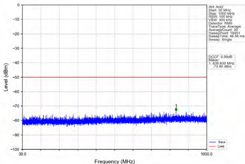
n78d_30kHz_MIMO_NTNV_100MHz_CP-OFDM_QPSK_3600MHz_Inner_1RB_Left
