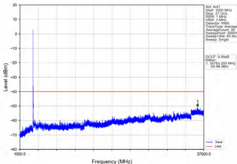
n78d_30kHz_MIMO_NTNV_90MHz_CP-OFDM_QPSK_3595.02MHz_Edge_1RB_Left
