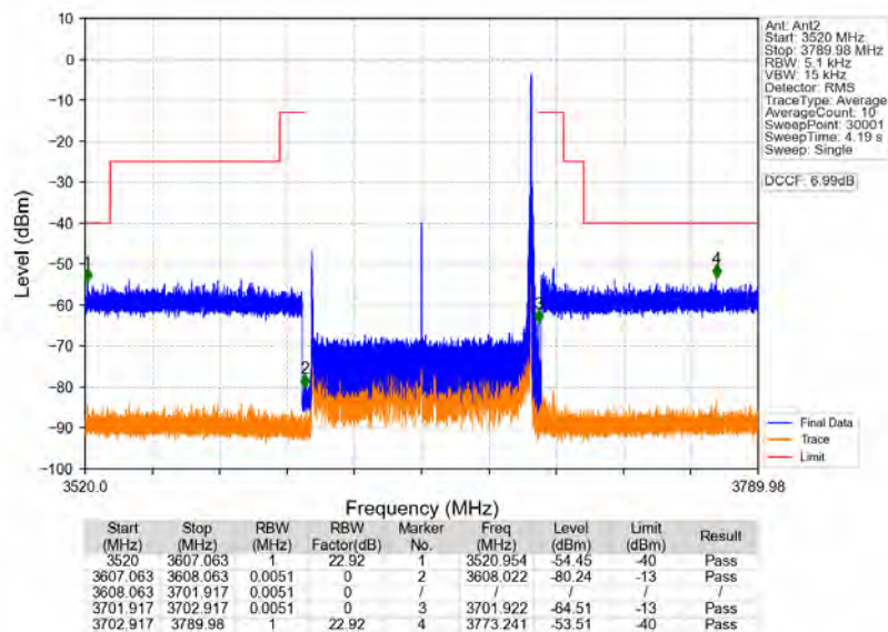
n78d_30kHz_MIMO_NTNV_90MHz_CP-OFDM_QPSK_3654.99MHz_Edge_1RB_Right
