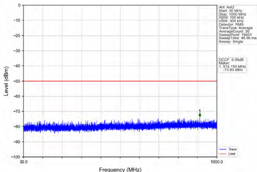
n78d_30kHz_MIMO_NTNV_80MHz_CP-OFDM_QPSK_3660MHz_Inner_1RB_Right
