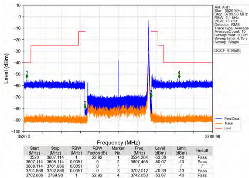
n78d_30kHz_MIMO_NTNV_90MHz_CP-OFDM_QPSK_3654.99MHz_Inner_1RB_Right
