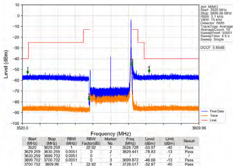
n78d_30kHz_MIMO_NTNV_70MHz_CP-OFDM_QPSK_3664.98MHz_Inner_1RB_Right
