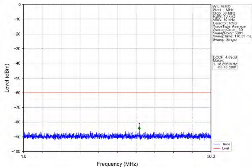
n78d_30kHz_MIMO_NTNV_100MHz_CP-OFDM_QPSK_3649.98MHz_Inner_1RB_Right
