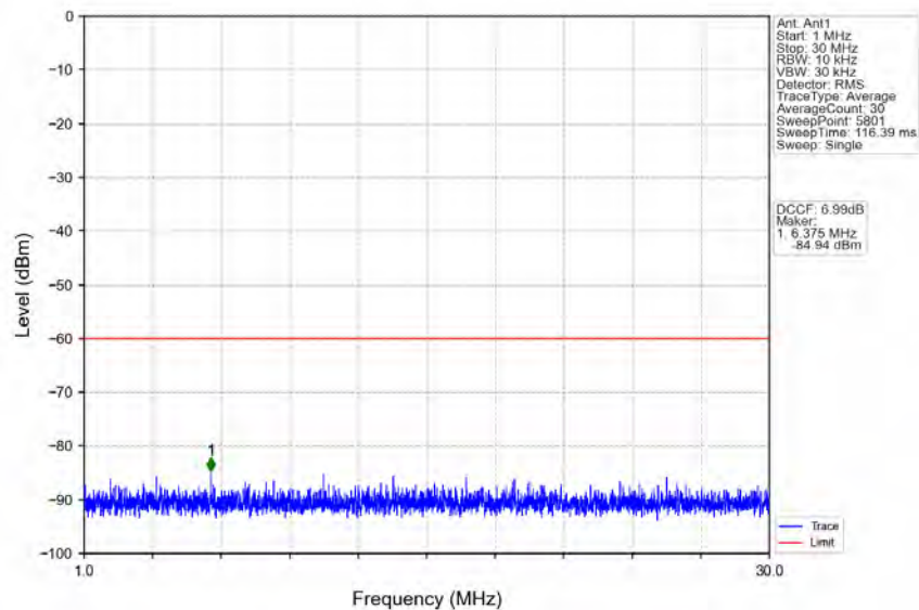
n78d_30kHz_MIMO_NTNV_80MHz_CP-OFDM QPSK_3660MHz_Edge_1RB_Right
