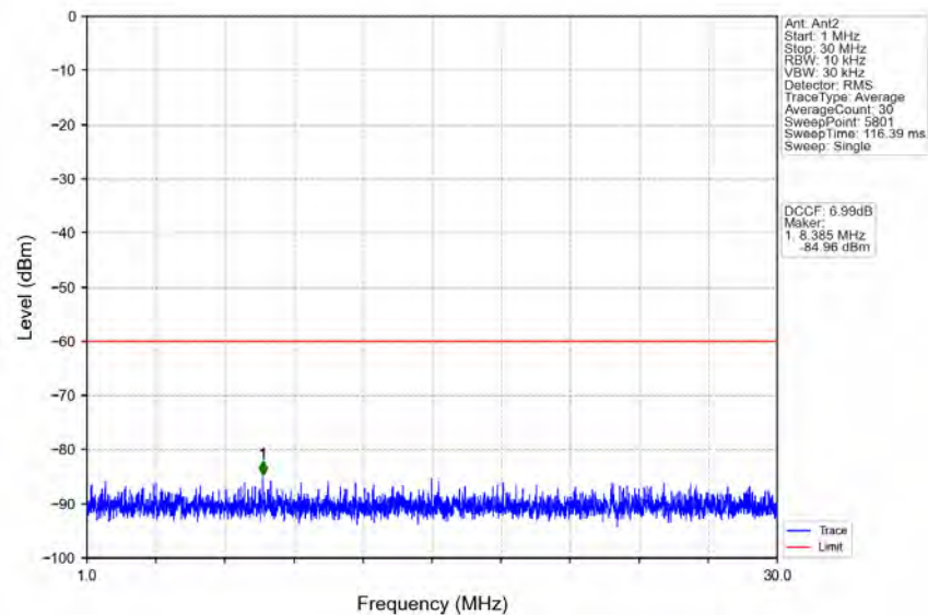
n78d_30kHz_MIMO_NTNV_100MHz_CP-OFDM_QPSK_3600MHz_Edge_1RB_Left
