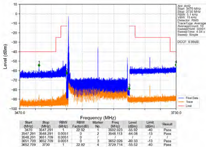
n78d_30kHz_MIMO_NTNV_100MHz_CP-OFDM_QPSK_3600MHz_Edge_1RB_Left
