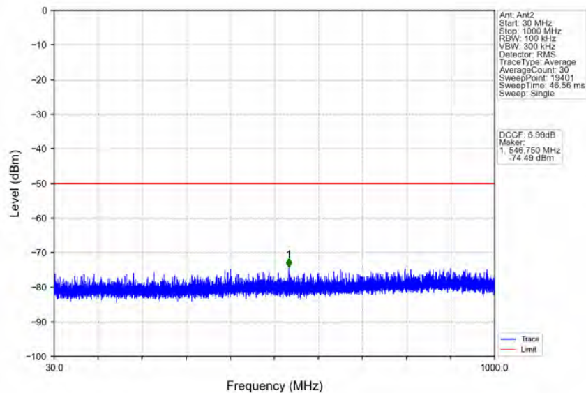
n78d_30kHz_MIMO_NTNV_90MHz_CP-OFDM_QPSK_3654.99MHz_Outer_Full
