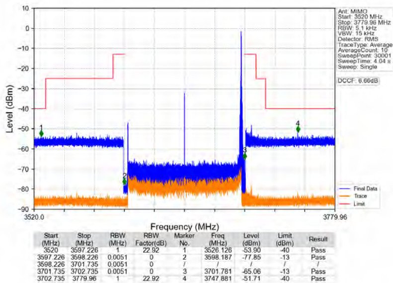
n78d_30kHz_MIMO_NTNV_100MHz_CP-OFDM_QPSK_3649.98MHz_Edge_1RB_Right
