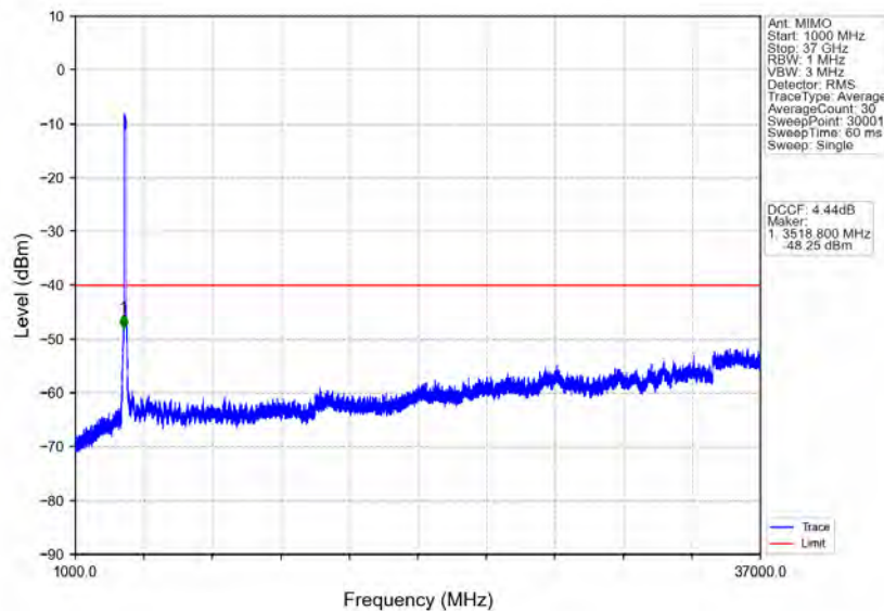
n78d_30kHz_MIMO_NTNV_100MHz_CP-OFDM QPSK_3600MHz_Outer_Full
