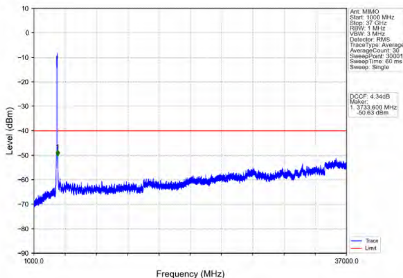
n78d_30kHz_MIMO_NTNV_90MHz_CP-OFDM_QPSK_3654.99MHz_Inner_1RB_Right
