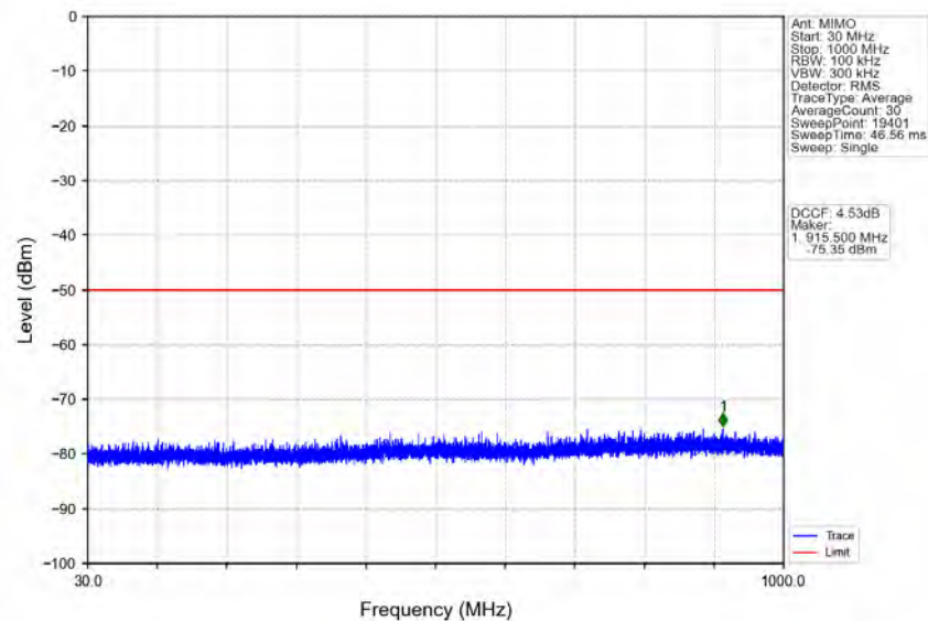
n78d_30kHz_MIMO_NTNV_80MHz_CP-OFDM_QPSK_3660MHz_Outer_Full
