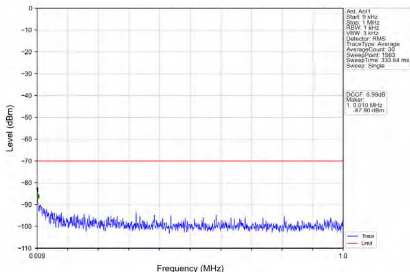
n78d_30kHz_MIMO_NTNV_100MHz_CP-OFDM_QPSK_3649.98MHz_Outer_Full
