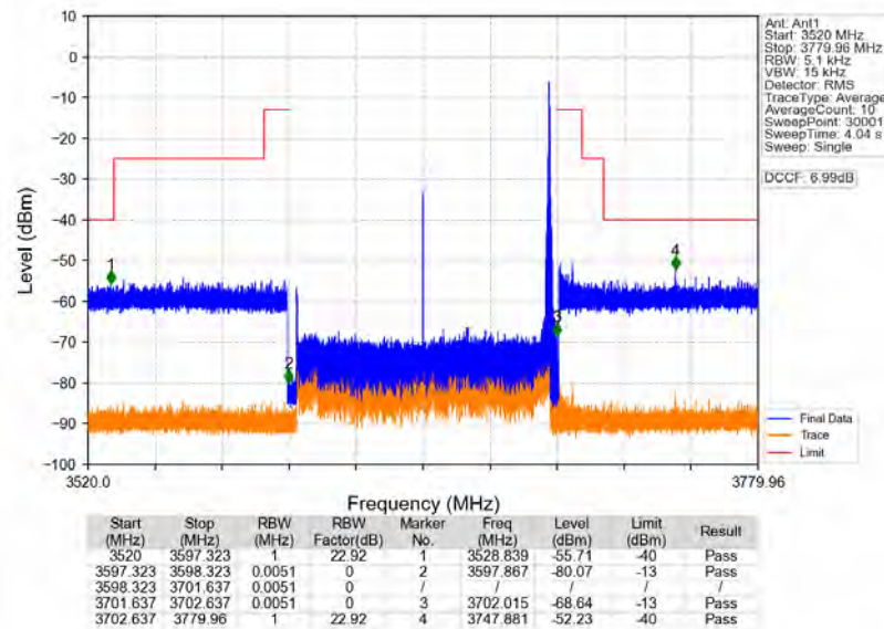
n78d_30kHz_MIMO_NTNV_100MHz_CP-OFDM_QPSK_3649.98MHz_Edge_1RB_Right
