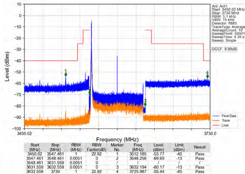
n78d 30kHz MIMO_NTNV_80MHz_CP-OFDM QPSK_3590.01MHz_Edge_1RB_Left
