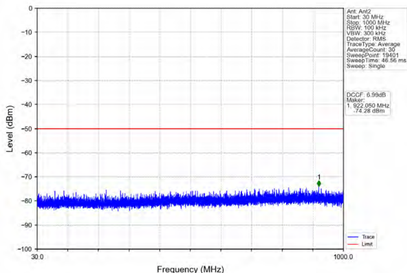
n78d_30kHz_MIMO_NTNV_100MHz_CP-OFDM_QPSK_3649.98MHz_Edge_1RB_Right
