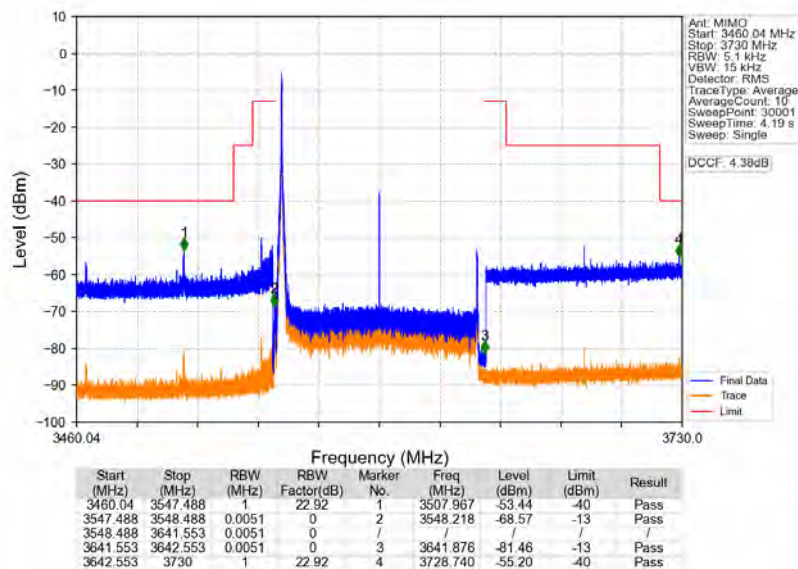
n78d_30kHz_MIMO_NTNV_90MHz_CP-OFDM_QPSK_3595.02MHz_Inner_1RB_Left
