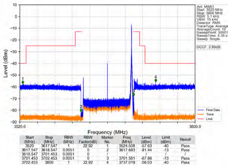
n78d_30kHz_MIMO_NTNV_80MHz_CP-OFDM_QPSK_3660MHz_Inner_1RB_Right
