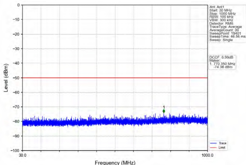
n78d_30kHz_MIMO_NTNV_80MHz_CP-OFDM_QPSK_3660MHz_Outer_Full
