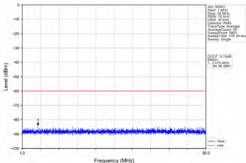
n78d_30kHz_MIMO_NTNV_90MHz_CP-OFDM_QPSK_3595.02MHz_Edge_1RB_Left
