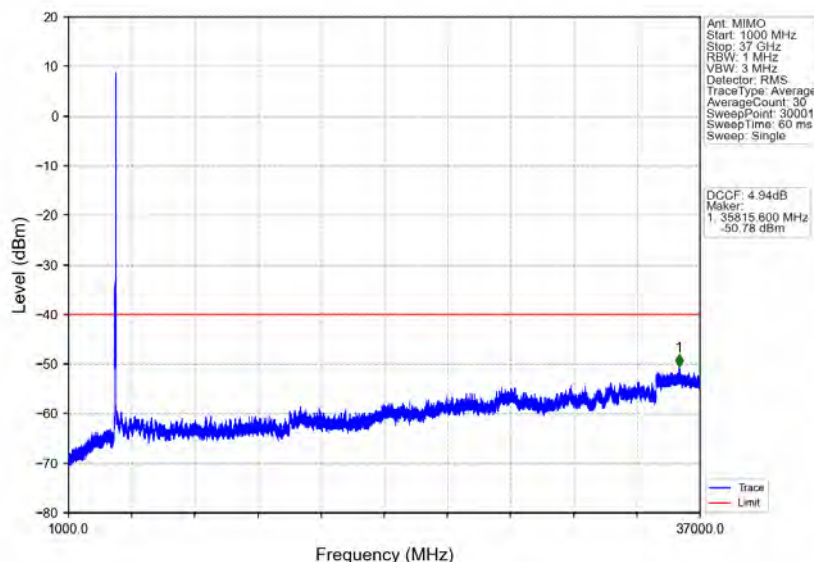
n78d_30kHz_MIMO_NTNV_80MHz_CP-OFDM QPSK_3660MHz_Edge_1RB_Right
