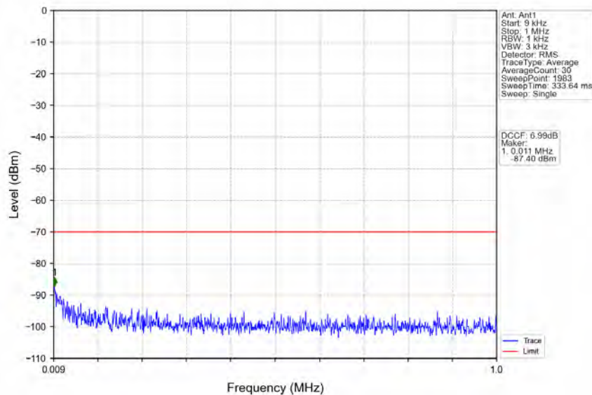
n78d_30kHz_MIMO_NTNV_90MHz_CP-OFDM_QPSK_3654.99MHz_Outer_Full
