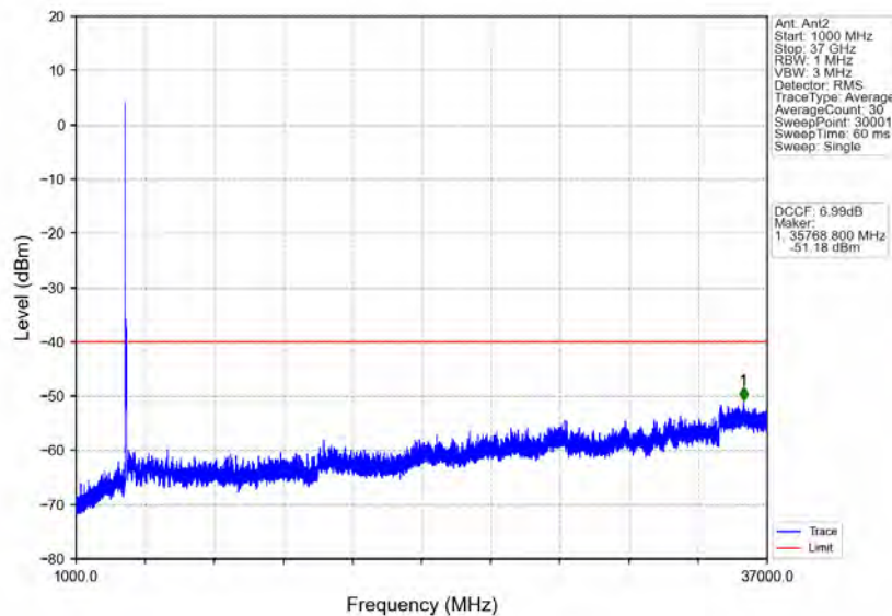
n78d_30kHz_MIMO_NTNV_80MHz_CP-OFDM_QPSK_3590.01MHz_Edge_1RB_Left
