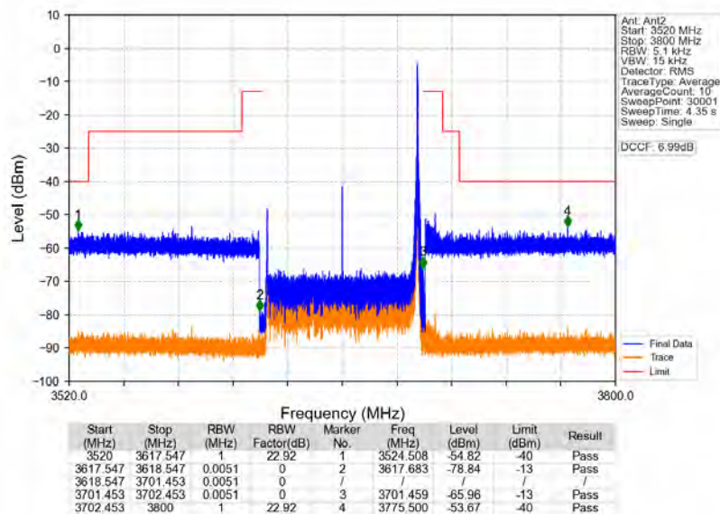
n78d_30kHz_MIMO_NTNV_80MHz_CP-OFDM_QPSK_3660MHz_Inner_1RB_Right
