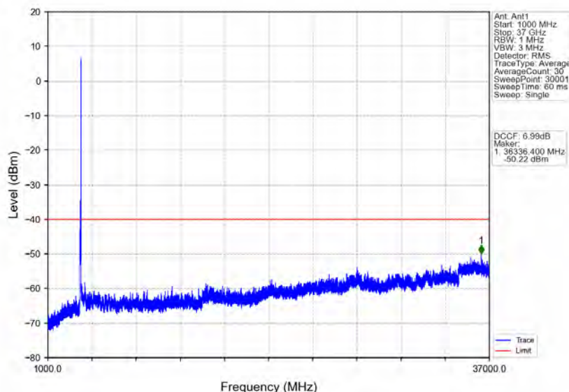
n78d_30kHz_MIMO_NTNV_100MHz_CP-OFDM_QPSK_3649.98MHz_Inner_1RB_Right
