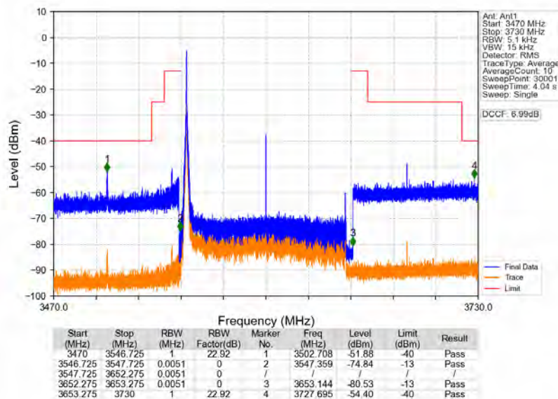
n78d_30kHz_MIMO_NTNV_100MHz_CP-OFDM_QPSK_3600MHz_Inner_1RB_Left
