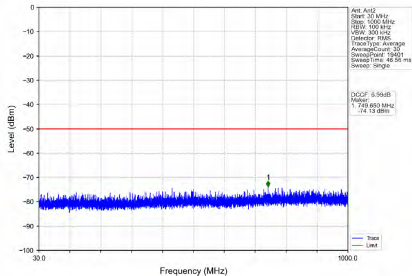
n78d_30kHz_MIMO_NTNV_100MHz_CP-OFDM_QPSK_3600MHz_Edge_1RB_Left
