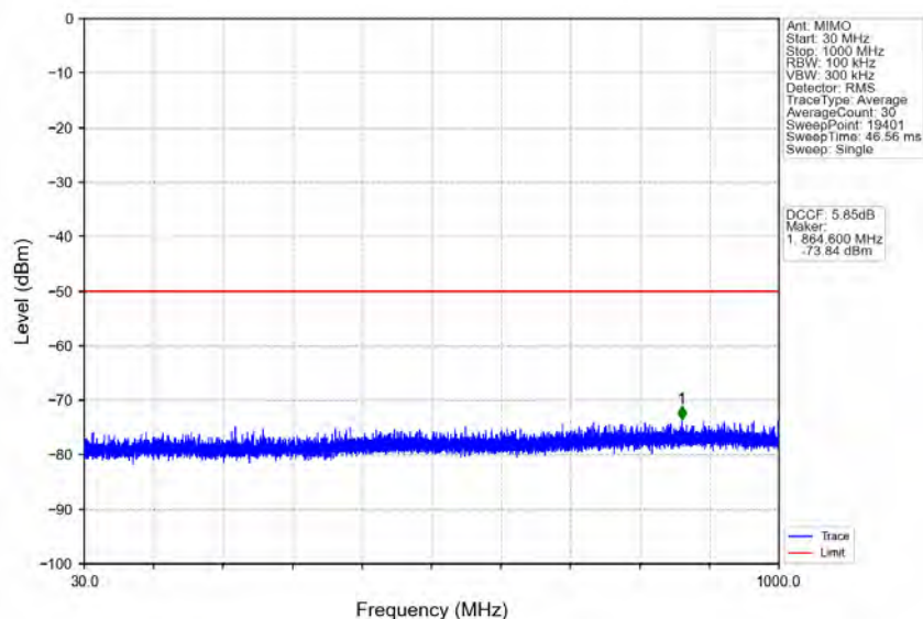
n78d_30kHz_MIMO_NTNV_70MHz_CP-OFDM QPSK_3664.98MHz_Inner_1RB_Right
