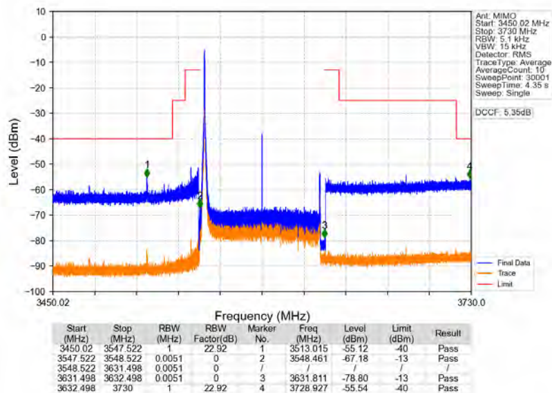
n78d_30kHz_MIMO_NTNV_80MHz_CP-OFDM_QPSK_3590.01MHz_Inner_1RB_Left
