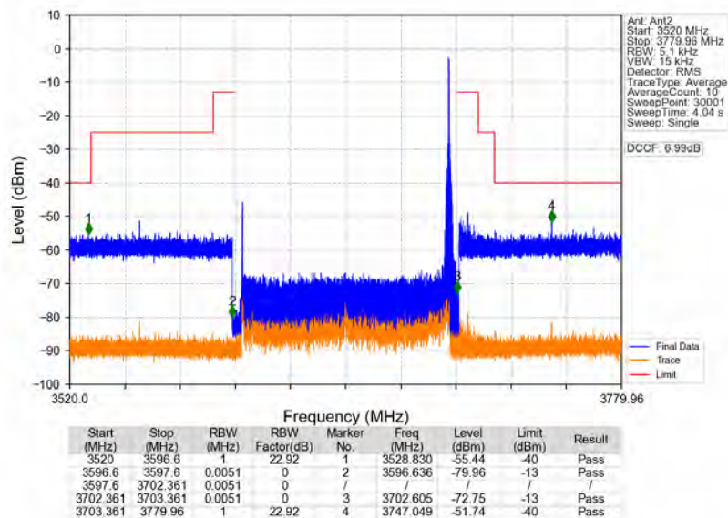
n78d_30kHz_MIMO_NTNV_100MHz_CP-OFDM_QPSK_3649.98MHz_Inner_1RB_Right
