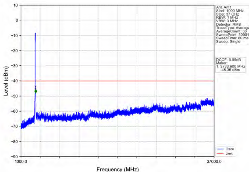
n78d_30kHz_MIMO_NTNV_90MHz_CP-OFDM_QPSK_3654.99MHz_Outer_Full
