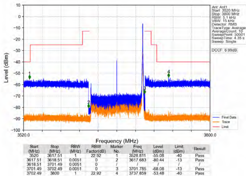
n78d_30kHz_MIMO_NTNV_80MHz_CP-OFDM_QPSK_3660MHz_Edge_1RB_Right
