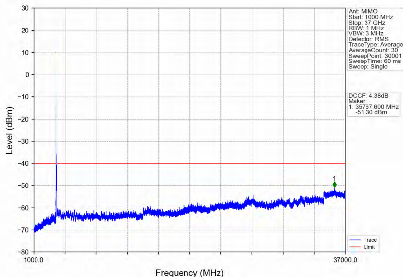
n78d_30kHz_MIMO_NTNV_90MHz_CP-OFDM_QPSK_3654.99MHz_Edge_1RB_Right
