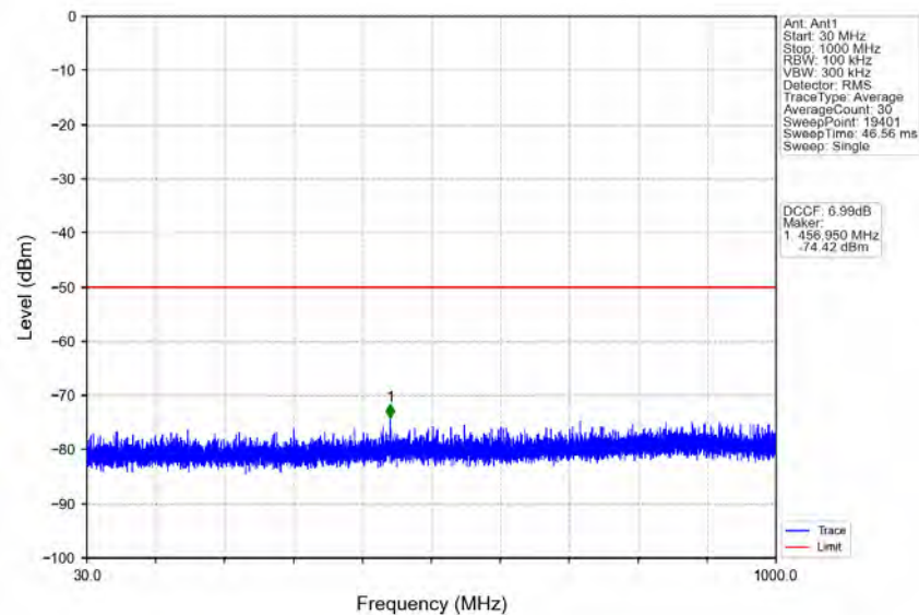
n78d_30kHz_MIMO_NTNV_80MHz_CP-OFDM QPSK_3660MHz_Edge_1RB_Right
