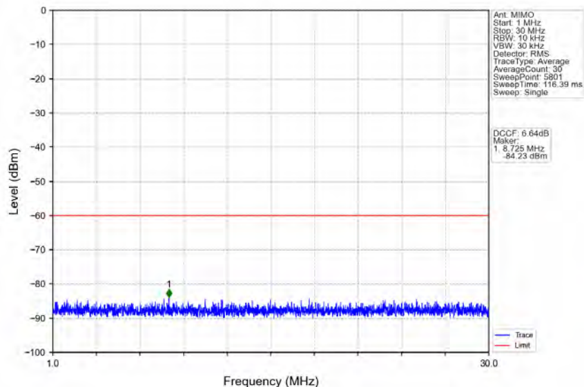
n78d_30kHz_MIMO_NTNV_100MHz_CP-OFDM_QPSK_3600MHz_Edge_1RB_Left
