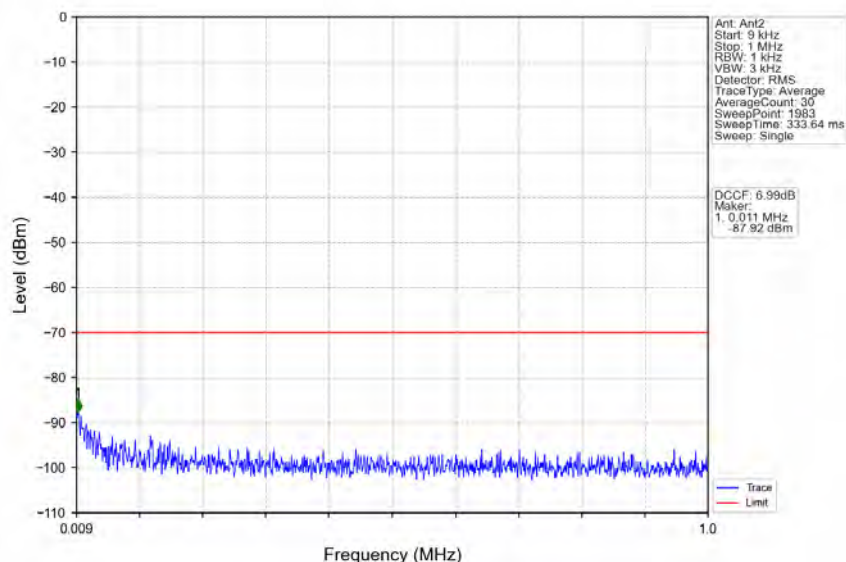
n78d_30kHz_MIMO_NTNV_90MHz_CP-OFDM_QPSK_3595.02MHz_Outer_Full
