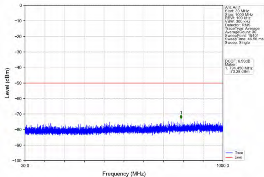
n78d_30kHz_MIMO_NTNV_100MHz_CP-OFDM_QPSK_3649.98MHz_Edge_1RB_Right
