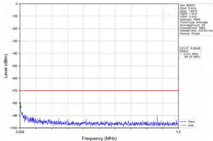
n78d_30kHz_MIMO_NTNV_100MHz_CP-OFDM_QPSK_3649.98MHz_Edge_1RB_Right
