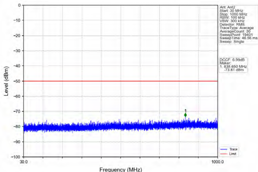
n78d_30kHz_MIMO_NTNV_90MHz_CP-OFDM_QPSK_3654.99MHz_Inner_1RB_Right
