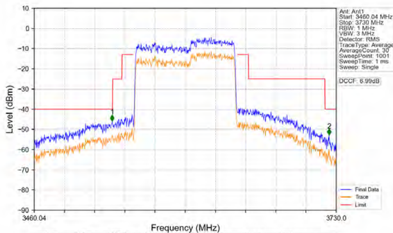
n78d_30kHz_MIMO_NTNV_90MHz_CP-OFDM_QPSK_3595.02MHz_Outer_Full
