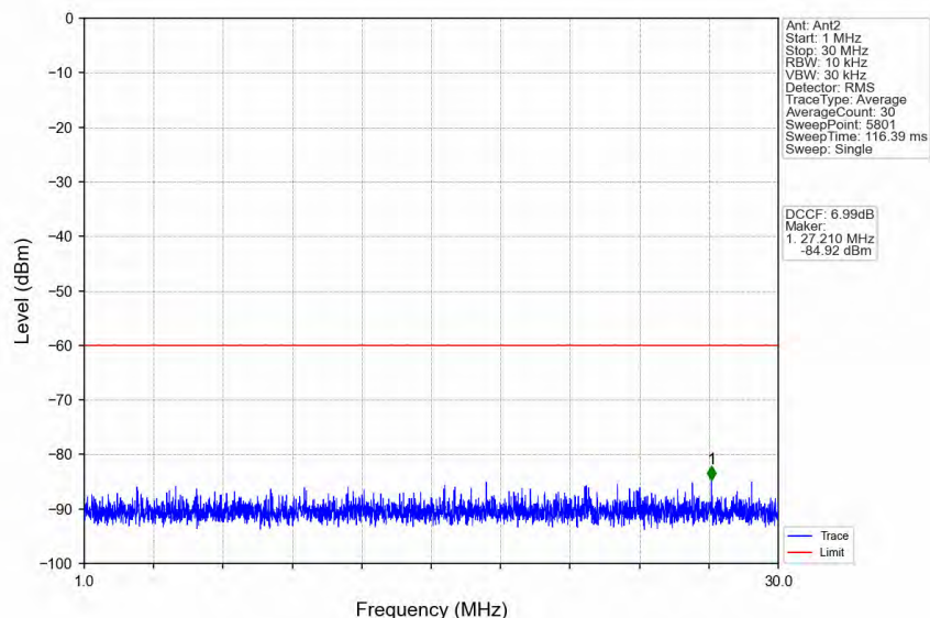
n78d_30kHz_MIMO_NTNV_80MHz_CP-OFDM_QPSK_3590.01MHz_Edge_1RB_Left
