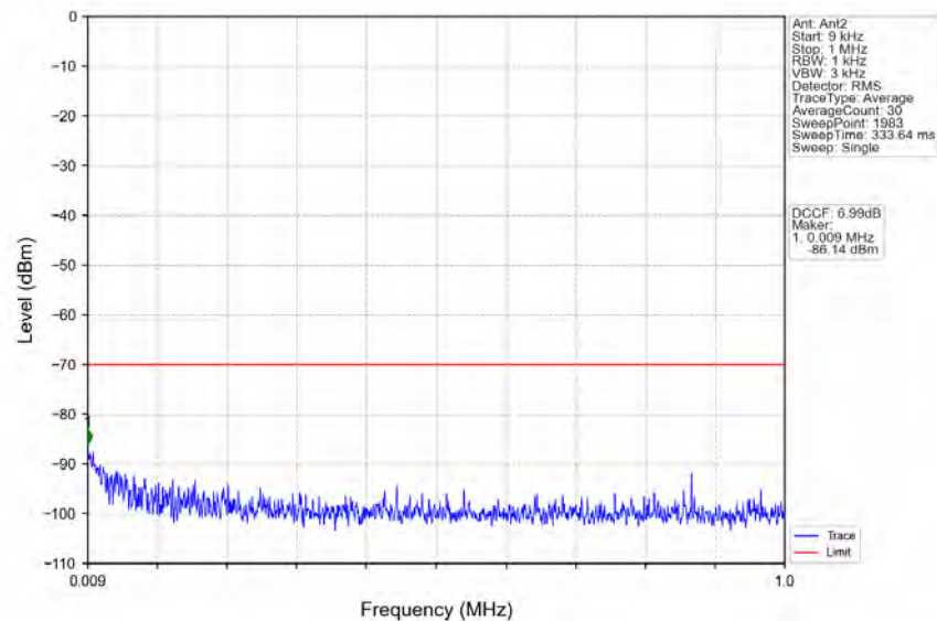
n78d_30kHz_MIMO_NTNV_100MHz_CP-OFDM_QPSK_3600MHz_Inner_1RB_Left
