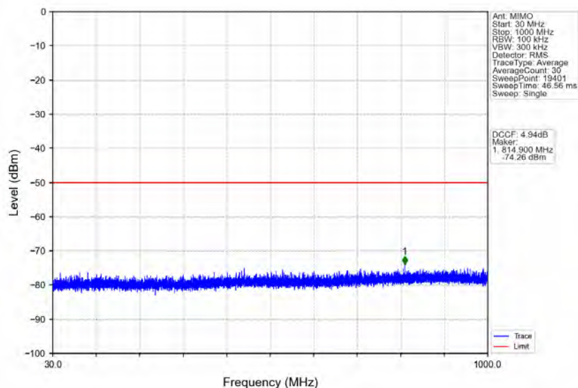
n78d_30kHz_MIMO_NTNV_80MHz_CP-OFDM QPSK_3660MHz_Edge_1RB_Right
