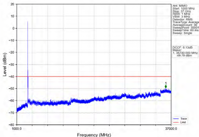
n78d_30kHz_MIMO_NTNV_90MHz_CP-OFDM_QPSK_3595.02MHz_Outer_Full
