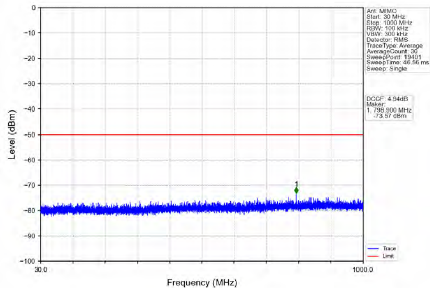
n78d_30kHz_MIMO_NTNV_100MHz_CP-OFDM QPSK_3600MHz_Inner_1RB_Left
