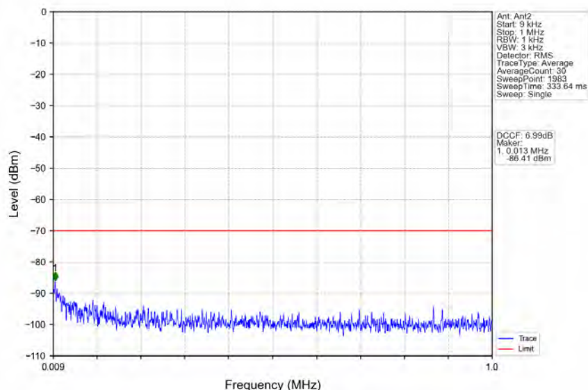
n78d_30kHz_MIMO_NTNV_90MHz_CP-OFDM_QPSK_3654.99MHz_Edge_1RB_Right
