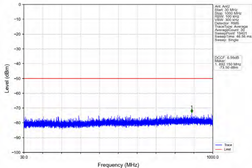
n78d_30kHz_MIMO_NTNV_100MHz_CP-OFDM_QPSK_3649.98MHz_Inner_1RB_Right
