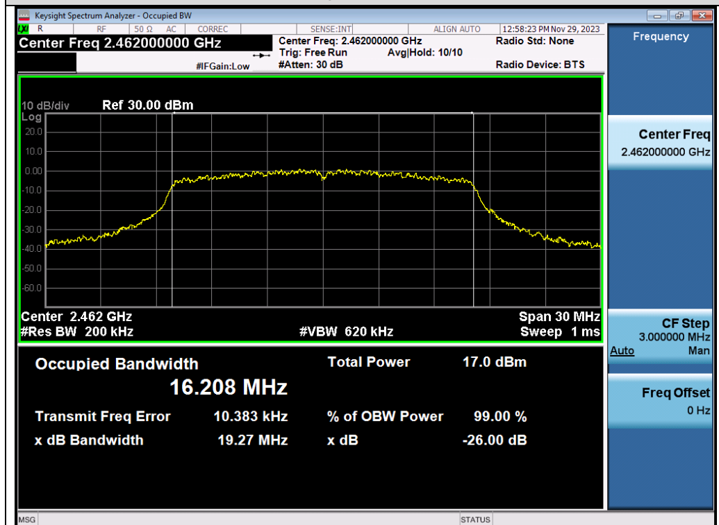
Test_Graph_802.11g_ANT1_2462_6Mbps_OBW
