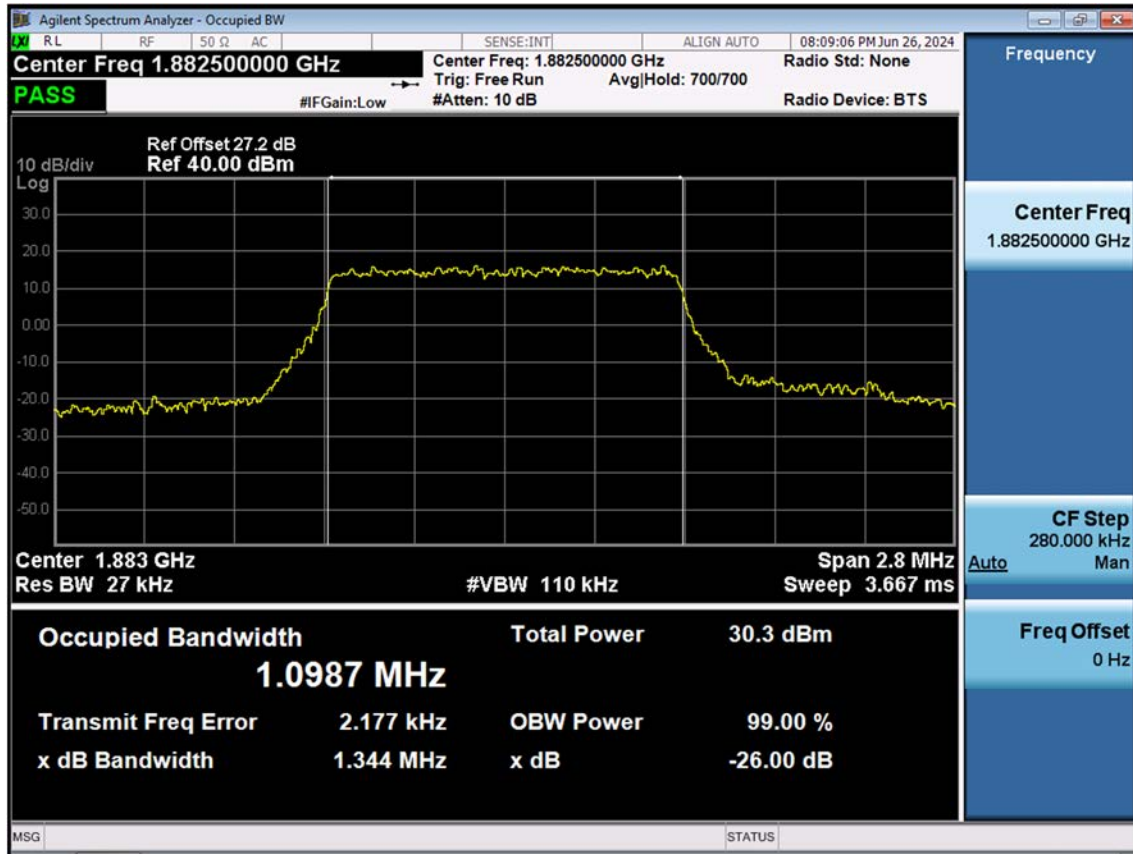
LTE B25(2)_1.4M_OBW_Mid_16QAM_FullRB
