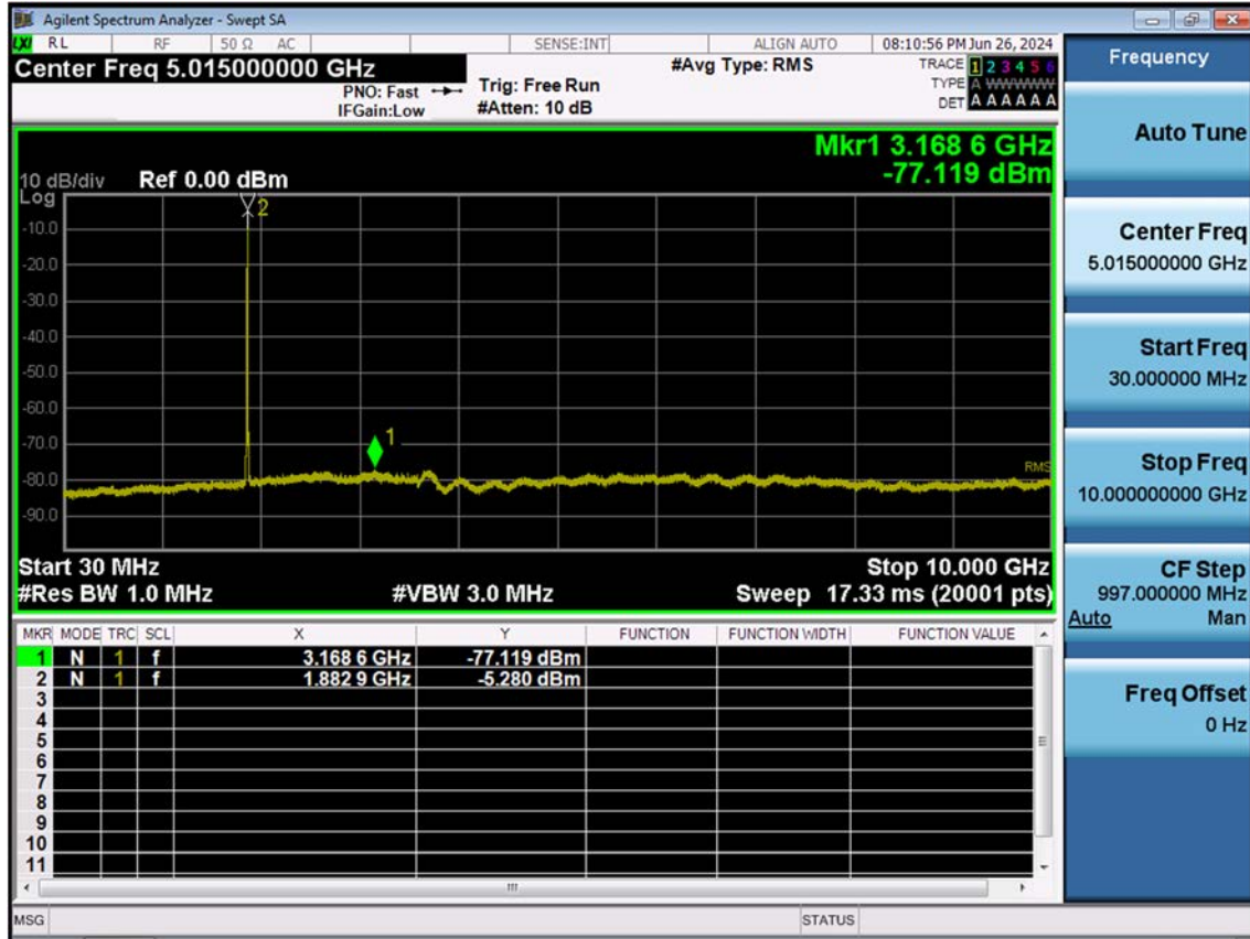
LTE B25(2)_1.4M_Conducted Spurious(30 M-10 G)_Mid_QPSK_1RB
