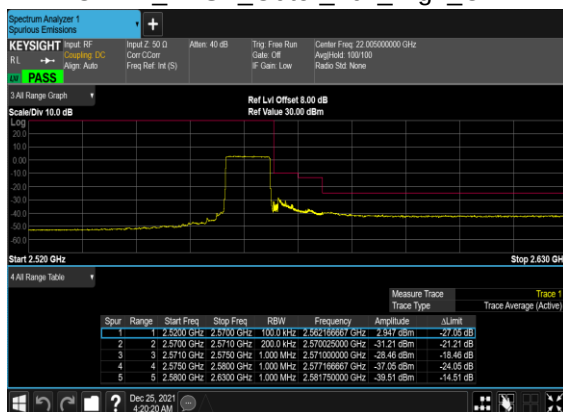
B5_N7(10M)_DFT-s- OFDM_BPSK_Outer_Full_High_CH
