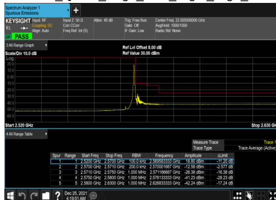
B5_N7(10M)_DFT-s- OFDM_QPSK_Edge_1RB_Right_High_CH
