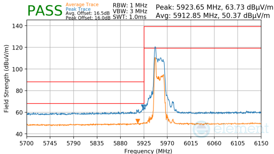
Plot 7-1013. Antenna WF8 Radiated Lower Band Edge (Peak/Average – UNII Band 5 – RU26)
