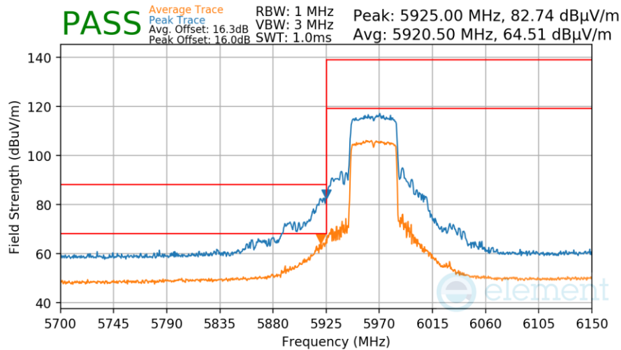
Plot 7-1019. Antenna WF8 Radiated Lower Band Edge (Peak & Average – UNII Band 5 – RU484)
