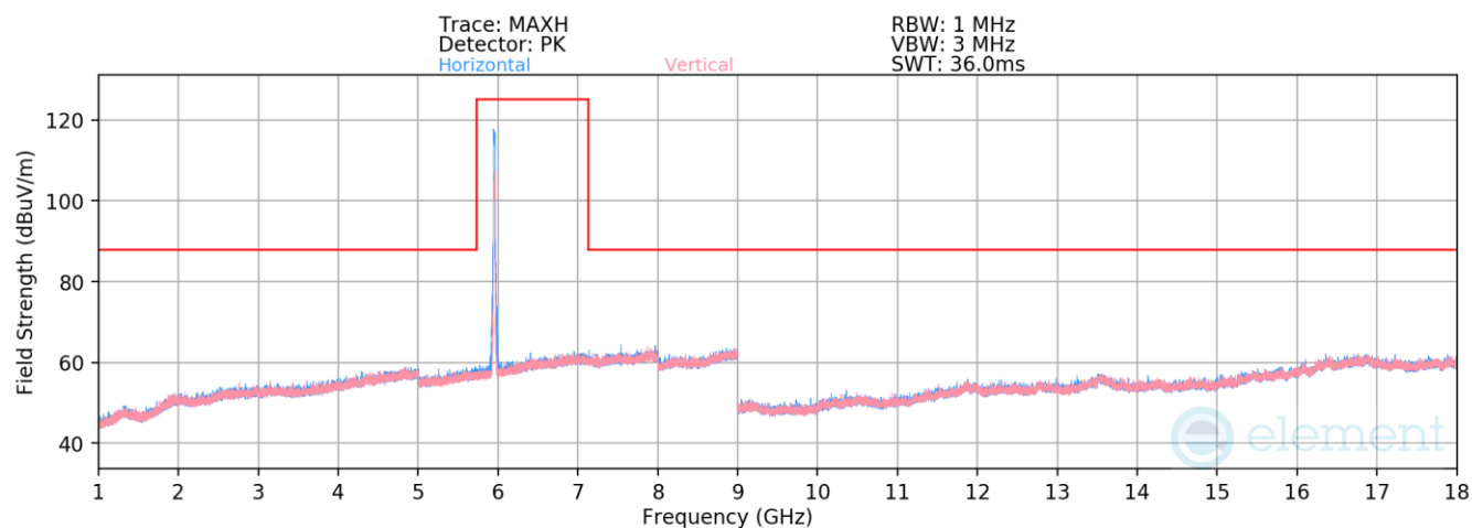
Plot 7-997. Radiated Spurious Emissions above 1GHz SDM (802.11ax – Ch. 1 – RU242)
