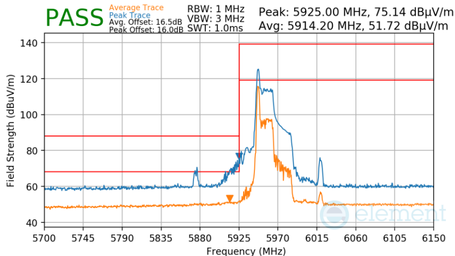
Plot 7-1017. Antenna WF8 Radiated Lower Band Edge (Peak & Average – UNII Band 5 – RU26)
