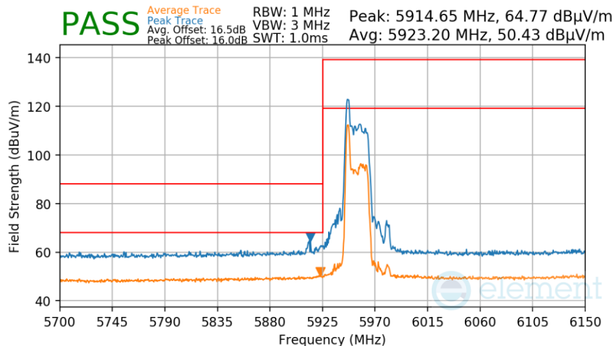
Plot 7-1032. Antenna WF7a Radiated Lower Band Edge (Peak/Average – UNII Band 5 – RU26)
