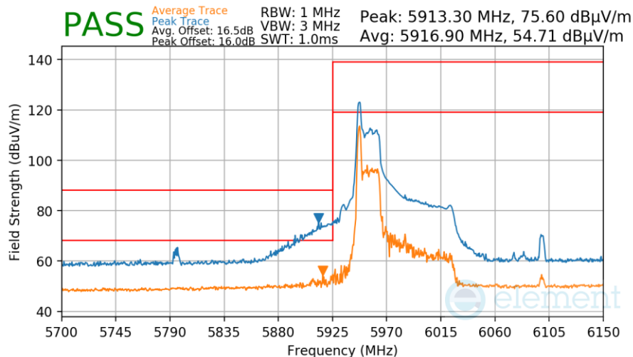
Plot 7-1022. Antenna WF8 Radiated Lower Band Edge (Peak & Average – UNII Band 5 – RU26)
