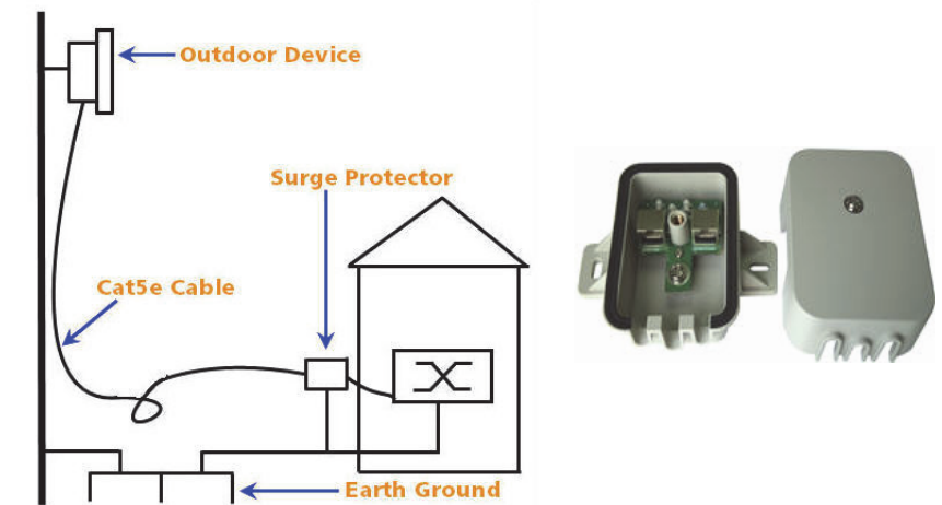
Figure 6: Surge Protector
