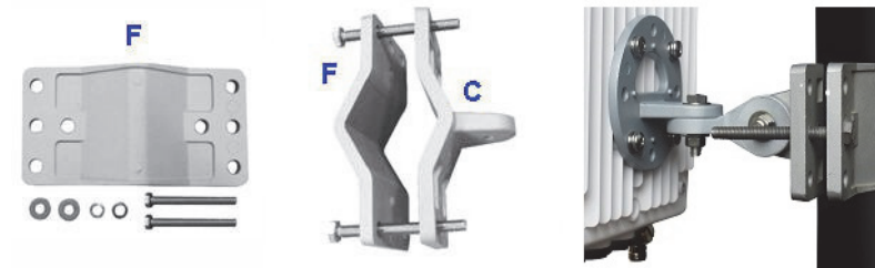
Figure 4: Pole Mounting
