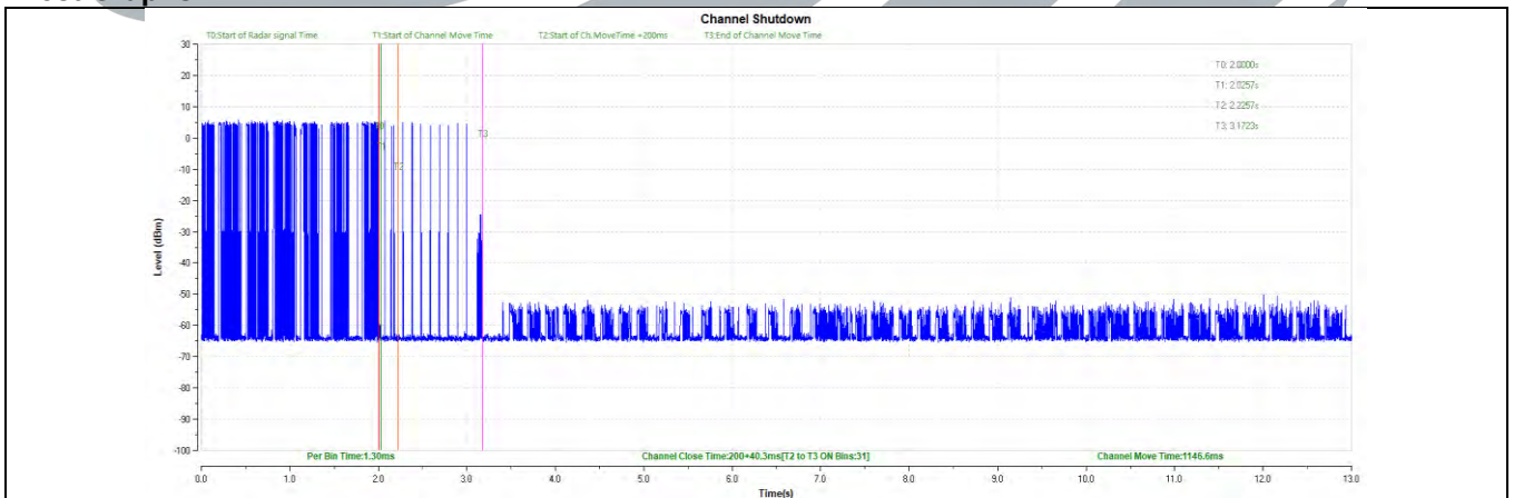
11AC20SISO-5300-Type0-PASS
