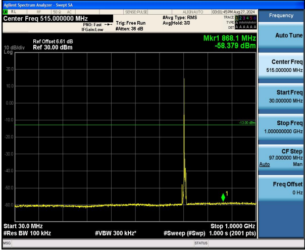
Band12_5MHz_16QAM_23155_1RB#0_30~1000_30~1000
