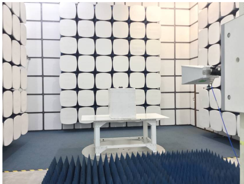
PTC test site: Radiated Emission from 1GHz to 18GHz
