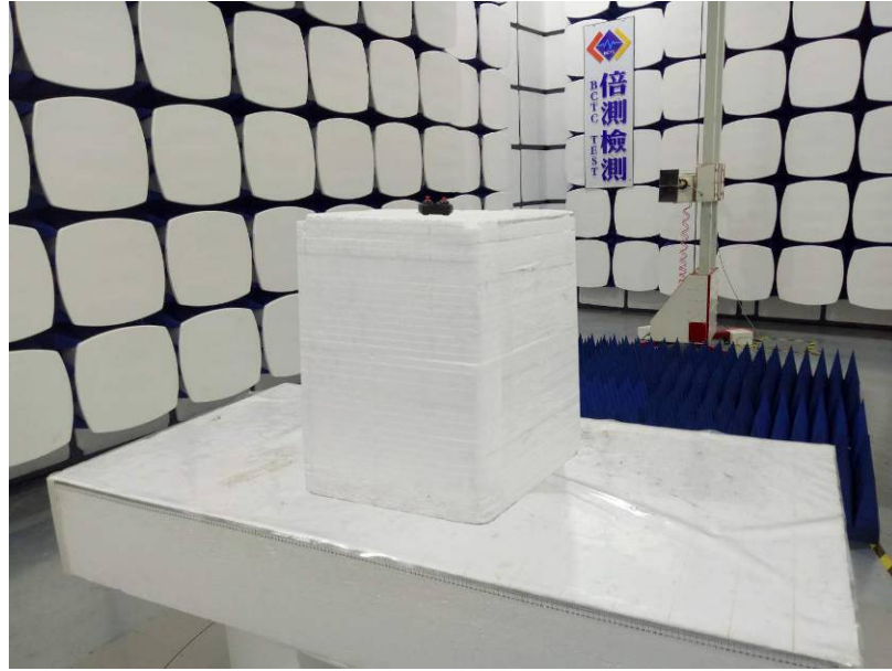
BCTC test site: Radiated Emission from 18GHz to 25GHz
