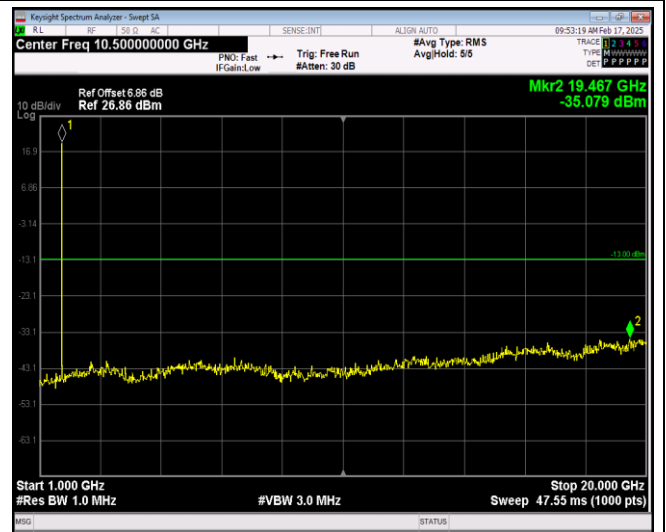
Band66-1.4MHz-64QAM-132322-1RB#0-Range2:1000~20000MHz
