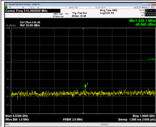
Band66-20MHz-64QAM-132072-1RB#0-Range1:30~1000MHz
