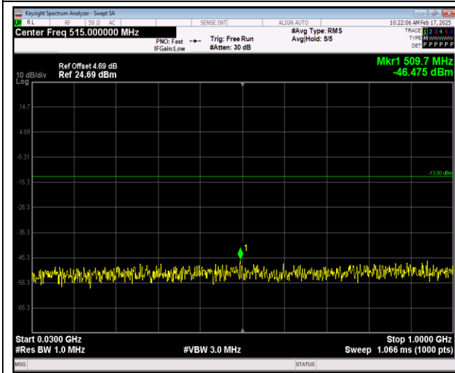
Band66-20MHz-64QAM-132072-1RB#0-Range1:30~1000MHz
