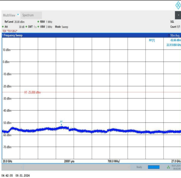
Band41_5MHz_QPSK_40620_1RB#0_20000~27000_20000~27000
