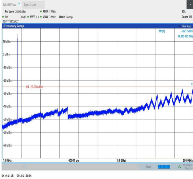
Band41_5MHz_16QAM_39675_25RB#0_1000~20000_1000~20000
