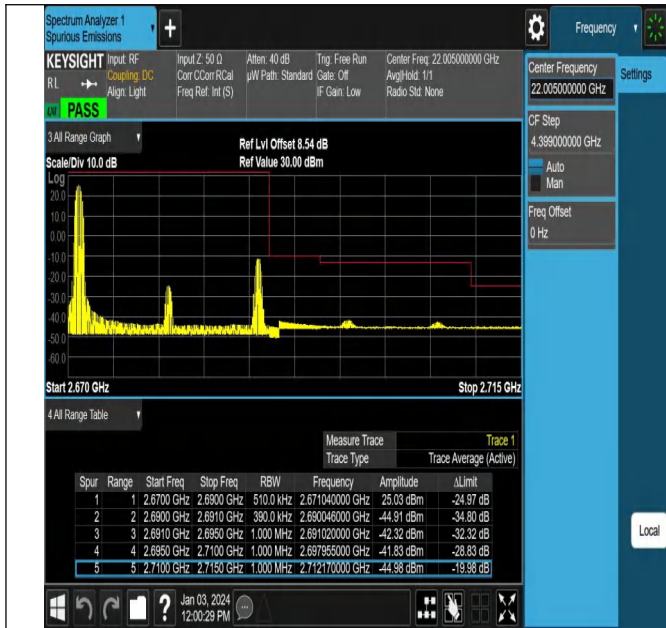
Band41_20MHz_16QAM_41490_1RB#0
