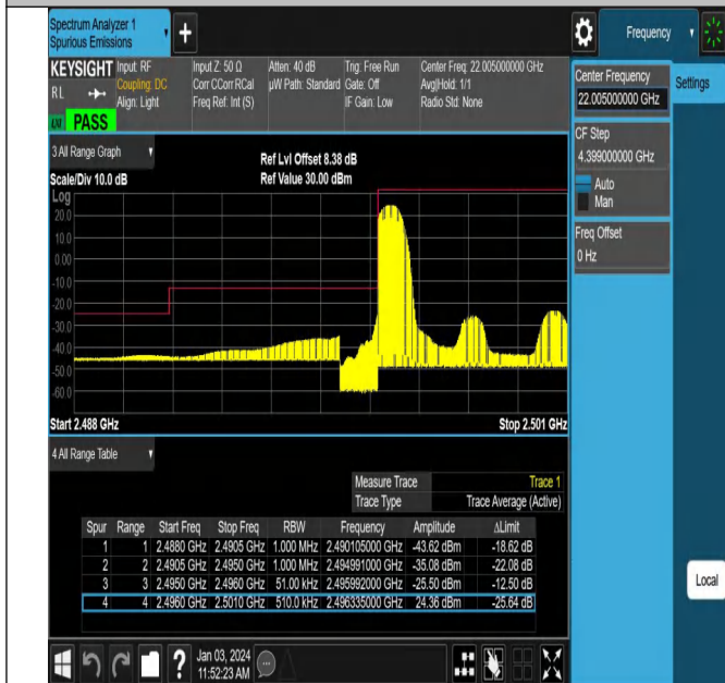
Band41_5MHz_16QAM_39675_1RB#0
