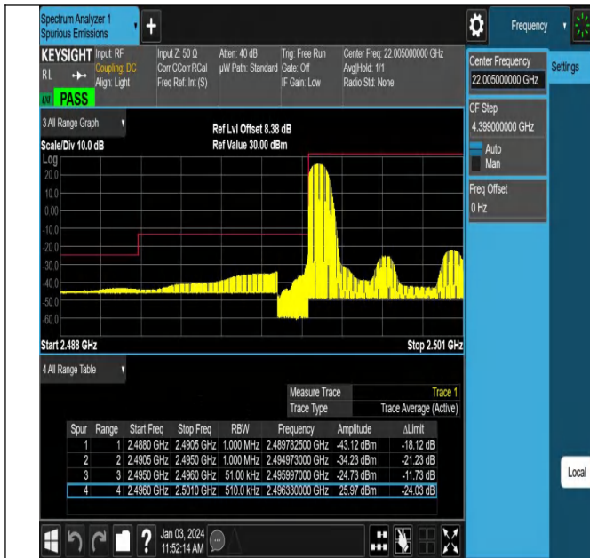
Band41_5MHz_QPSK_39675_1RB#0
