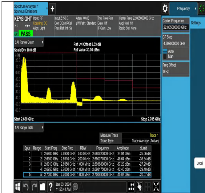
Band41_10MHz_16QAM_41540_1RB#0
