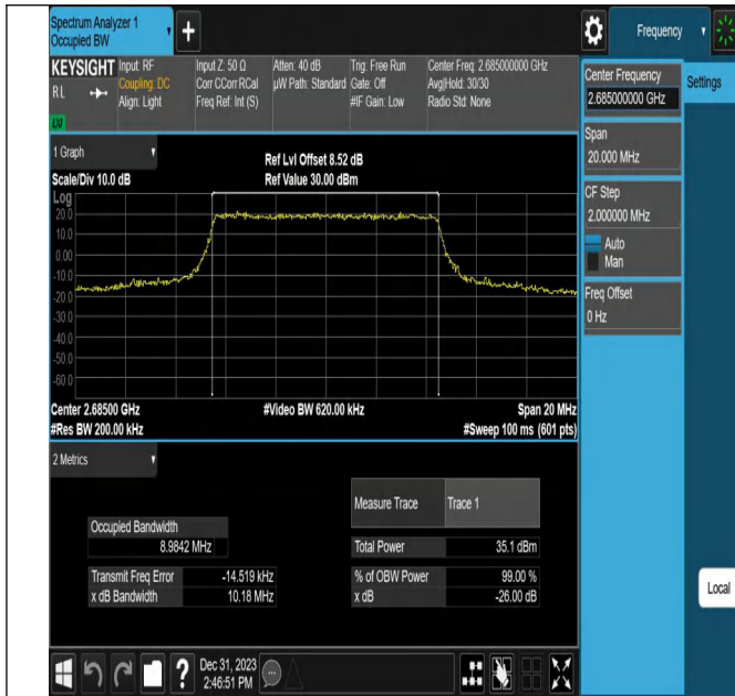
Band41-10MHz-QPSK-41540-50RB#0-PASS
