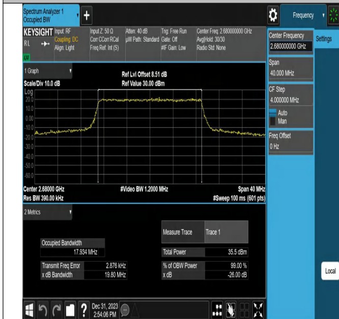
Band41-20MHz-QPSK-41490-100RB#0-PASS
