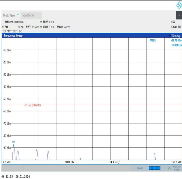
Band41_5MHz_QPSK_40620_1RB#0_0.009~0.15_0.009~0.15
