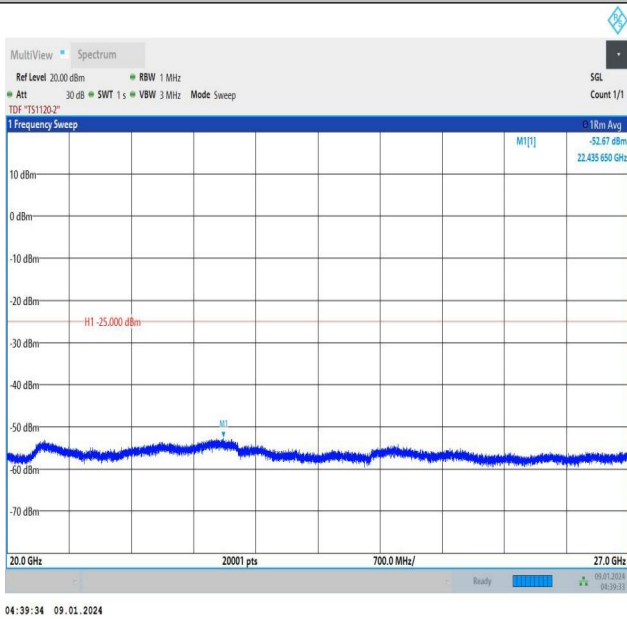
Band41_5MHz_QPSK_39675_1RB#24_20000~27000_20000~27000
