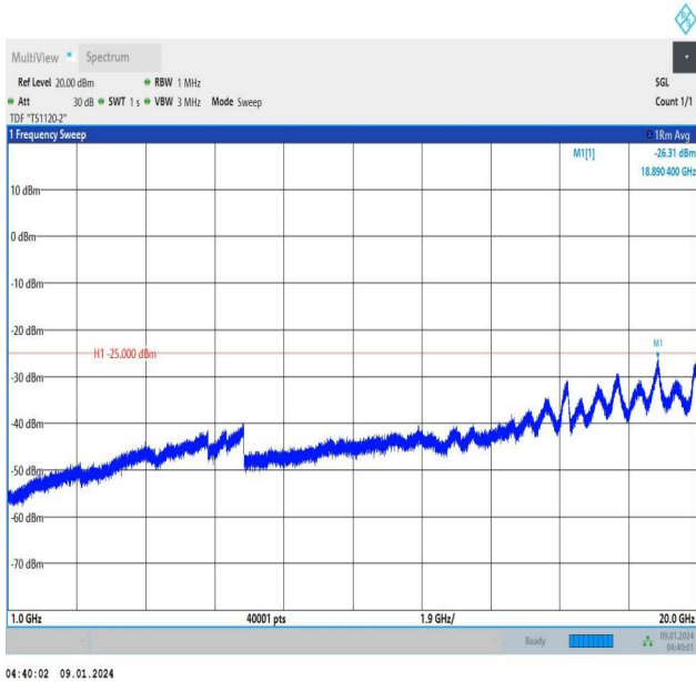
Band41_5MHz_16QAM_39675_1RB#24_1000~20000_1000~20000
