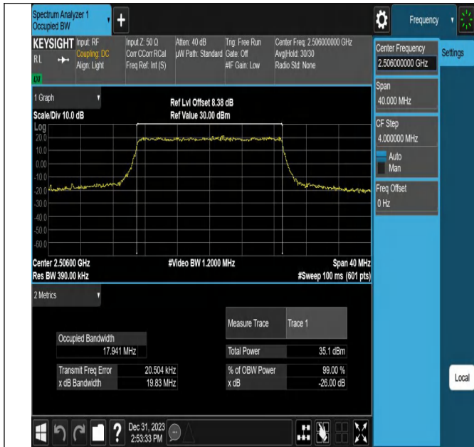
Band41-20MHz-QPSK-39750-100RB#0-PASS
