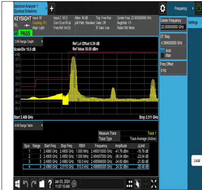
Band41_15MHz_16QAM_39725_1RB#0
