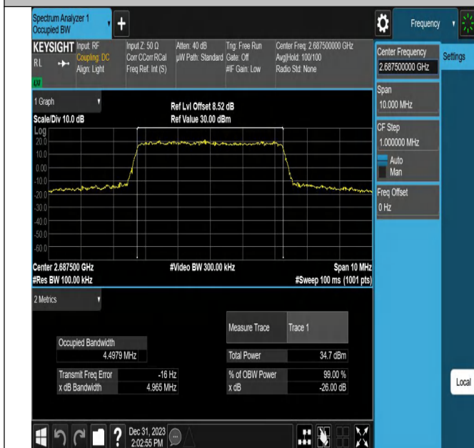
Band41-5MHz-QPSK-41565-25RB#0-PASS
