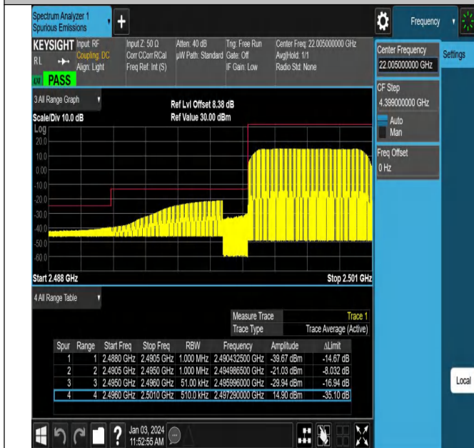
Band41_5MHz_QPSK_39675_25RB#0
