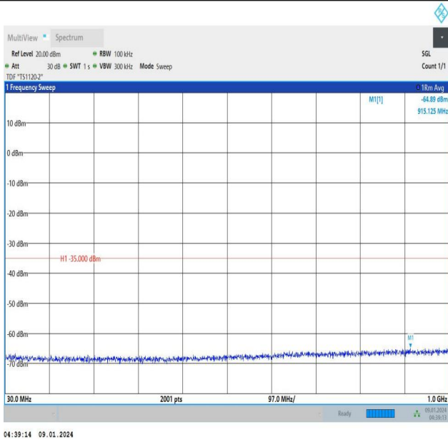
Band41_5MHz_QPSK_39675_1RB#24_30~1000_30~1000
