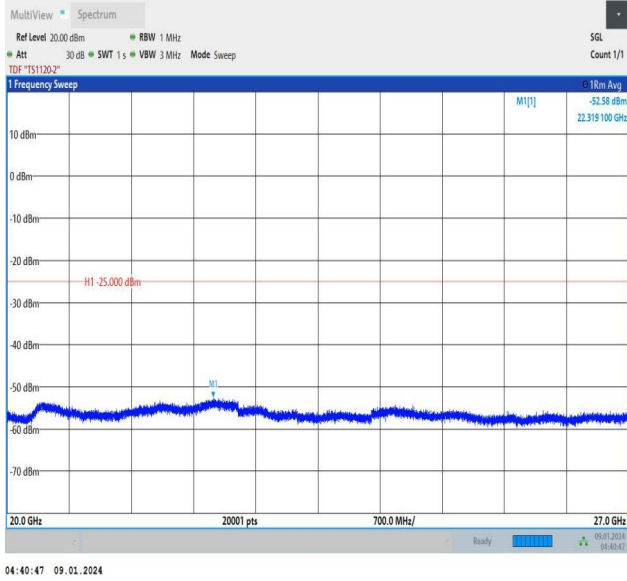
Band41_5MHz_QPSK_39675_25RB#0_20000~27000_20000~27000
