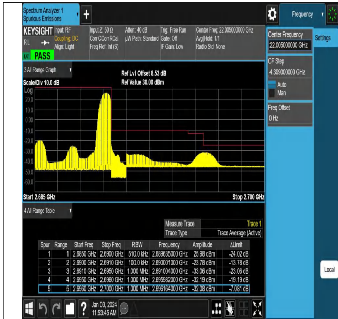
Band41_5MHz_QPSK_41565_1RB#24
