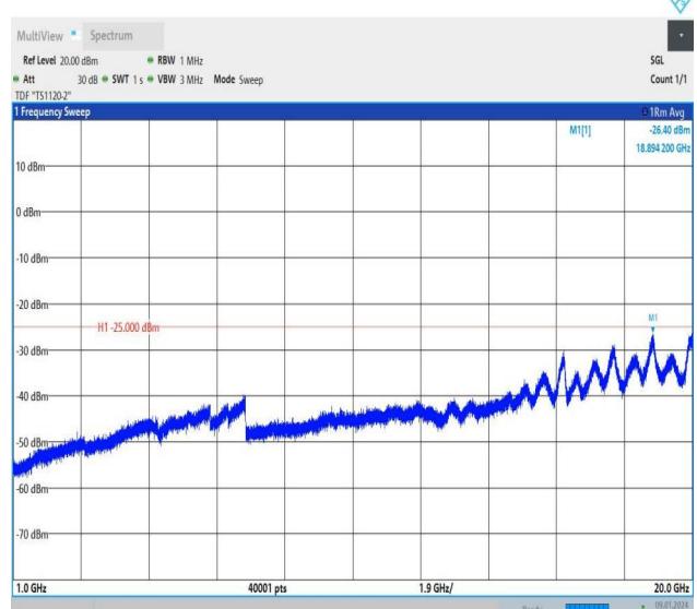
Band41_5MHz_QPSK_39675_1RB#0_1000~20000_1000~20 000
