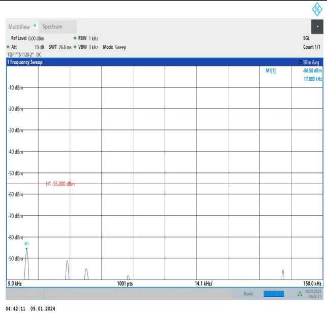
Band41_5MHz_16QAM_40620_1RB#0_0.009~0.15_0.009~0.15
