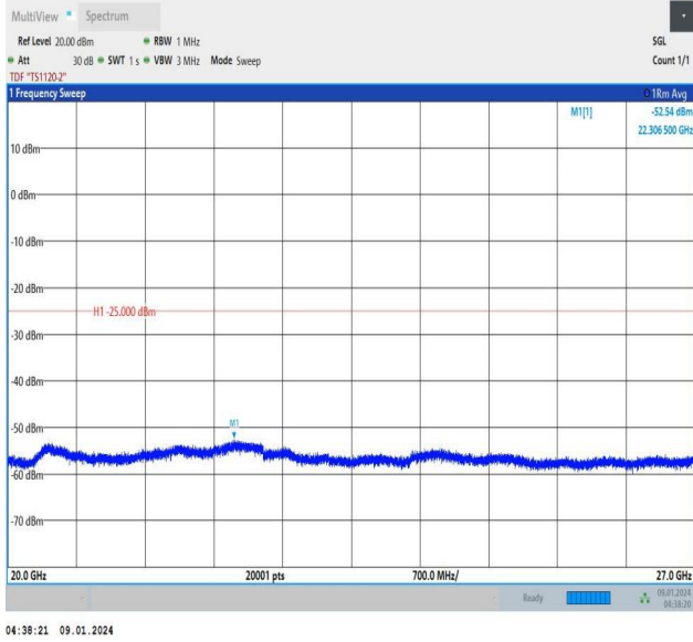
Band41_5MHz_QPSK_39675_1RB#0_20000~27000_20000~27000
