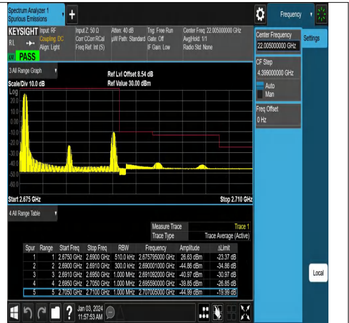
Band41_15MHz_QPSK_41515_1RB#0
