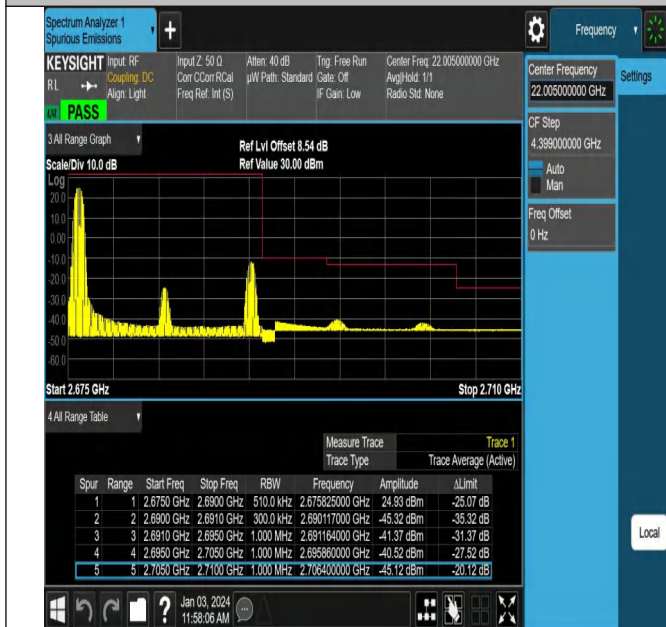
Band41_15MHz_16QAM_41515_1RB#0
