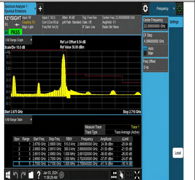
Band41_15MHz_16QAM_41515_1RB#74
