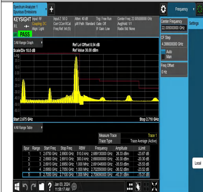
Band41_15MHz_QPSK_41515_1RB#74
