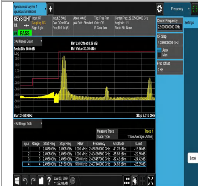
Band41_20MHz_16QAM_39750_1RB#0
