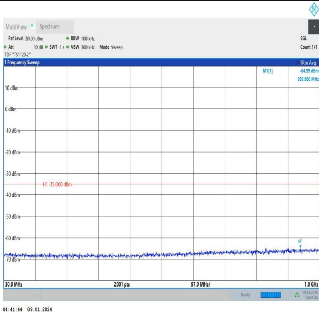
Band41_5MHz_QPSK_40620_1RB#0_30~1000_30~1000
