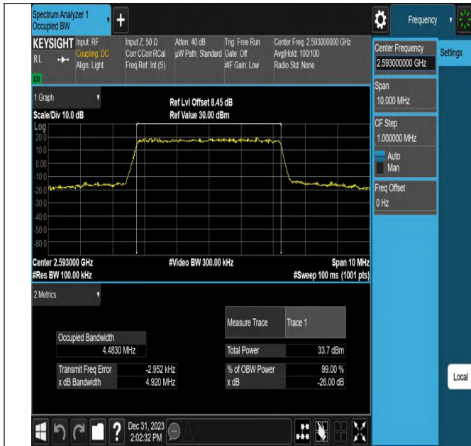
Band41-5MHz-16QAM-40620-25RB#0-PASS
