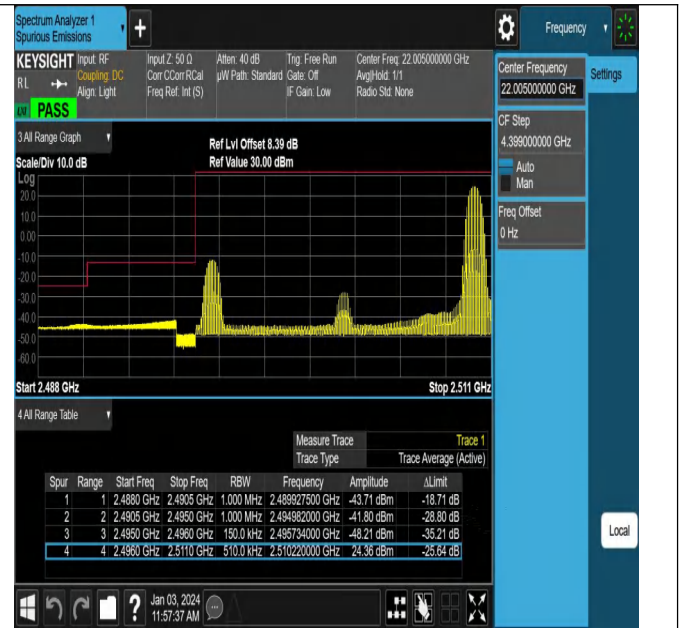
Band41_15MHz_16QAM_39725_1RB#74
