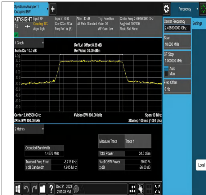
Band41-5MHz-QPSK-39675-25RB#0-PASS
