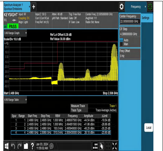
Band41_10MHz_QPSK_39700_1RB#49
