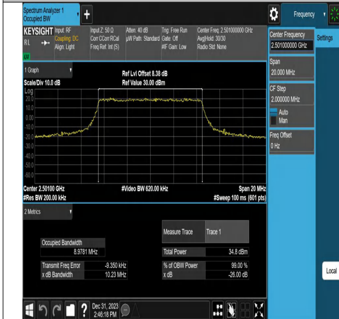
Band41-10MHz-QPSK-39700-50RB#0-PASS
