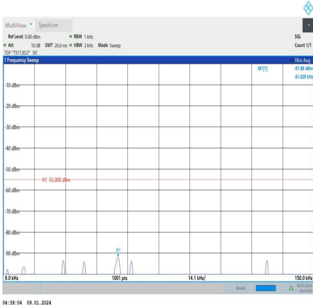
Band41_5MHz_QPSK_39675_1RB#24_0.009~0.15_0.009~0.15
