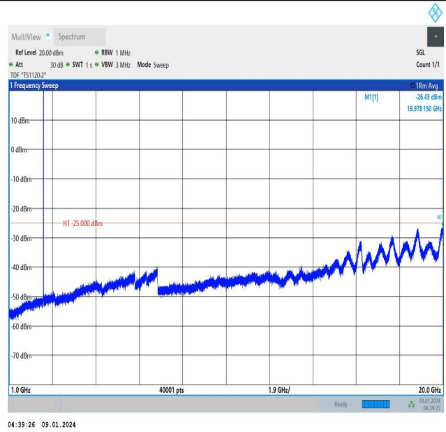
Band41_5MHz_QPSK_39675_1RB#24_1000~20000_1000~20000
