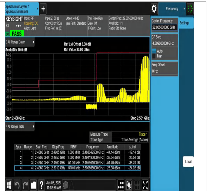
Band41_5MHz_QPSK_39675_1RB#24
