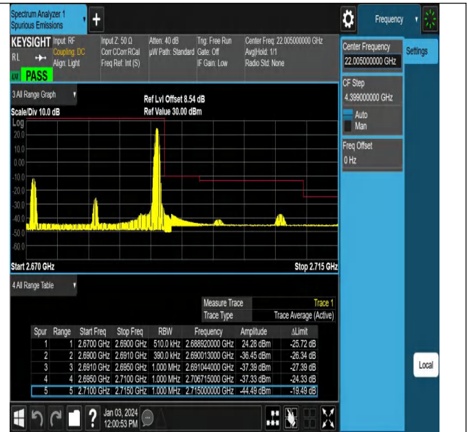
Band41_20MHz_16QAM_41490_1RB#99
