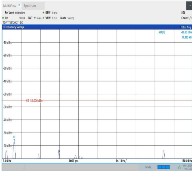
Band41_5MHz_QPSK_39675_1RB#0_0.009~0.15_0.009~0.1 5
