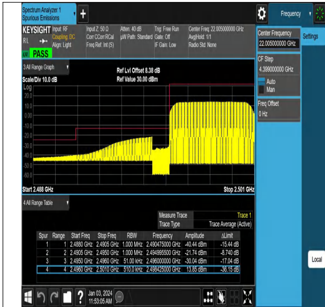
Band41_5MHz_16QAM_39675_25RB#0
