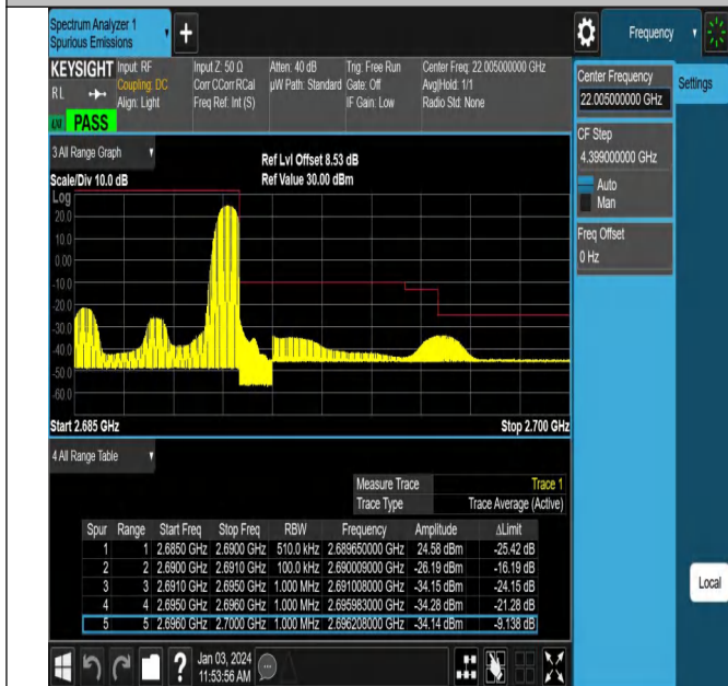
Band41_5MHz_16QAM_41565_1RB#24
