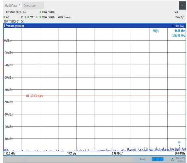
Band41_5MHz_QPSK_39675_1RB#0_0.15~30_0.15~30
