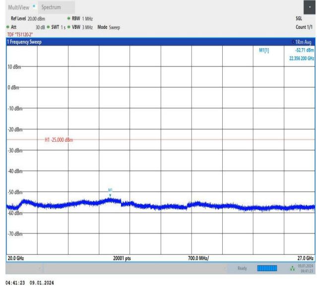
Band41_5MHz_16QAM_39675_25RB#0_20000~27000_20000~27000
