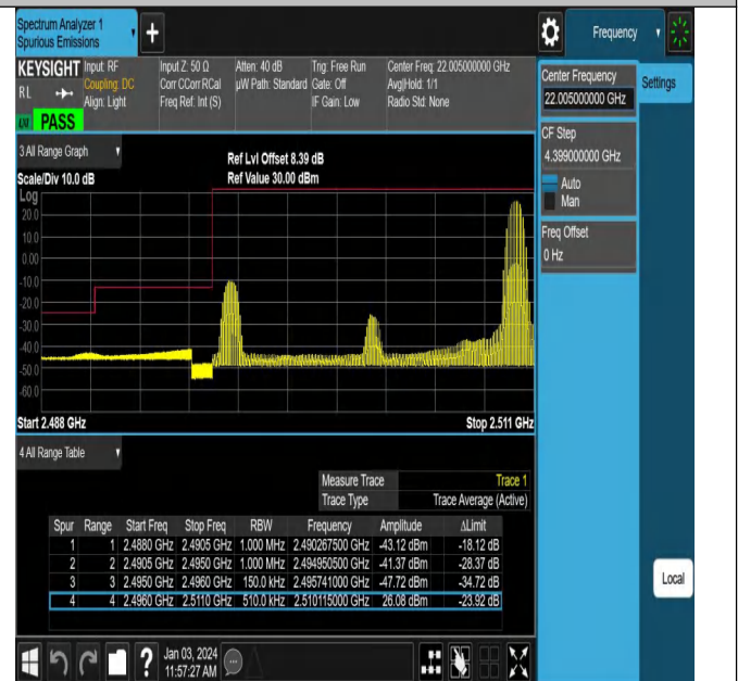
Band41_15MHz_QPSK_39725_1RB#74
