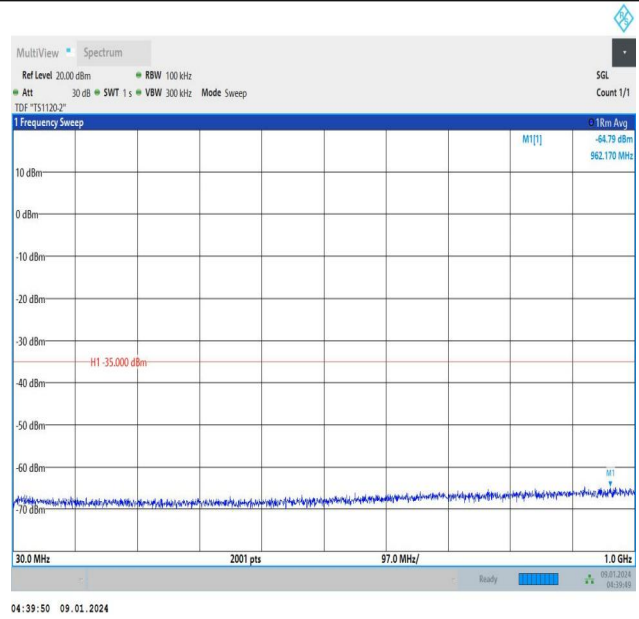
Band41_5MHz_16QAM_39675_1RB#24_30~1000_30~1000
