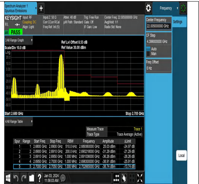
Band41_10MHz_16QAM_41540_1RB#49
