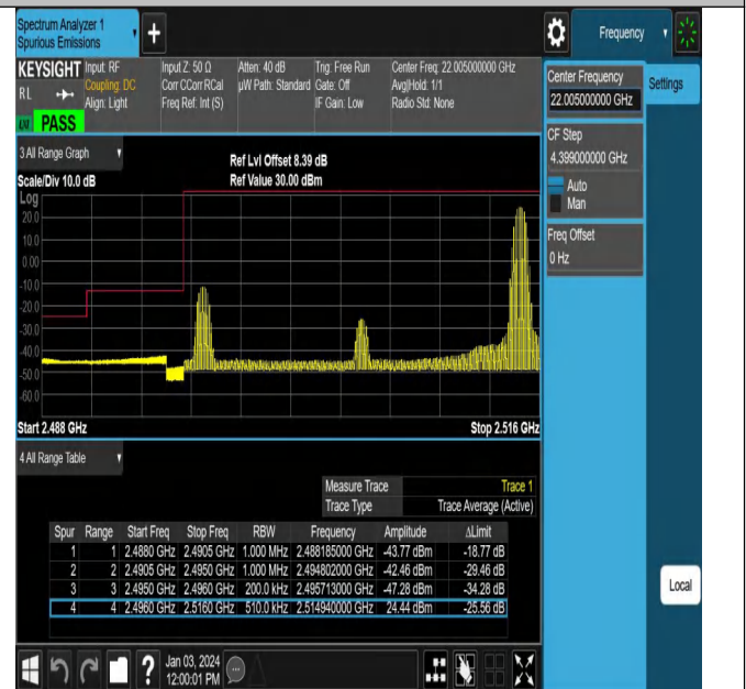
Band41_20MHz_16QAM_39750_1RB#99
