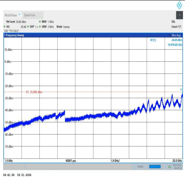
Band41_5MHz_QPSK_40620_1RB#0_1000~20000_1000~20000
