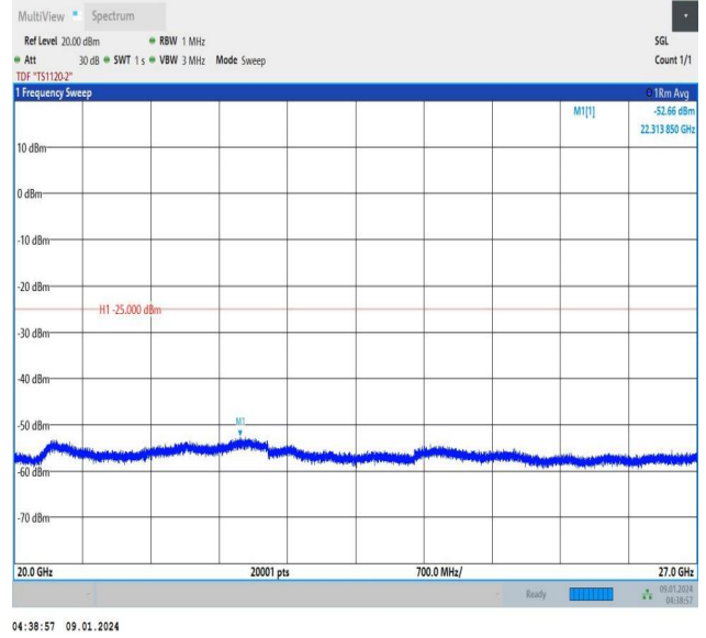
Band41_5MHz_16QAM_39675_1RB#0_20000~27000_20000
