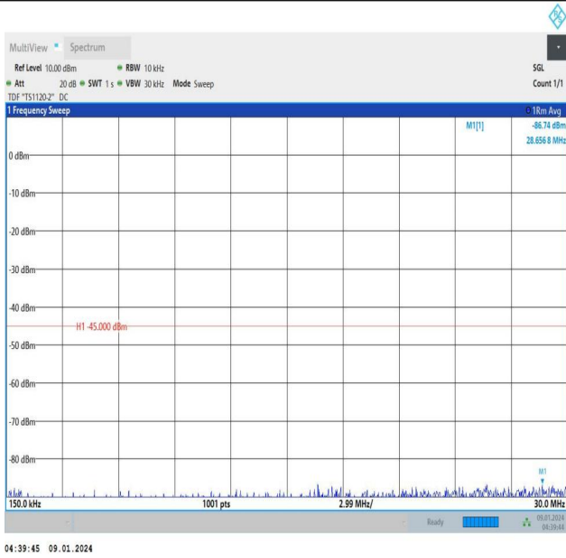
Band41_5MHz_16QAM_39675_1RB#24_0.15~30_0.15~30
