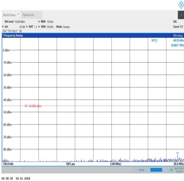
Band41_5MHz_16QAM_39675_1RB#0_0.15~30_0.15~30
