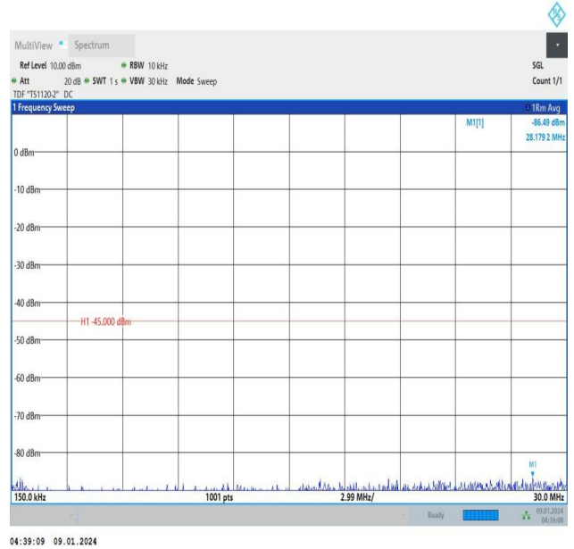
Band41_5MHz_QPSK_39675_1RB#24_0.15~30_0.15~30
