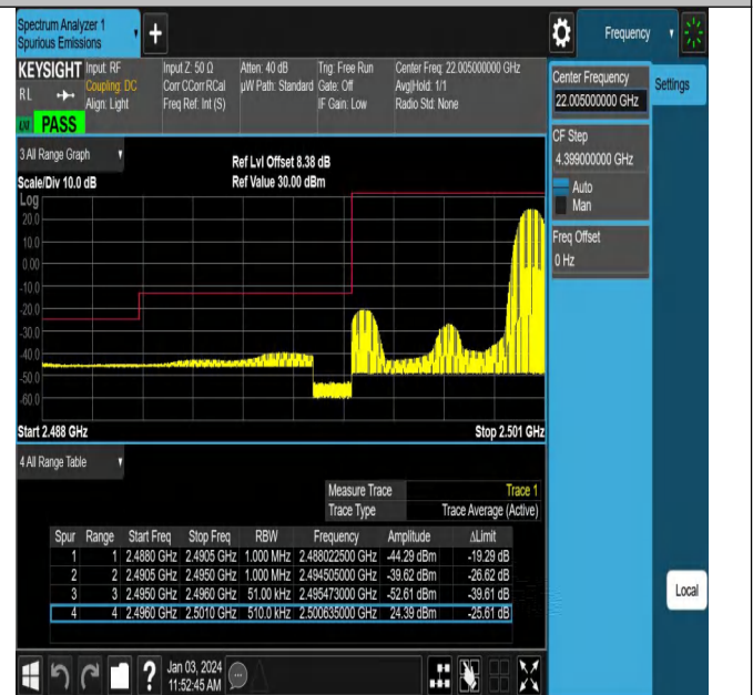
Band41_5MHz_16QAM_39675_1RB#24
