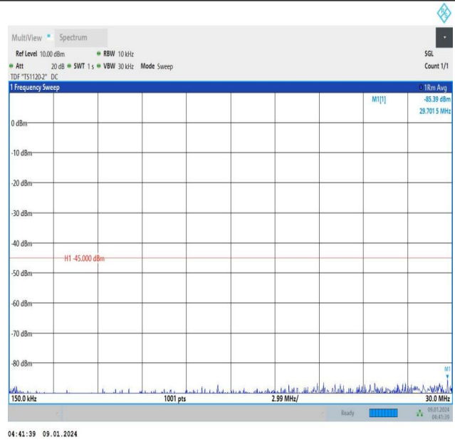
Band41_5MHz_QPSK_40620_1RB#0_0.15~30_0.15~30
