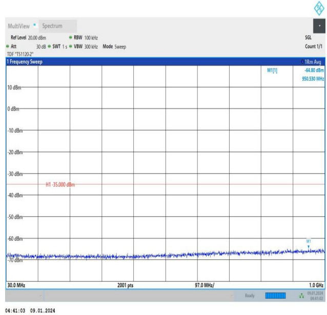
Band41_5MHz_16QAM_39675_25RB#0_30~1000_30~1000
