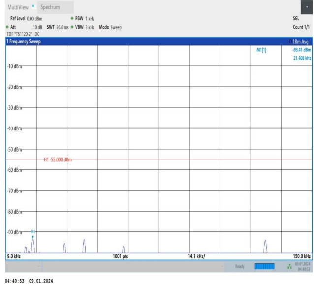
Band41_5MHz_16QAM_39675_25RB#0_0.009~0.15_0.009~0.15
