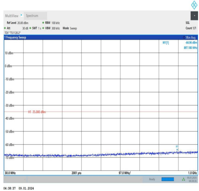
Band41_5MHz_16QAM_39675_1RB#0_30~1000_30~1000
