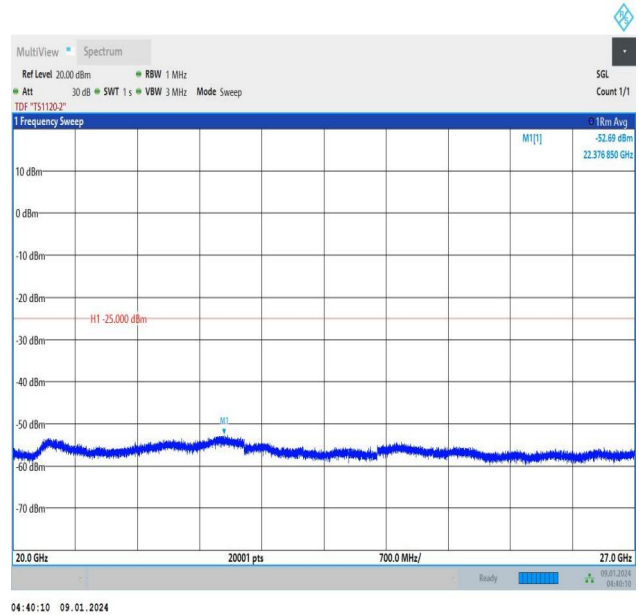
Band41_5MHz_16QAM_39675_1RB#24_20000~27000_20000~27000
