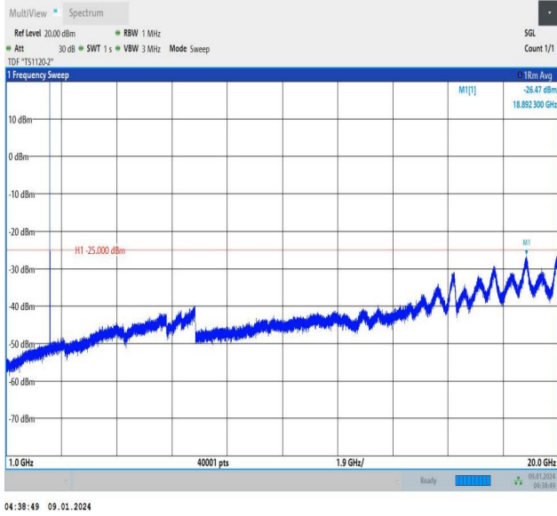
Band41_5MHz_16QAM_39675_1RB#0_1000~20000_1000~20000
