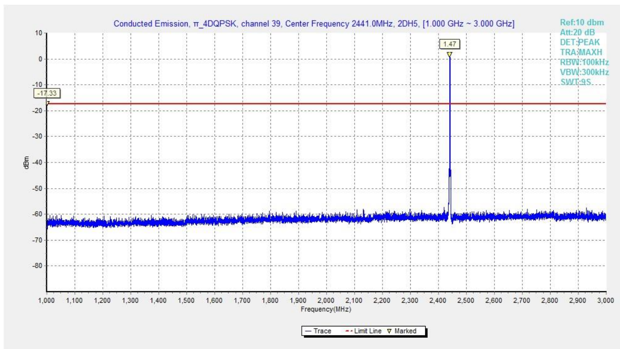
Fig. 35 Conducted Spurious Emission ( \pi/4 DQPSK, Ch39, 1GHz-3 GHz)
