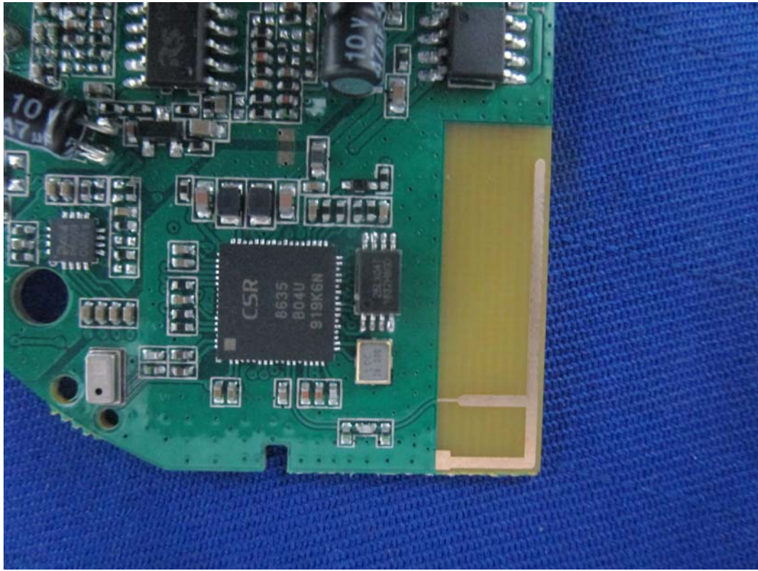
RF chip&ANT
