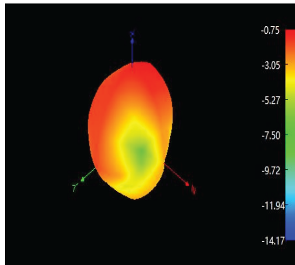
3D Radiation Pattern for 2440MHz
