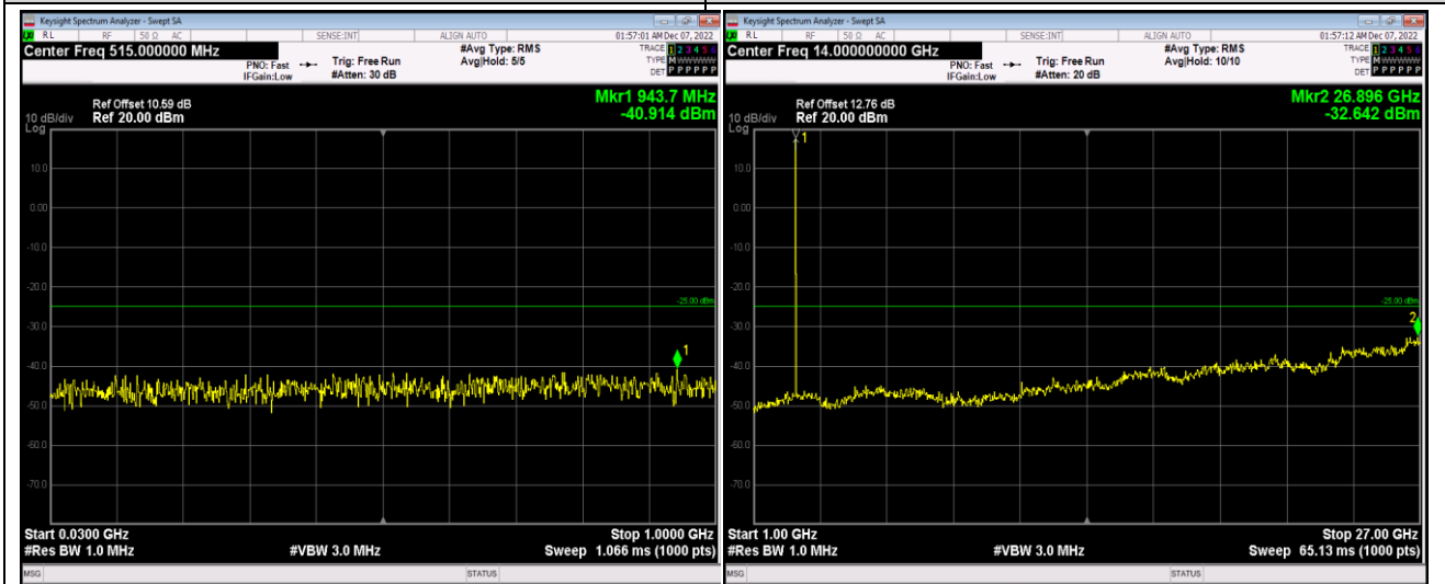
Band41-20MHz-QPSK-40140-1RB#0-Range1:30~1000MHz
