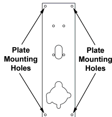
Figure 2-10 – Reader Scar/Push Plate Mounting Holes
