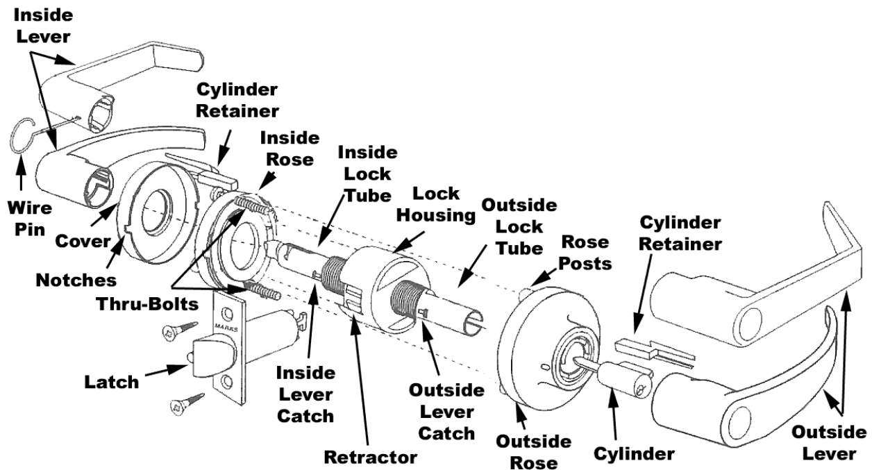
Figure 2-38 – Exploded Lock Hardware
