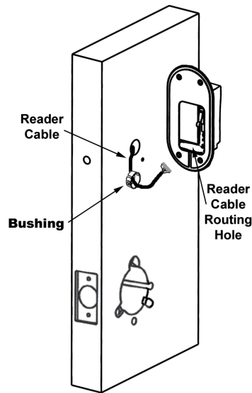
Figure 2-32 – Reader Cable Routing
