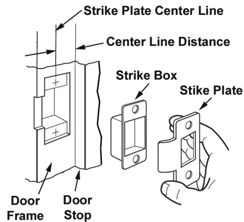
Figure 2-44 – Installing Strike Plate
