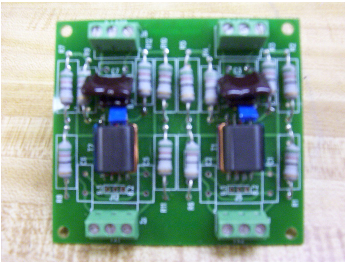
Liberty FX Shielded Matching Board Component Side
