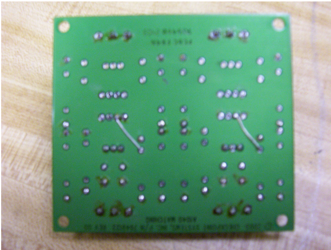
Liberty FX Shielded Matching Board Solder Side
