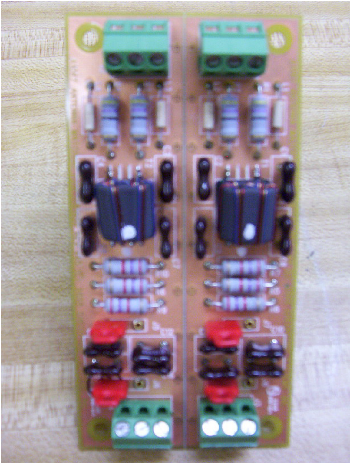
Liberty FX Unshielded Matching Board Component Side
