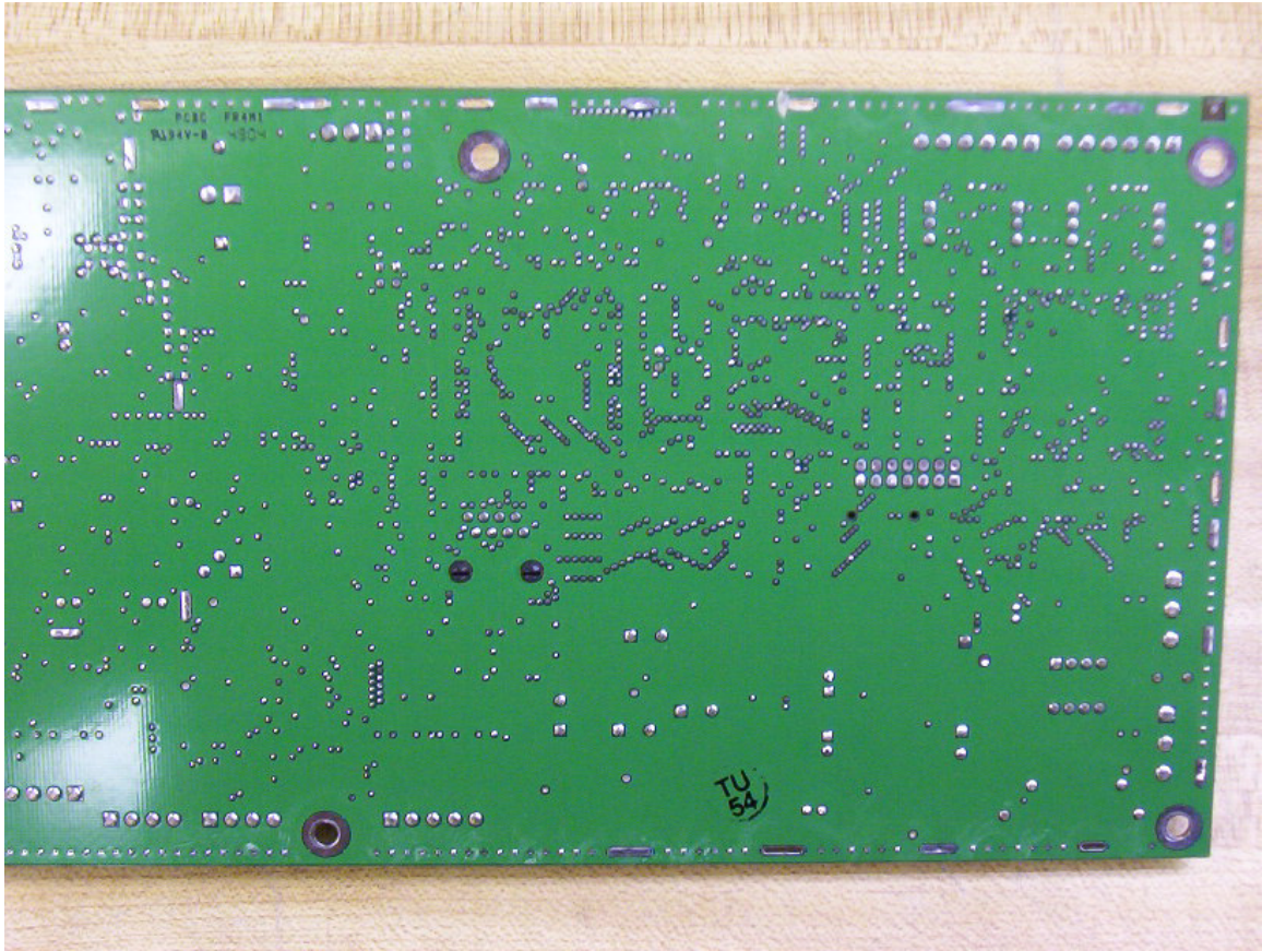
Liberty FX TR4024 PCB Solder Left Side
