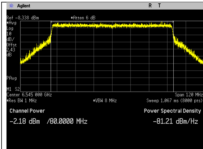
6545MHz_119_80MHz BW_be-mode_Chain 2
