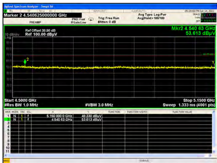
U-NII-1 11ax160(SU) CH50 Peak
