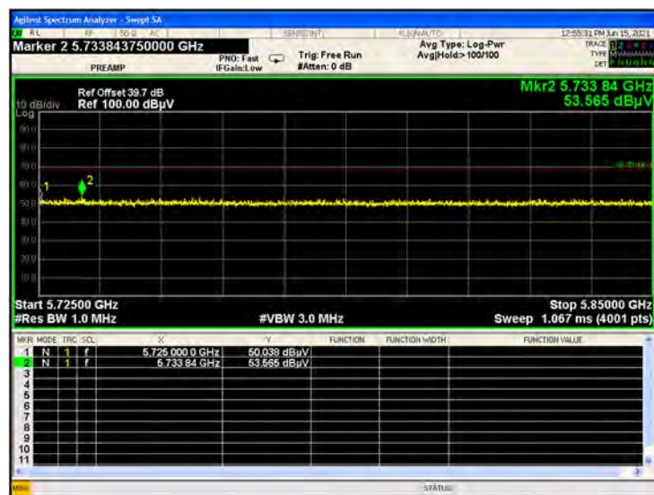
U-NII-2C 11ax20(SU) CH140 Peak
