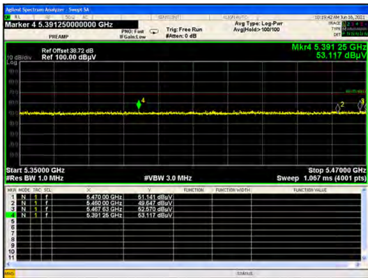
U-NII-2C 11ac160 CH114 Peak
