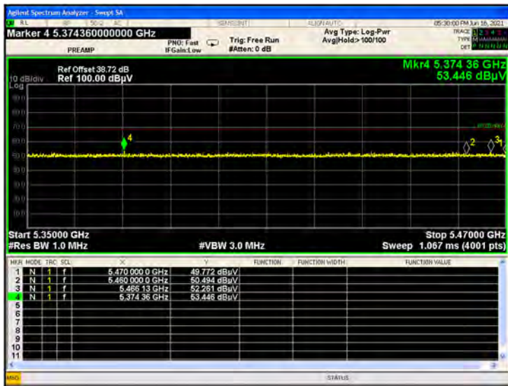
U-NII-2C 11ac80 CH138 Peak
