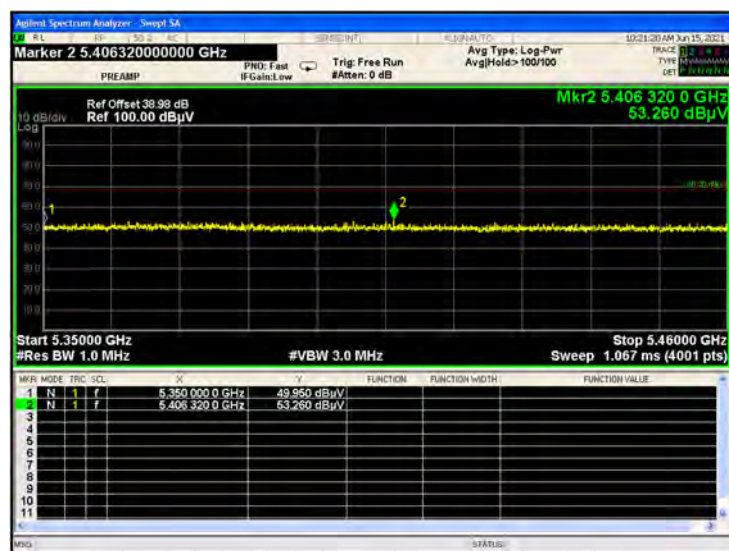
U-NII-2A 11a CH64 Peak
