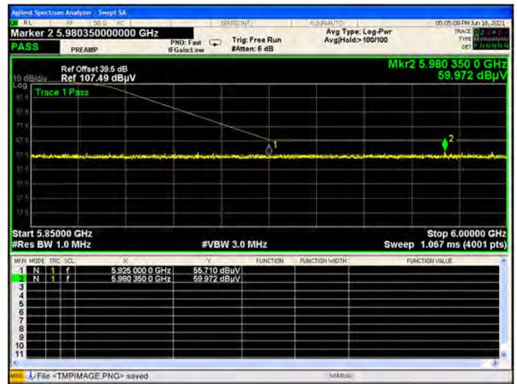
U-NII-2C 11ax20(SU) CH144 Peak
