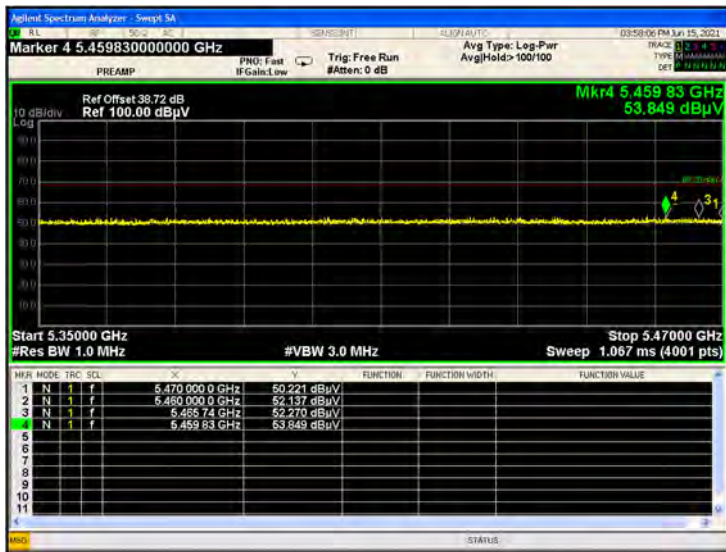
U-NII-2C 11ax160(SU) CH114 Peak
