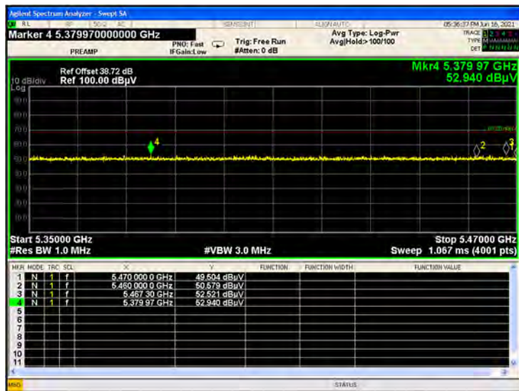
U-NII-2C 11ax80(SU) CH138 Peak
