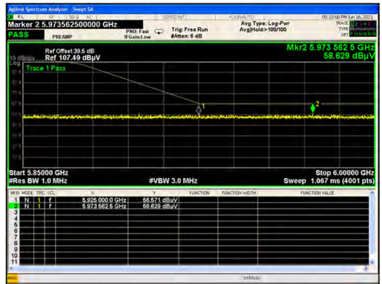
U-NII-2C 11ac80 CH138 Peak
