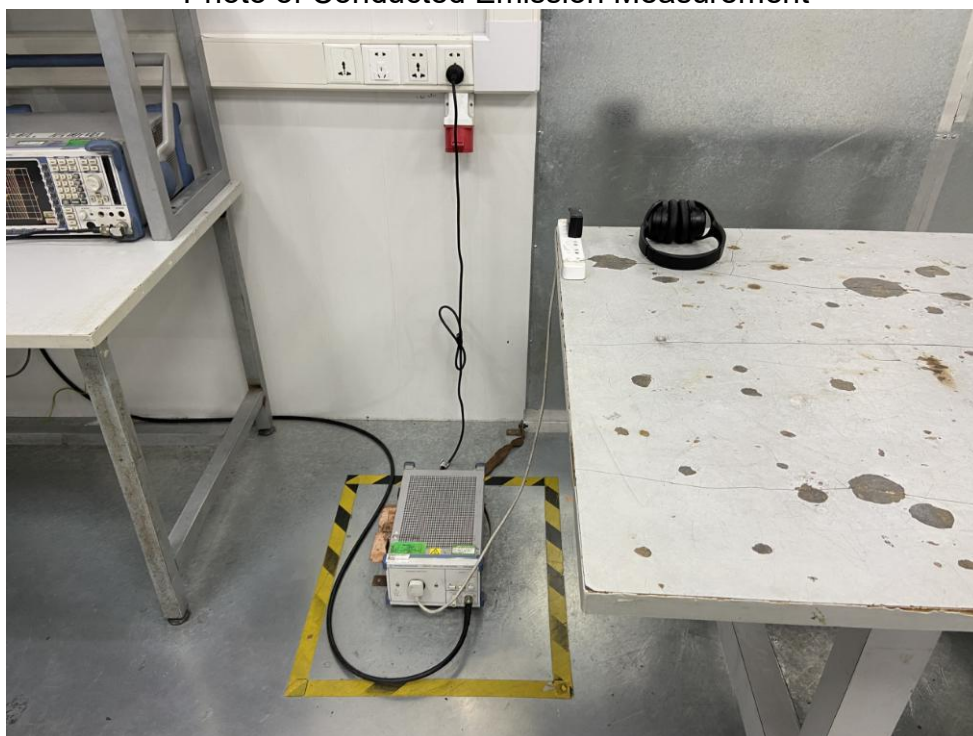
FCC ID: 2AFTU-DD019 Photo of Conducted Emission Measurement
