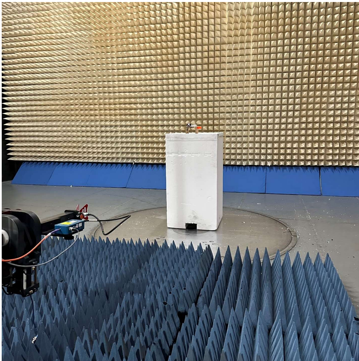
Radiated Emissions, 18GHz – 40GHz
