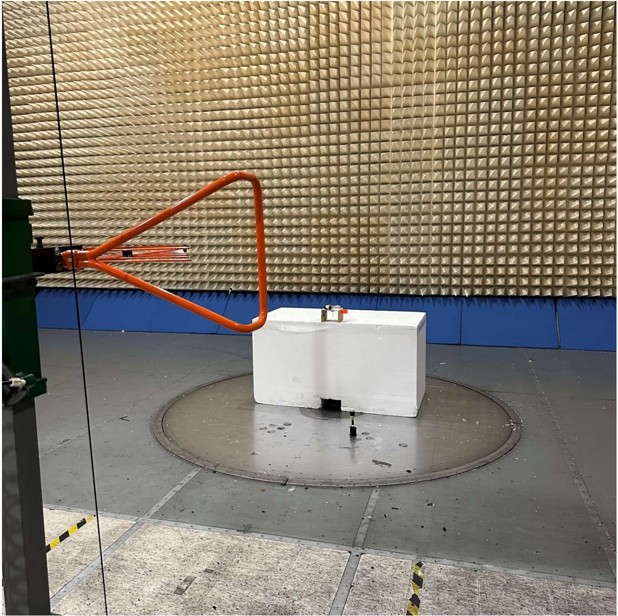
Radiated Emissions, 30MHz – 1GHz
