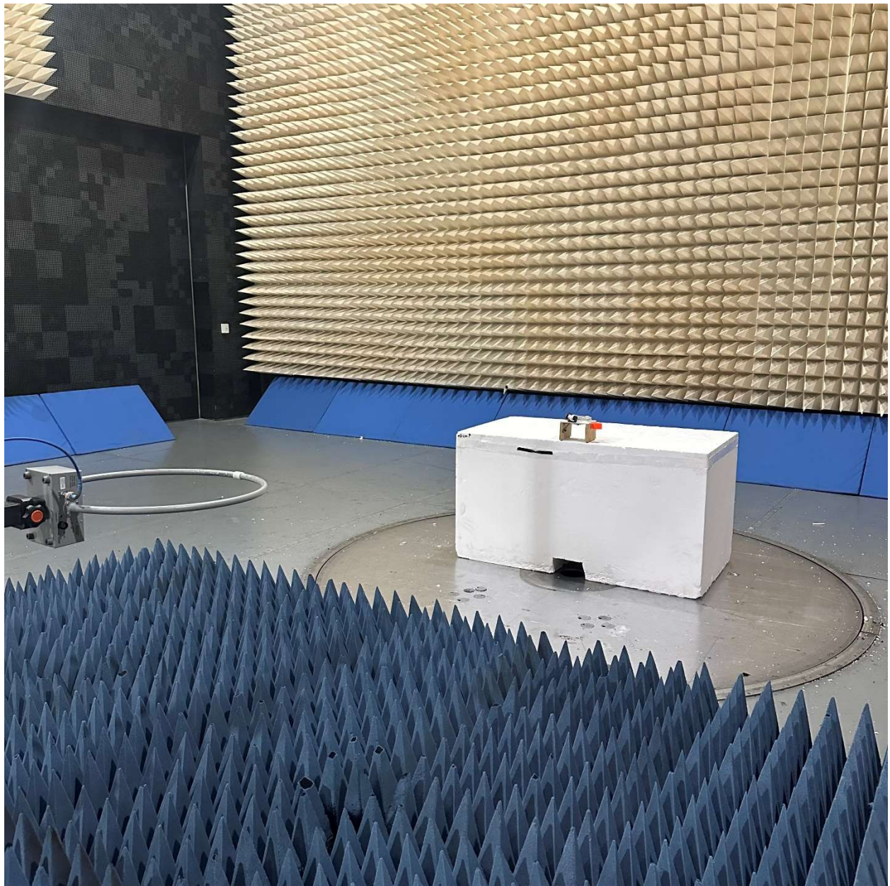
Radiated Emissions, 10kHz – 30MHz
