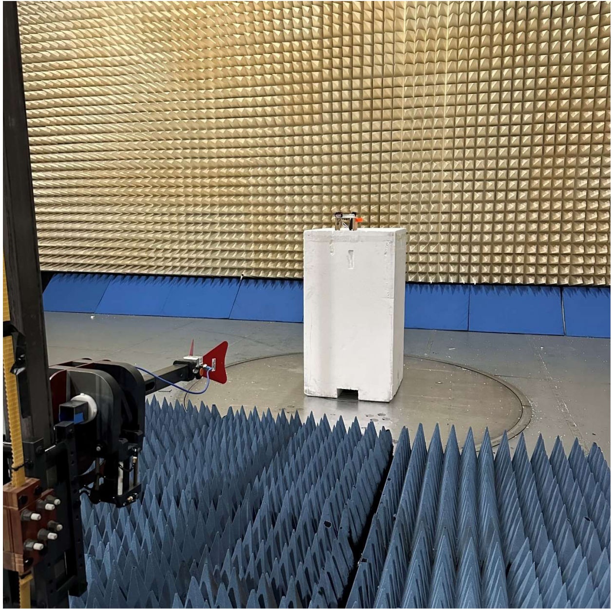
Radiated Emissions, 1GHz – 18GHz
