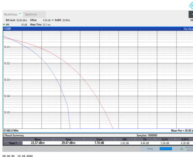
Band71-20MHz-QPSK-133322-100RB#0
