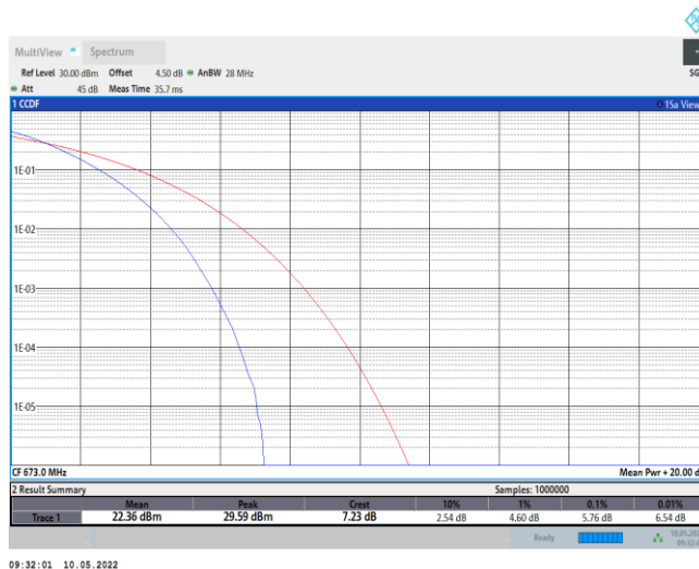
Band71-20MHz-QPSK-133322-100RB#0
