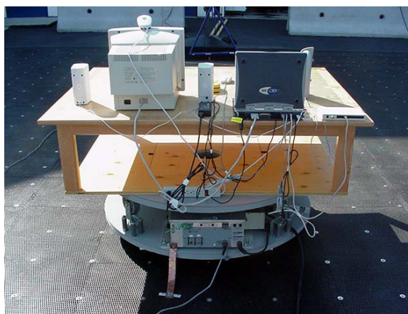
Photograph F-3 - Back of Radiated Emission Configuration
