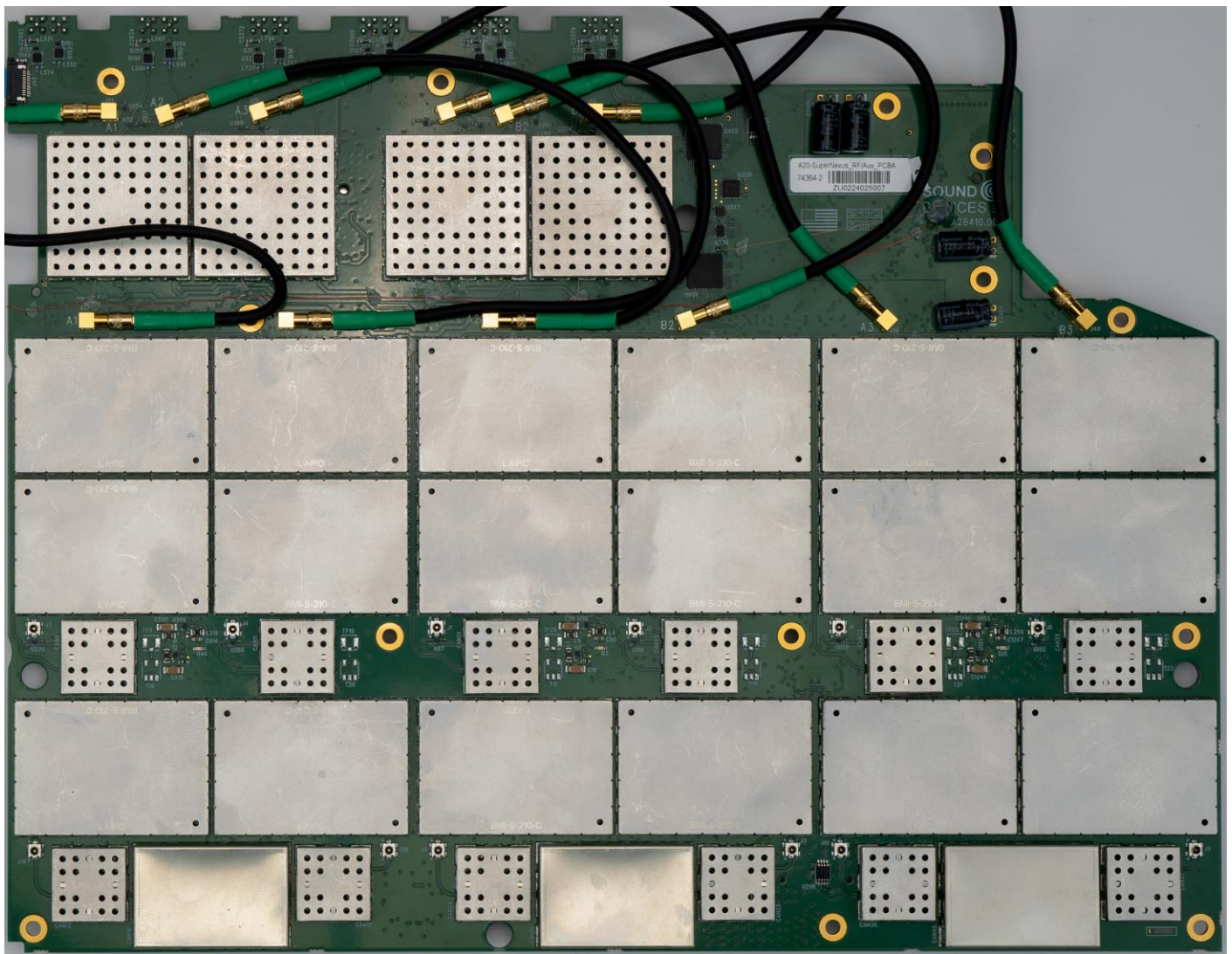
PCB-RF (TOP)
