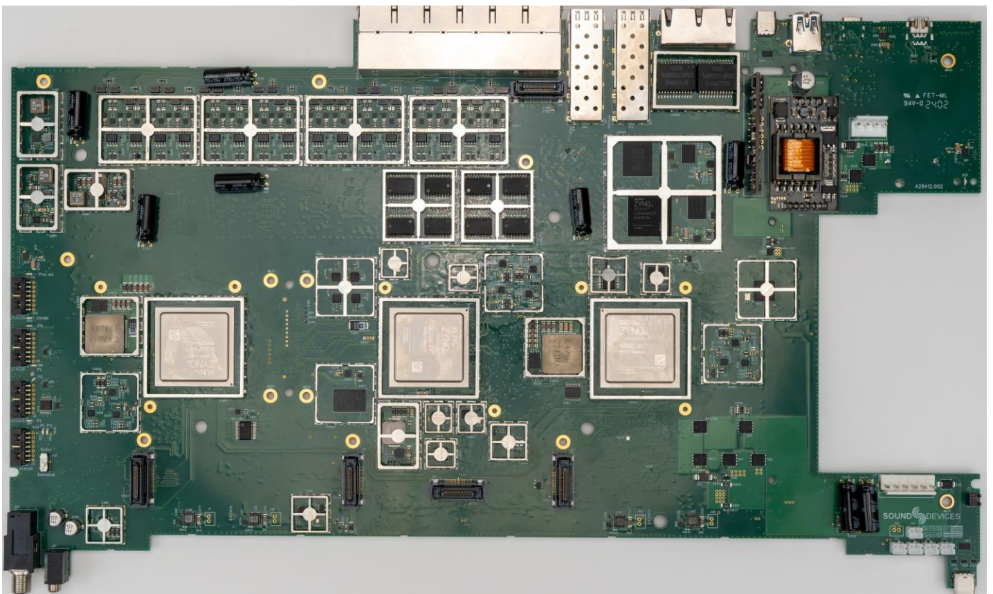
PCB-MAIN (BOTTOM)
