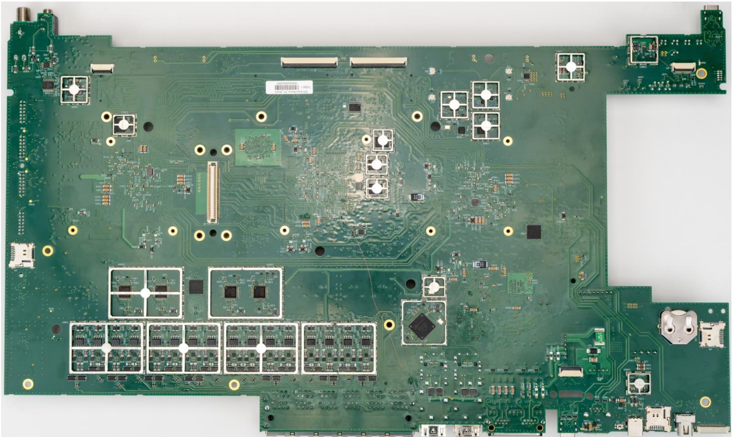
PCB-MAIN (BOTTOM-SHIELDS REMOVED)
