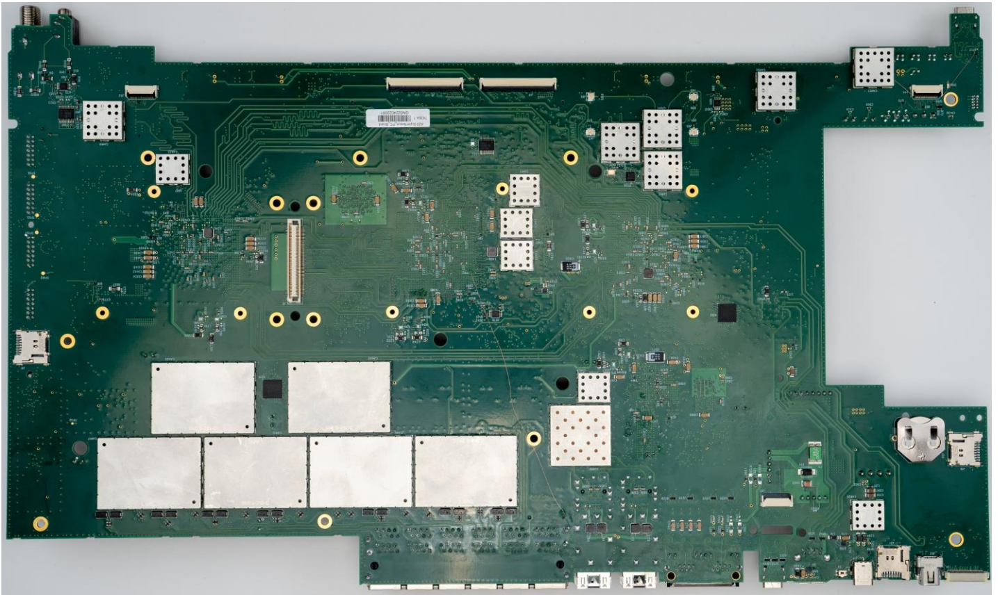
PCB-MAIN (TOP-SHIELDS REMOVED)
