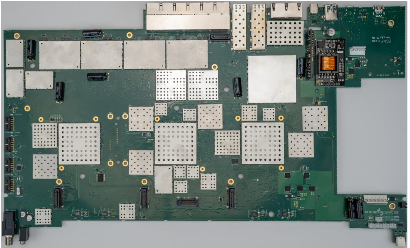
PCB-MAIN (TOP)
