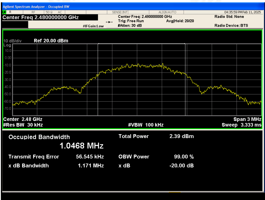
CH39: 2480MHz
