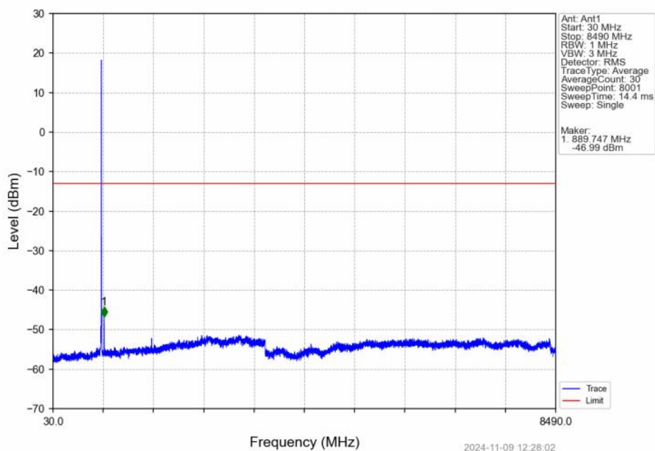
Band5_5MHz_QPSK_HCH_846.5MHz_RB_1_0_NTNV
