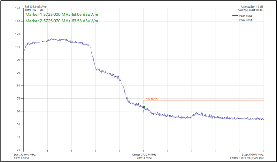
Figure 473 - 802.11ax HE20, SU, TxBF, Core 0 - Core 1 - 5700 MHz Band Edge Frequency 5725 MHz
