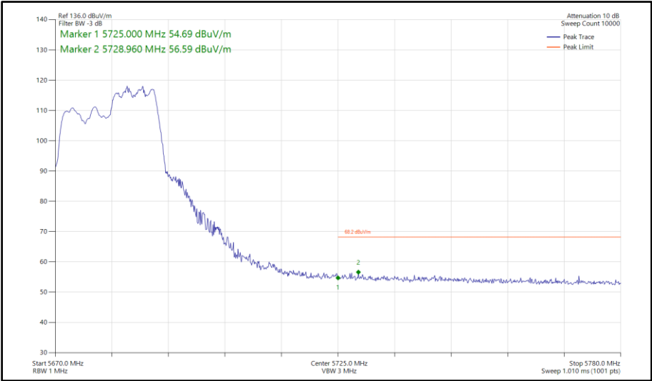
Figure 430 - 802.11ax HE20, RU 106-54, CDD, Core 0 - Core 1 - 5680 MHz Band Edge Frequency 5725 MHz
