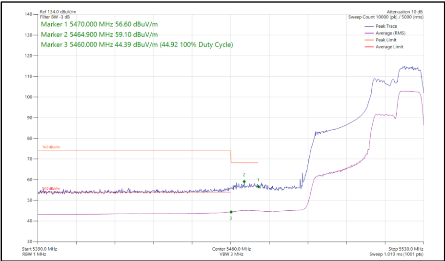
Figure 483 - 802.11ax HE40, RU 106-56, SISO, Core 0 - 5510 MHz Band Edge Frequency 5470 MHz
