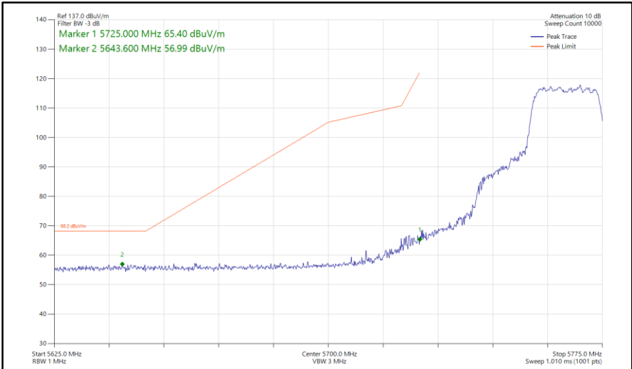
Figure 423 - 802.11n HT20, CDD, Core 0 - Core 1 - 5765 MHz Band Edge Frequency 5725 MHz
