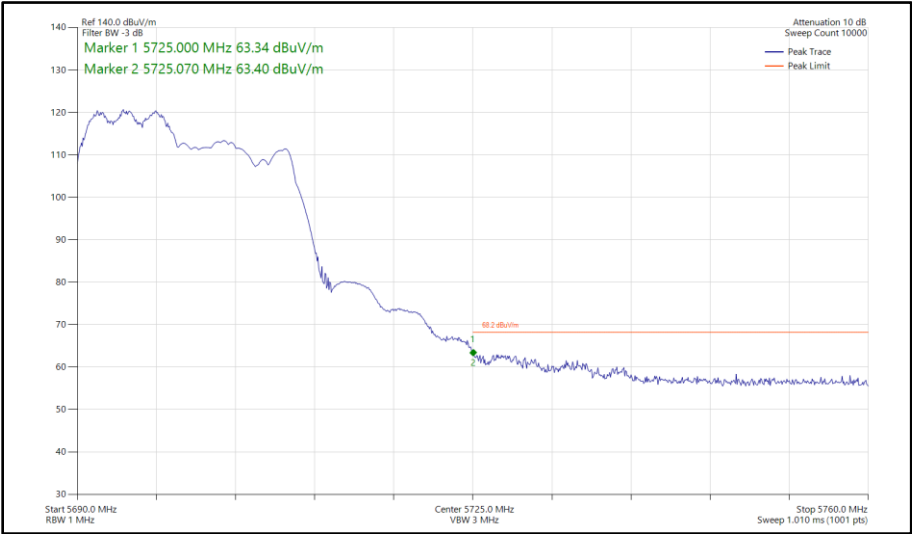
Figure 432 - 802.11ax HE20, RU 106-53, CDD, Core 0 - Core 1 - 5700 MHz Band Edge Frequency 5725 MHz
