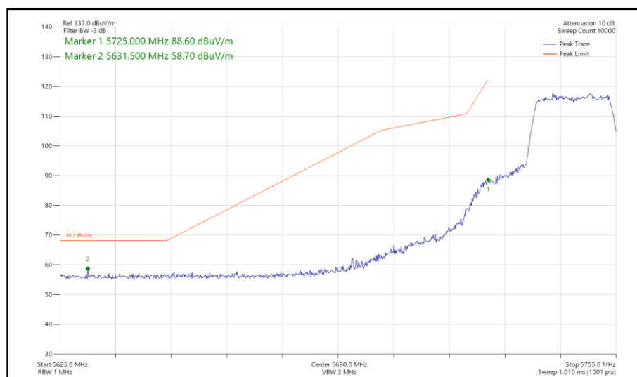
Figure 446 - 802.11n HT20, SDM, Core 0 - Core 1 - 5745 MHz Band Edge Frequency 5725 MHz
