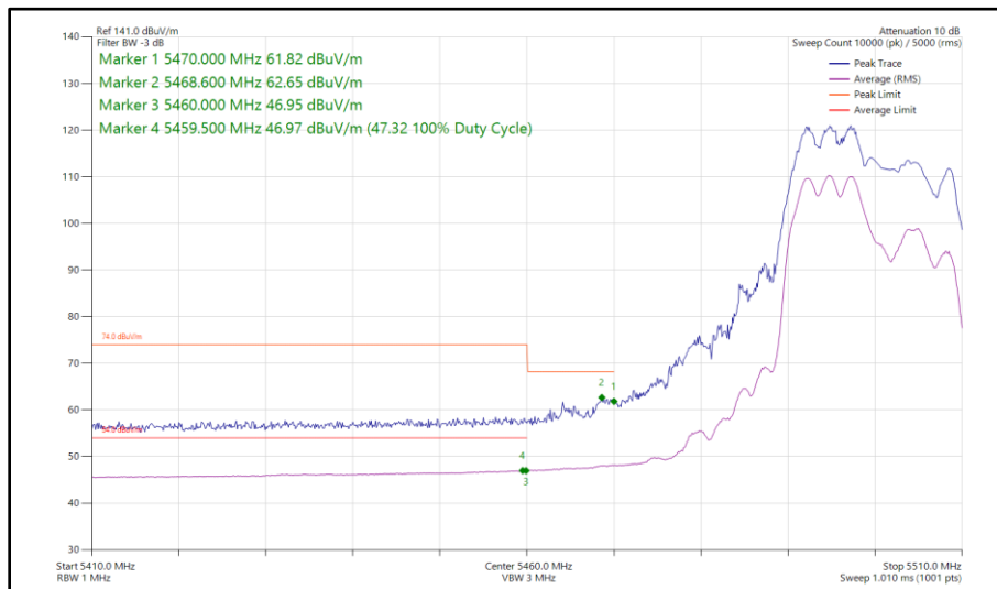
Figure 419 - 802.11ax HE20, RU 106-53, CDD, Core 0 - Core 1 - 5500 MHz Band Edge Frequency 5470 MHz
