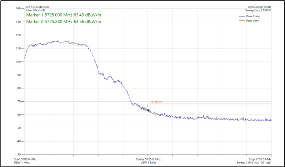
Figure 428 - 802.11n HT20, CDD, Core 0 - Core 1 - 5700 MHz Band Edge Frequency 5725 MHz
