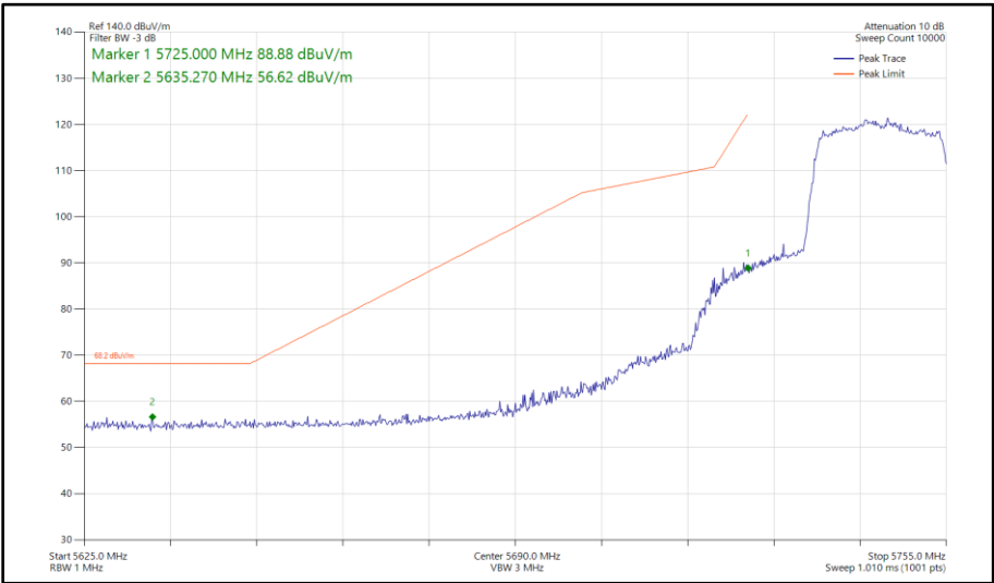
Figure 468 - 802.11ax HE20, SU, TxBF, Core 0 - Core 1 - 5745 MHz Band Edge Frequency 5725 MHz
