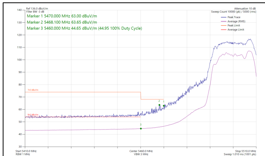
Figure 462 - 802.11ac VHT20, TxBF, Core 0 - Core 1 - 5500 MHz Band Edge Frequency 5470 MHz
