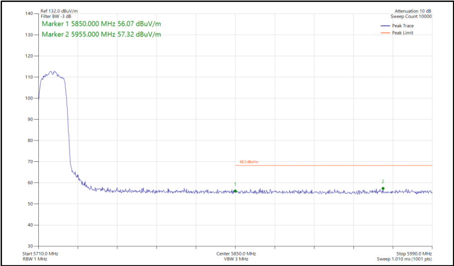
Figure 455 - 802.11n HT20, SDM, Core 0 - Core 1 - 5720 MHz Band Edge Frequency 5850 MHz
