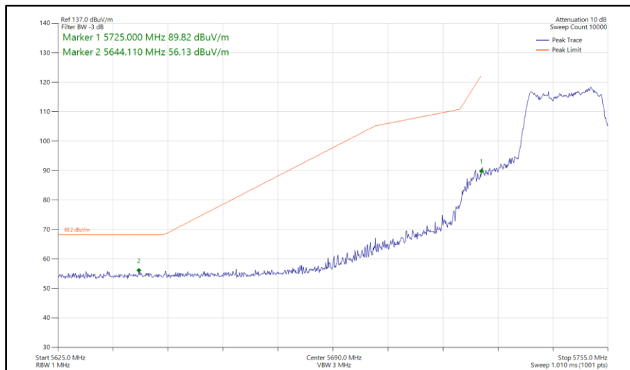
Figure 466 - 802.11ac VHT20, TxBF, Core 0 - Core 1 - 5745 MHz Band Edge Frequency 5725 MHz
