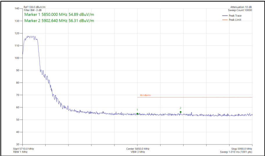
Figure 433 - 802.11n HT20, CDD, Core 0 - Core 1 - 5720 MHz Band Edge Frequency 5850 MHz
