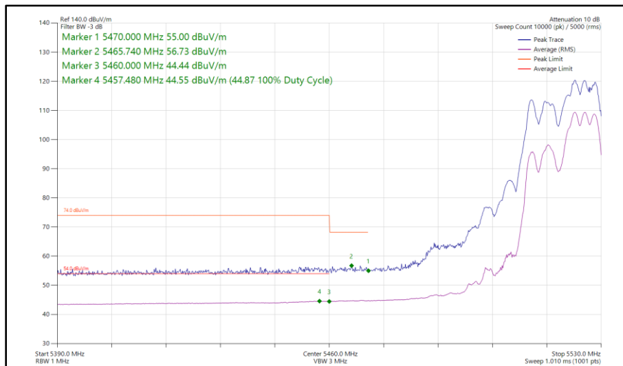
Figure 421 - 802.11ax HE20, RU 106-54, CDD, Core 0 - Core 1 - 5520 MHz Band Edge Frequency 5470 MHz
