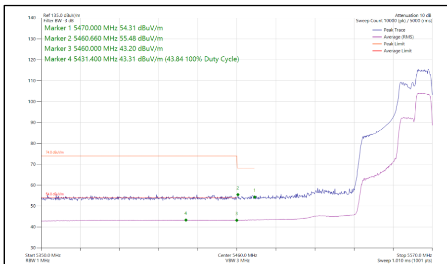
Figure 485 - 802.11ax HE40, RU 106-56, SISO, Core 0 - 5550 MHz Band Edge Frequency 5470 MHz
