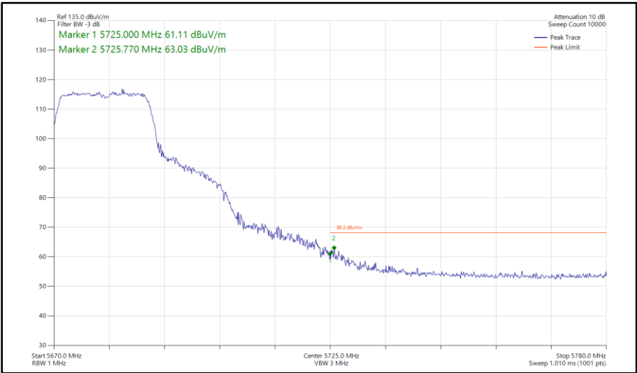
Figure 427 - 802.11n HT20, CDD, Core 0 - Core 1 - 5680 MHz Band Edge Frequency 5725 MHz
