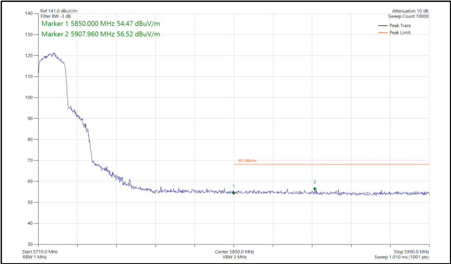
Figure 477 - 802.11ax HE20, SU, TxBF, Core 0 - Core 1 - 5720 MHz Band Edge Frequency 5850 MHz
