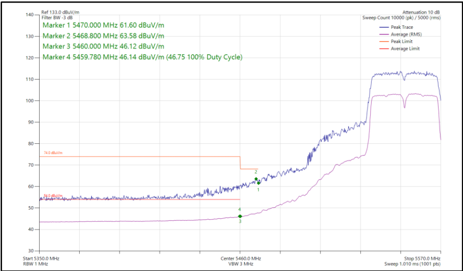
Figure 481 - 802.11n HT40, SISO, Core 0 - 5550 MHz Band Edge Frequency 5470 MHz
