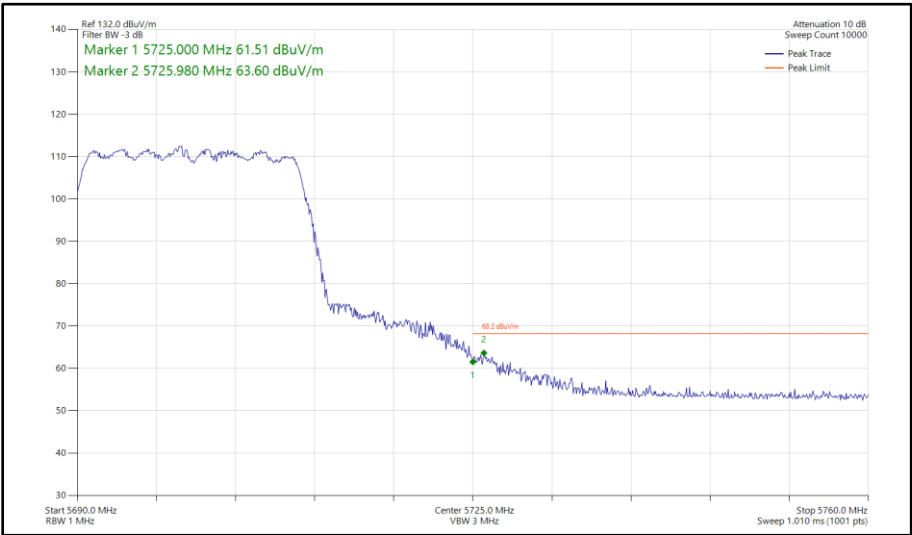
Figure 431 - 802.11ax HE20, SU, CDD, Core 0 - Core 1 - 5700 MHz Band Edge Frequency 5725 MHz
