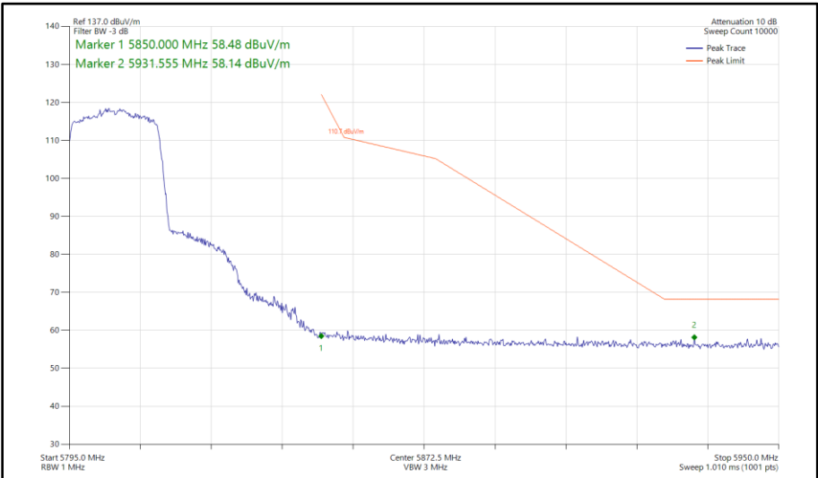
Figure 413 - 802.11ax HE20, SU, SISO, Core 1 - 5805 MHz Band Edge Frequency 5850 MHz
