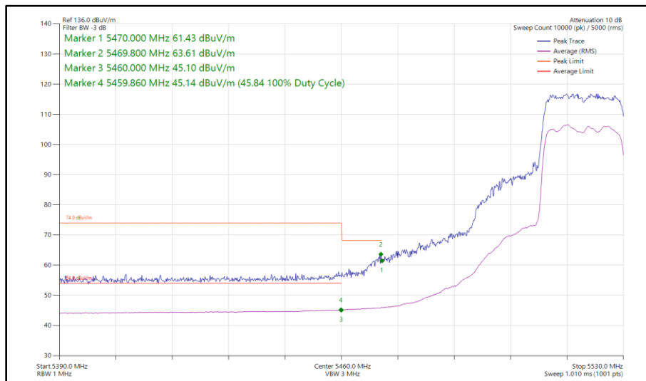
Figure 444 - 802.11ax HE20, SU, SDM, Core 0 - Core 1 - 5520 MHz Band Edge Frequency 5470 MHz
