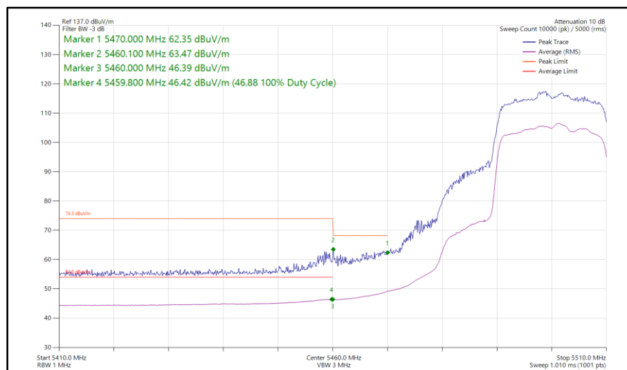
Figure 442 - 802.11ax HE20, SU, SDM, Core 0 - Core 1 - 5500 MHz Band Edge Frequency 5470 MHz
