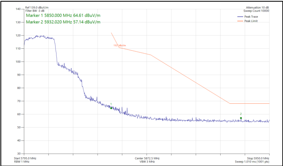
Figure 478 - 802.11ax HE20, SU, TxBF, Core 0 - Core 1 - 5805 MHz Band Edge Frequency 5850 MHz
