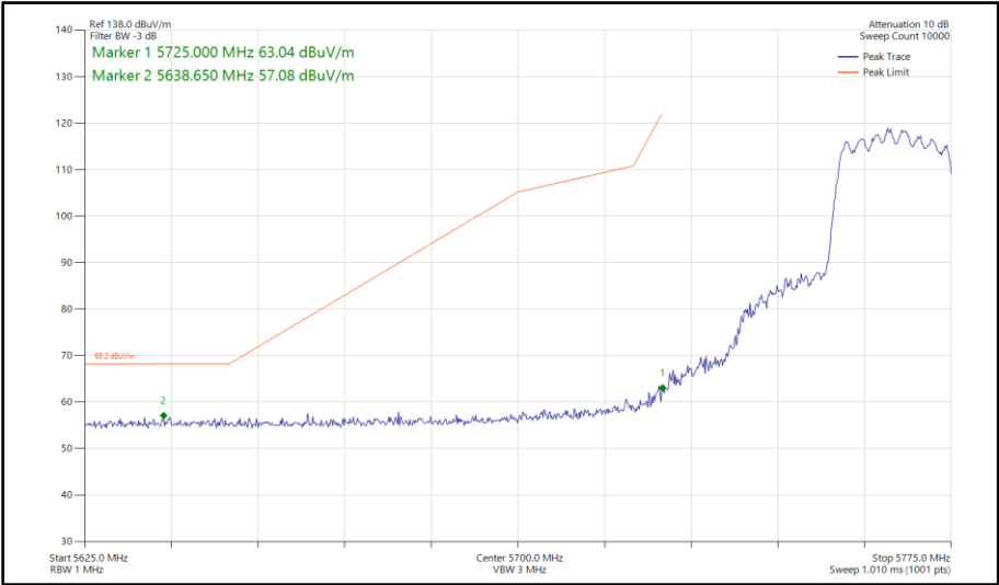
Figure 426 - 802.11ax HE20, SU, CDD, Core 0 - Core 1 - 5765 MHz Band Edge Frequency 5725 MHz
