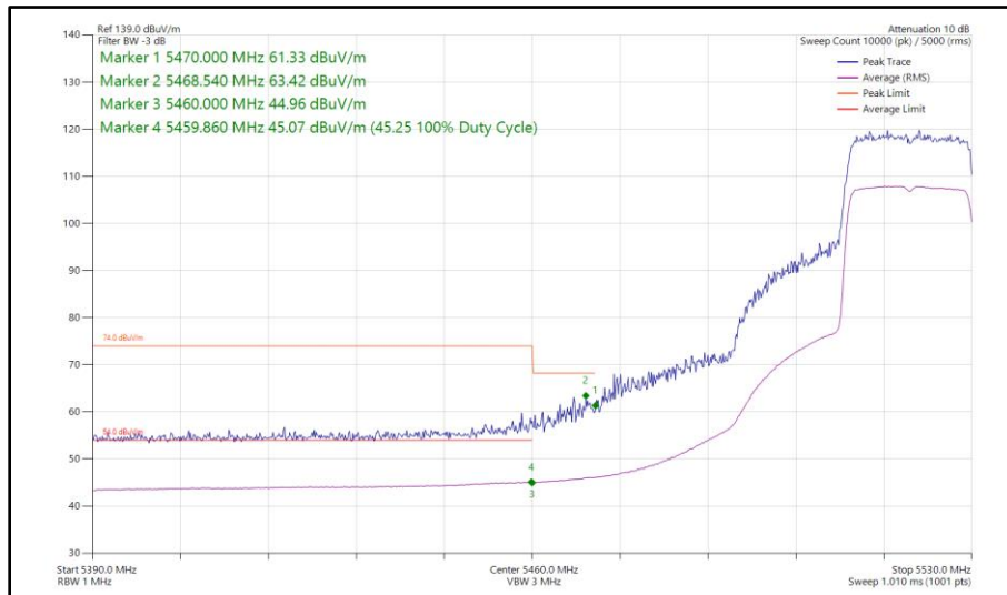
Figure 465 - 802.11ax HE20, SU, TxBF, Core 0 - Core 1 - 5520 MHz Band Edge Frequency 5470 MHz
