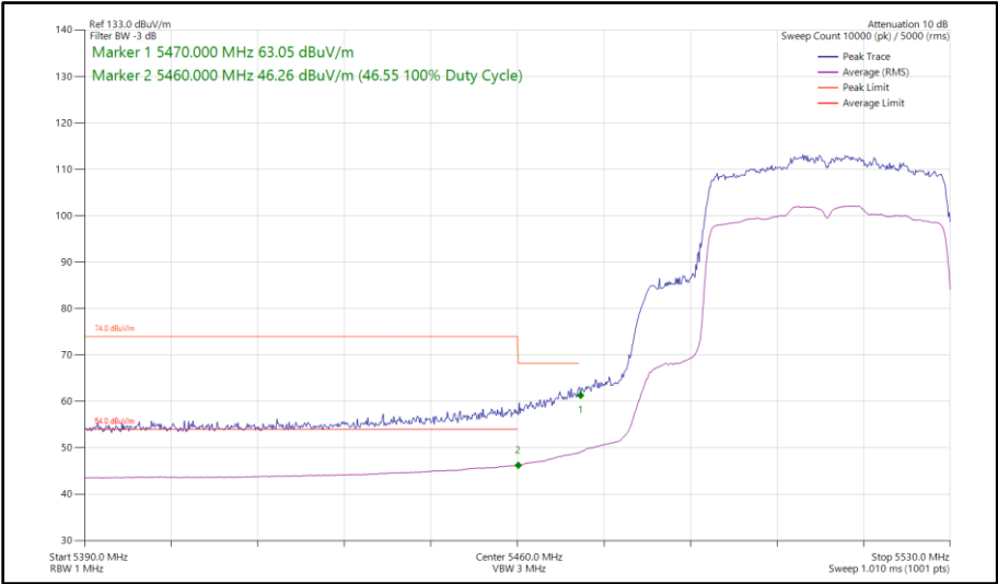
Figure 482 - 802.11ax HE40, SU, SISO, Core 0 - 5510 MHz Band Edge Frequency 5470 MHz
