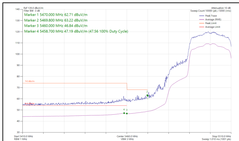
Figure 464 - 802.11ax HE20, SU, TxBF, Core 0 - Core 1 - 5500 MHz Band Edge Frequency 5470 MHz
