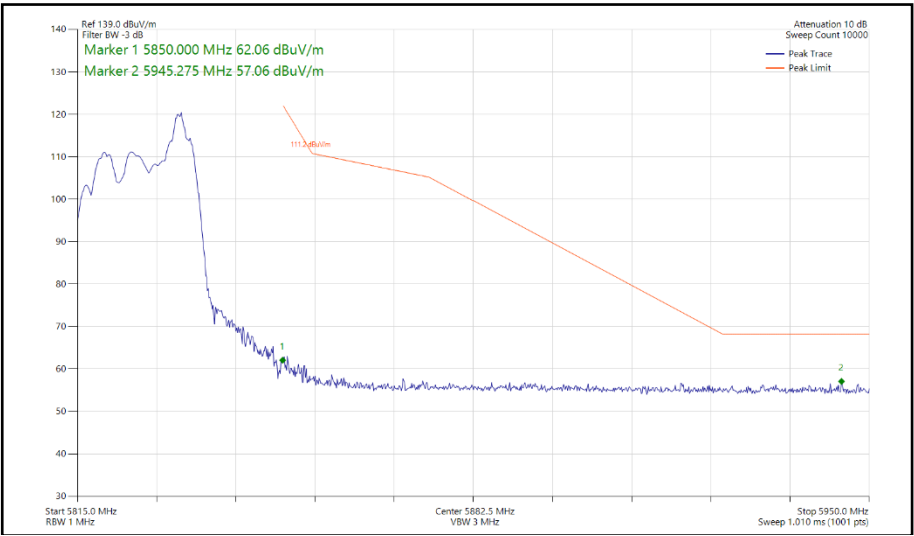
Figure 440 - 802.11ax HE20, RU 52-40, CDD, Core 0 - Core 1 - 5825 MHz Band Edge Frequency 5850 MHz
