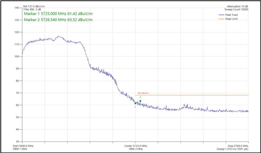
Figure 471 - 802.11ac VHT20, TxBF, Core 0 - Core 1 - 5700 MHz Band Edge Frequency 5725 MHz
