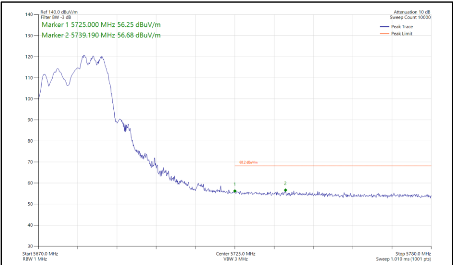
Figure 452 - 802.11ax HE20, RU 106-54, SDM, Core 0 - Core 1 - 5680 MHz Band Edge Frequency 5725 MHz
