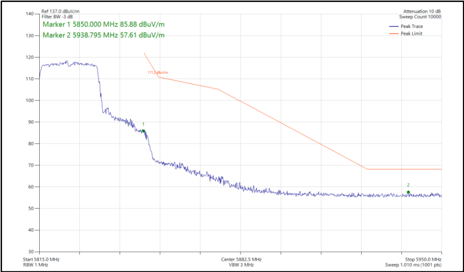
Figure 414 - 802.11ax HE20, SU, SISO, Core 1 - 5825 MHz Band Edge Frequency 5850 MHz
