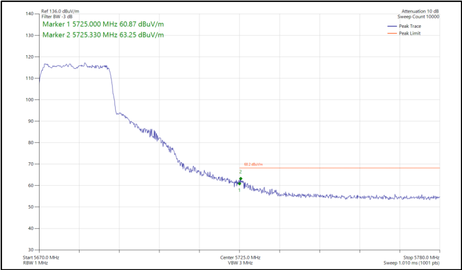
Figure 451 - 802.11ax HE20, SU, SDM, Core 0 - Core 1 - 5680 MHz Band Edge Frequency 5725 MHz
