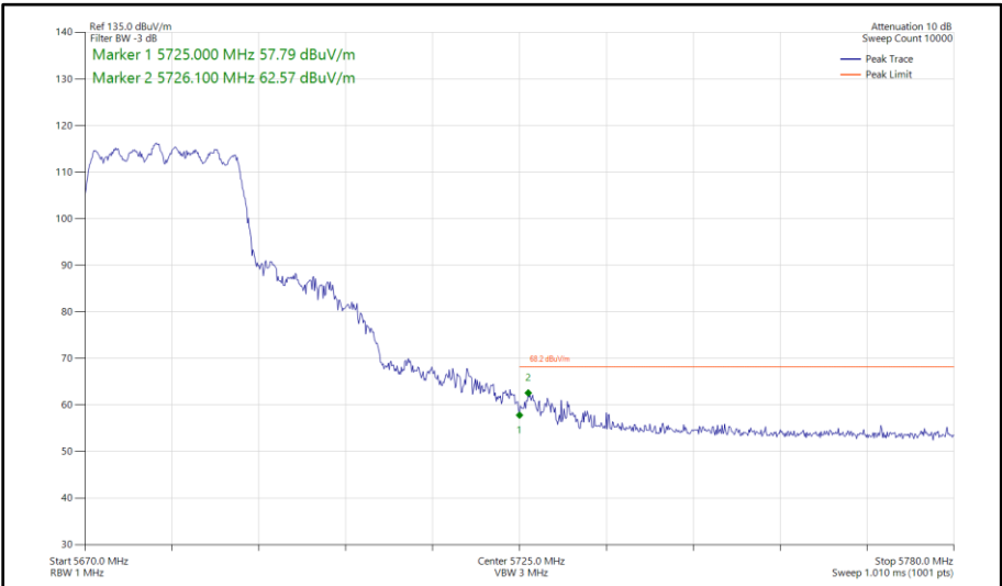
Figure 429 - 802.11ax HE20, SU, CDD, Core 0 - Core 1 - 5680 MHz Band Edge Frequency 5725 MHz
