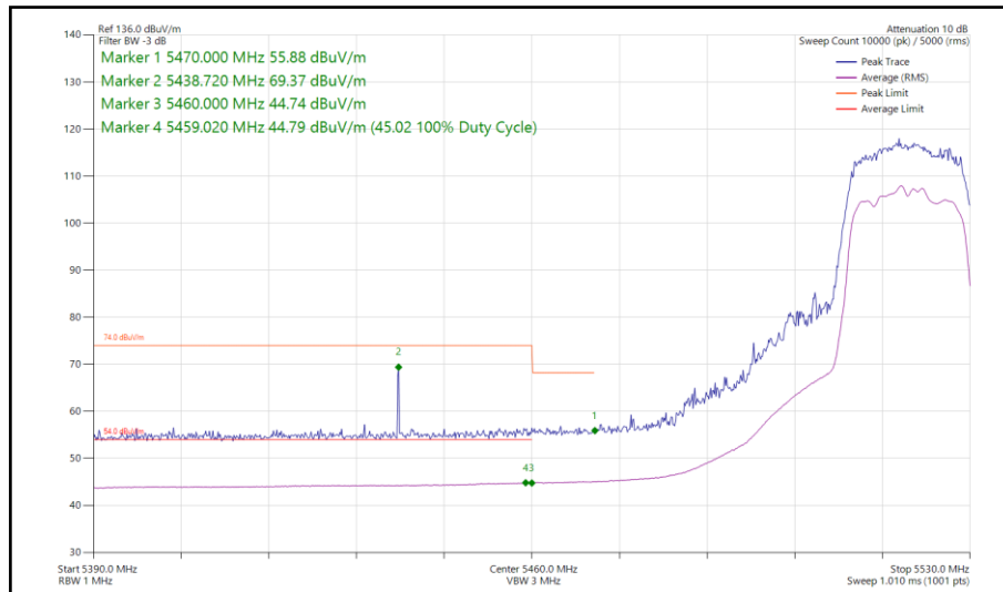
Figure 463 - 802.11ac VHT20, TxBF, Core 0 - Core 1 - 5520 MHz Band Edge Frequency 5470 MHz
