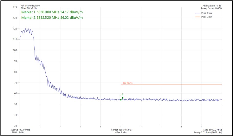
Figure 436 - 802.11ax HE20, SU, CDD, Core 0 - Core 1 - 5720 MHz Band Edge Frequency 5850 MHz
