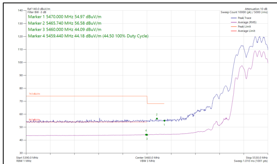
Figure 445 - 802.11ax HE20, RU 106-54, SDM, Core 0 - Core 1 - 5520 MHz Band Edge Frequency 5470 MHz
