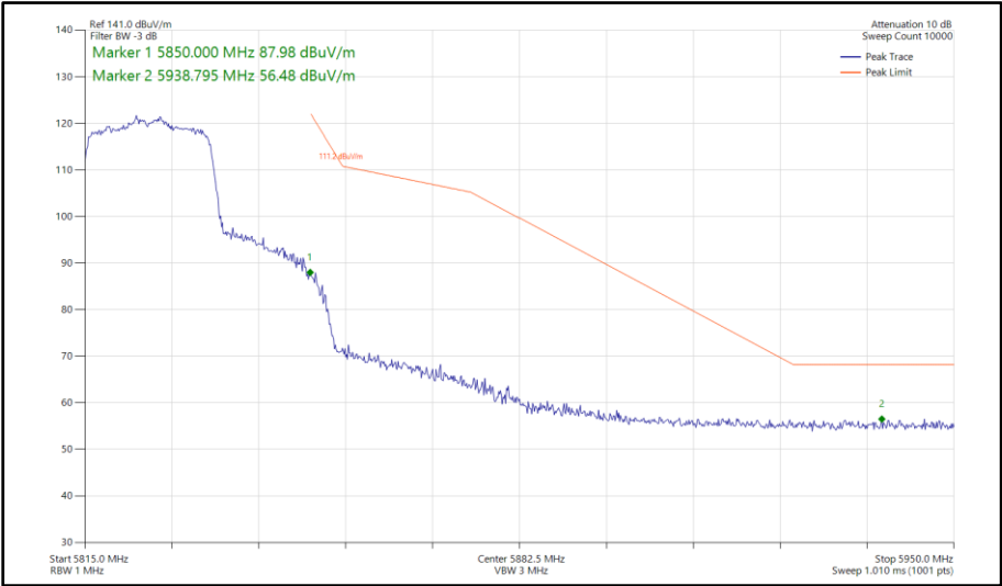
Figure 479 - 802.11ax HE20, SU, TxBF, Core 0 - Core 1 - 5825 MHz Band Edge Frequency 5850 MHz
