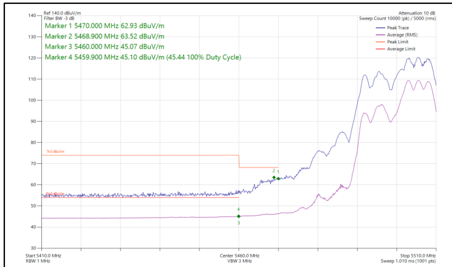
Figure 443 - 802.11ax HE20, RU 106-54, SDM, Core 0 - Core 1 - 5500 MHz Band Edge Frequency 5470 MHz
