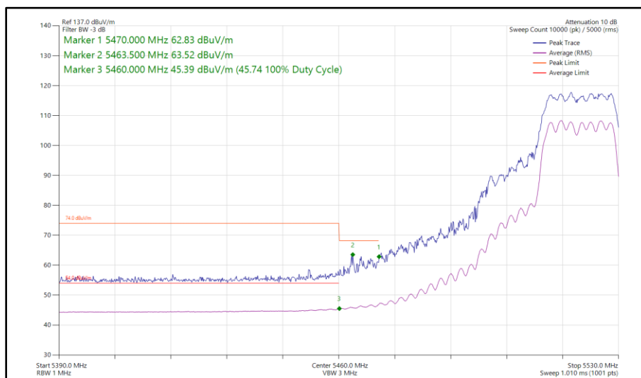
Figure 417 - 802.11n HT20, CDD, Core 0 - Core 1 - 5520 MHz Band Edge Frequency 5470 MHz
