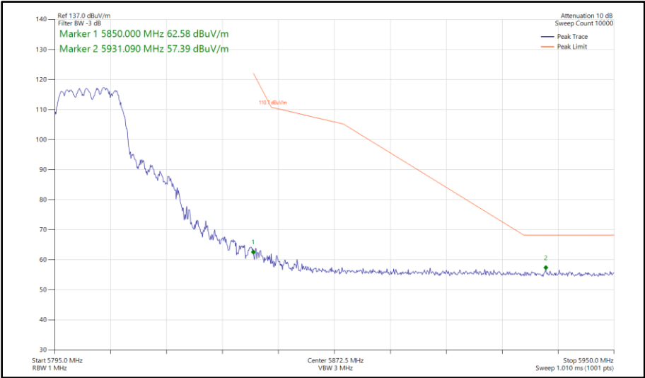
Figure 434 - 802.11n HT20, CDD, Core 0 - Core 1 - 5805 MHz Band Edge Frequency 5850 MHz
