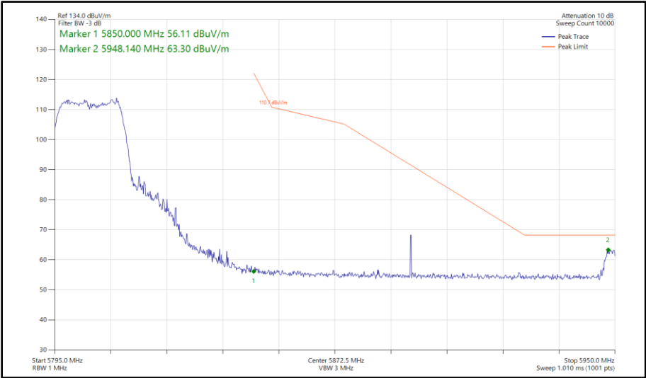
Figure 475 - 802.11ac VHT20, TxBF, Core 0 - Core 1 - 5805 MHz Band Edge Frequency 5850 MHz
