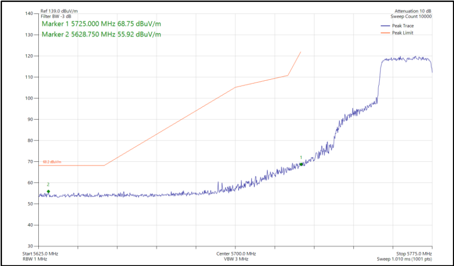
Figure 469 - 802.11ax HE20, SU, TxBF, Core 0 - Core 1 - 5765 MHz Band Edge Frequency 5725 MHz
