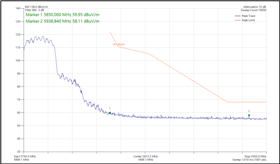
Figure 438 - 802.11ax HE20, SU, CDD, Core 0 - Core 1 - 5805 MHz Band Edge Frequency 5850 MHz
