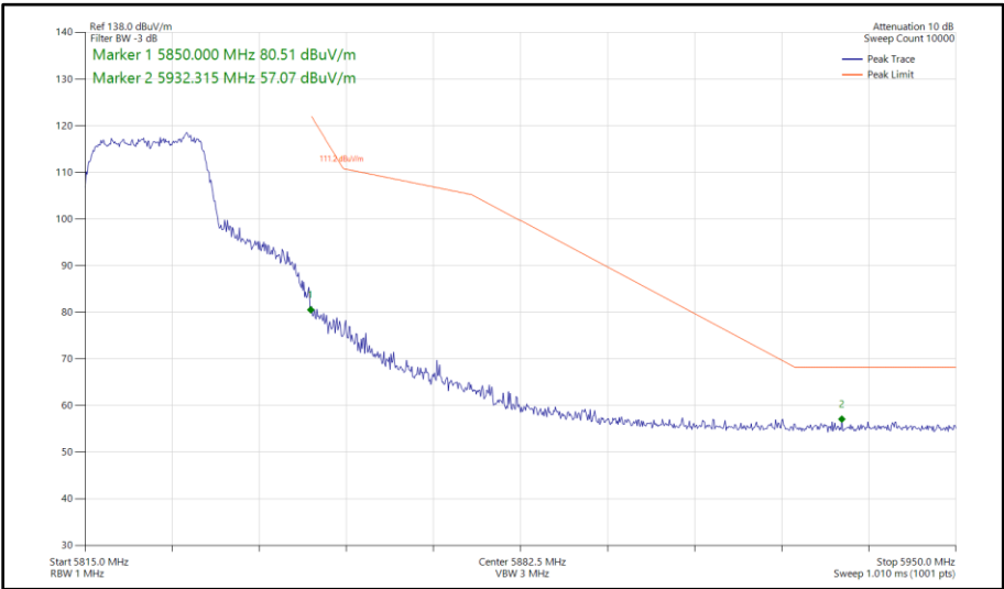
Figure 476 - 802.11ac VHT20, TxBF, Core 0 - Core 1 - 5825 MHz Band Edge Frequency 5850 MHz
