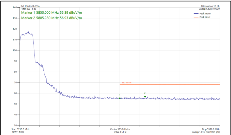
Figure 474 - 802.11ac VHT20, TxBF, Core 0 - Core 1 - 5720 MHz Band Edge Frequency 5850 MHz
