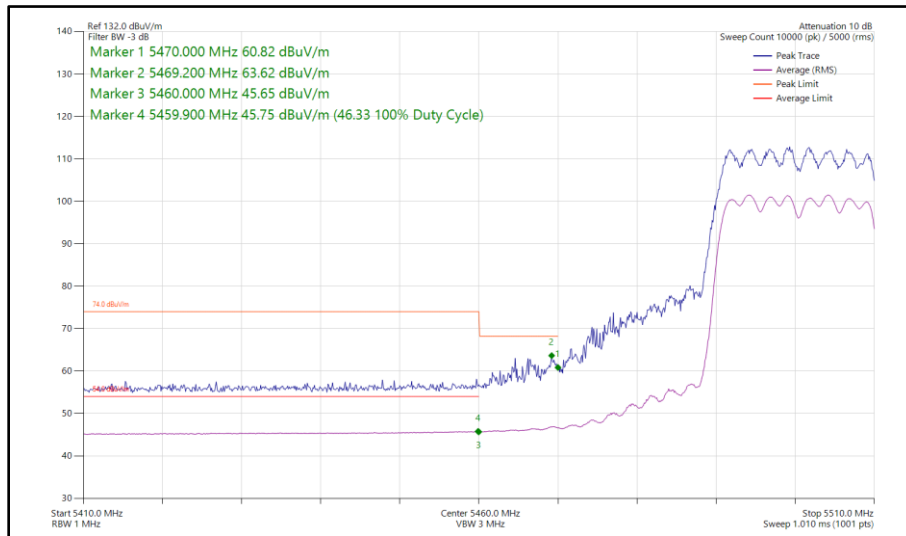
Figure 418 - 802.11ax HE20, SU, CDD, Core 0 - Core 1 - 5500 MHz Band Edge Frequency 5470 MHz
