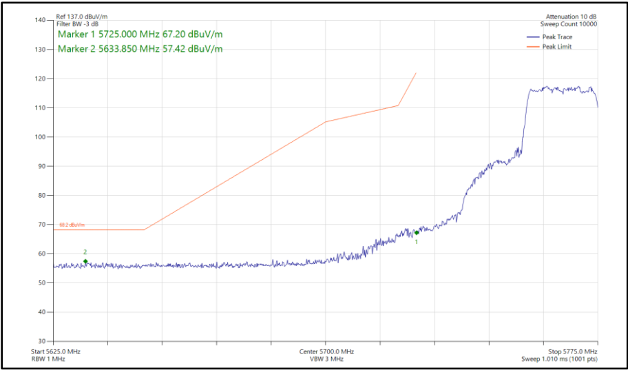
Figure 448 - 802.11ax HE20, SU, SDM, Core 0 - Core 1 - 5765 MHz Band Edge Frequency 5725 MHz
