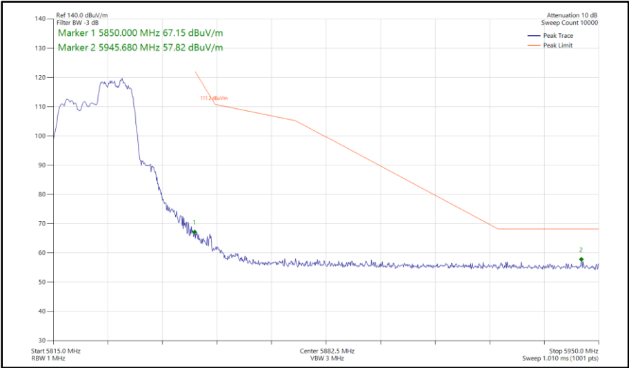
Figure 461 - 802.11ax HE20, RU 106-54, SDM, Core 0 - Core 1 - 5825 MHz Band Edge Frequency 5850 MHz
