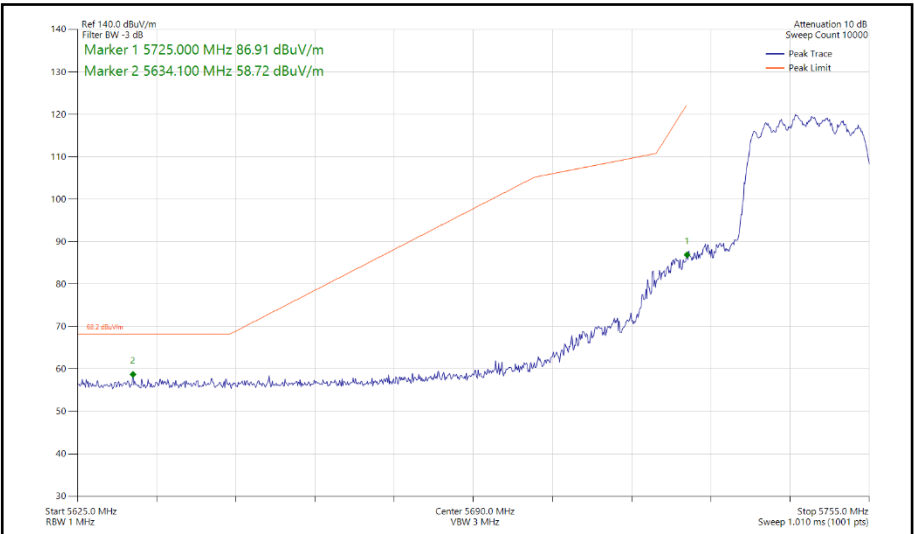
Figure 424 - 802.11ax HE20, SU, CDD, Core 0 - Core 1 - 5745 MHz Band Edge Frequency 5725 MHz
