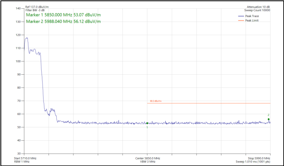
Figure 412 - 802.11ax HE20, RU 52-37, SISO, Core 1 - 5720 MHz Band Edge Frequency 5850 MHz
