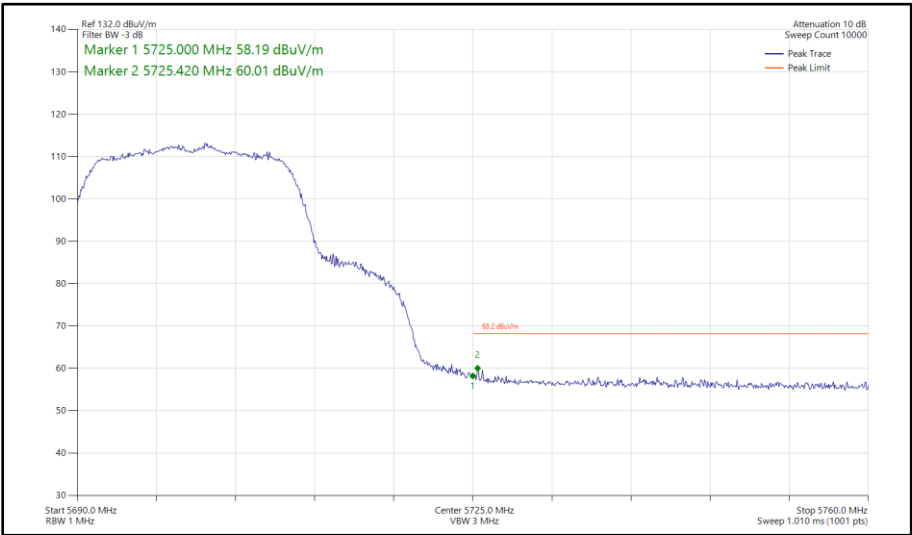
Figure 450 - 802.11n HT20, SDM, Core 0 - Core 1 - 5700 MHz Band Edge Frequency 5725 MHz
