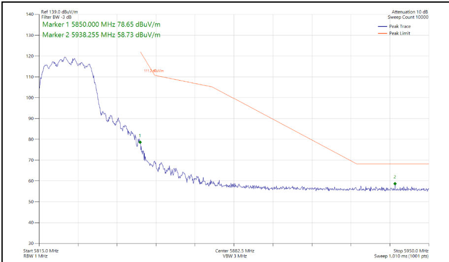
Figure 435 - 802.11n HT20, CDD, Core 0 - Core 1 - 5825 MHz Band Edge Frequency 5850 MHz
