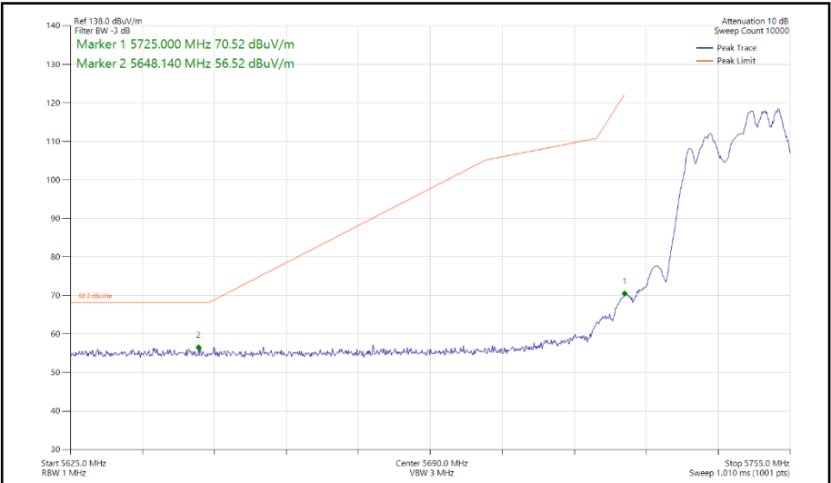
Figure 425 - 802.11ax HE20, RU 106-54, CDD, Core 0 - Core 1 - 5745 MHz Band Edge Frequency 5725 MHz
