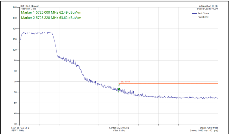
Figure 470 - 802.11ac VHT20, TxBF, Core 0 - Core 1 - 5680 MHz Band Edge Frequency 5725 MHz
