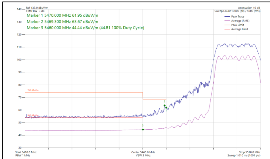
Figure 416 - 802.11n HT20, CDD, Core 0 - Core 1 - 5500 MHz Band Edge Frequency 5470 MHz
