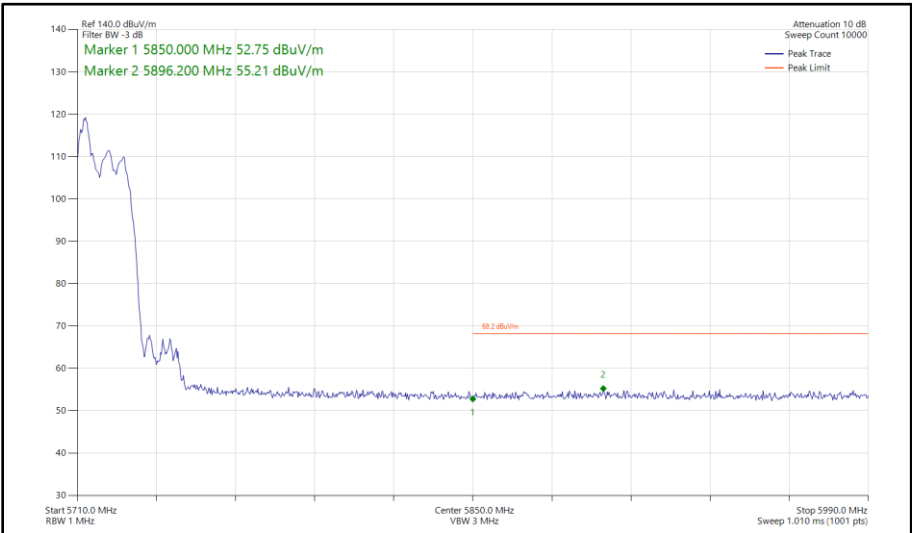
Figure 458 - 802.11ax HE20, RU 52-37, SDM, Core 0 - Core 1 - 5720 MHz Band Edge Frequency 5850 MHz
