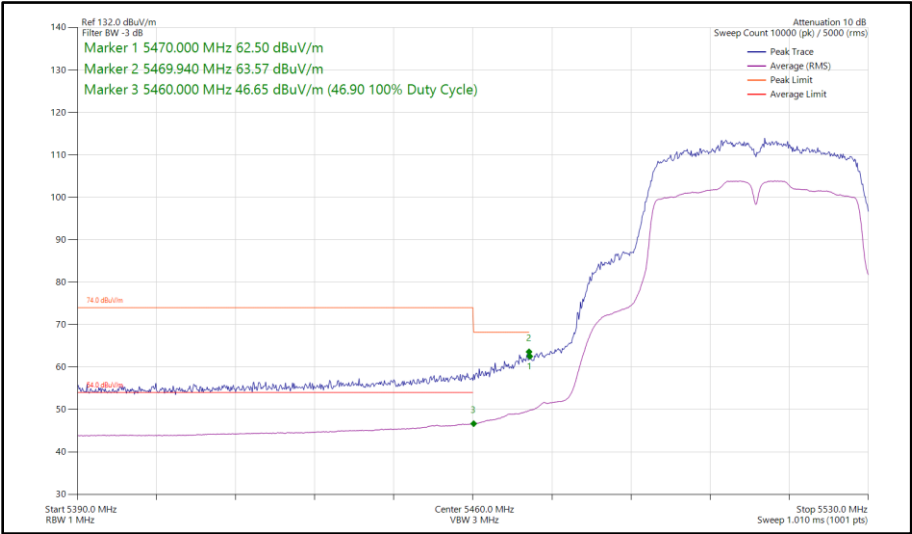
Figure 480 - 802.11n HT40, SISO, Core 0 - 5510 MHz Band Edge Frequency 5470 MHz
