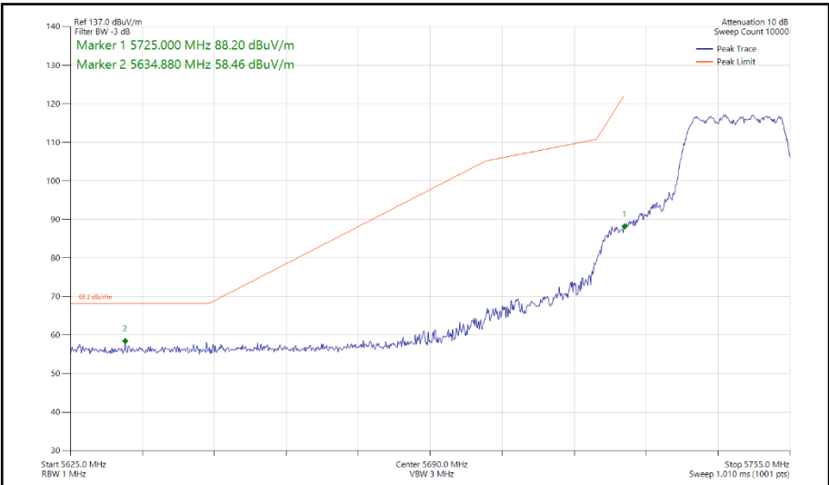
Figure 422 - 802.11n HT20, CDD, Core 0 - Core 1 - 5745 MHz Band Edge Frequency 5725 MHz
