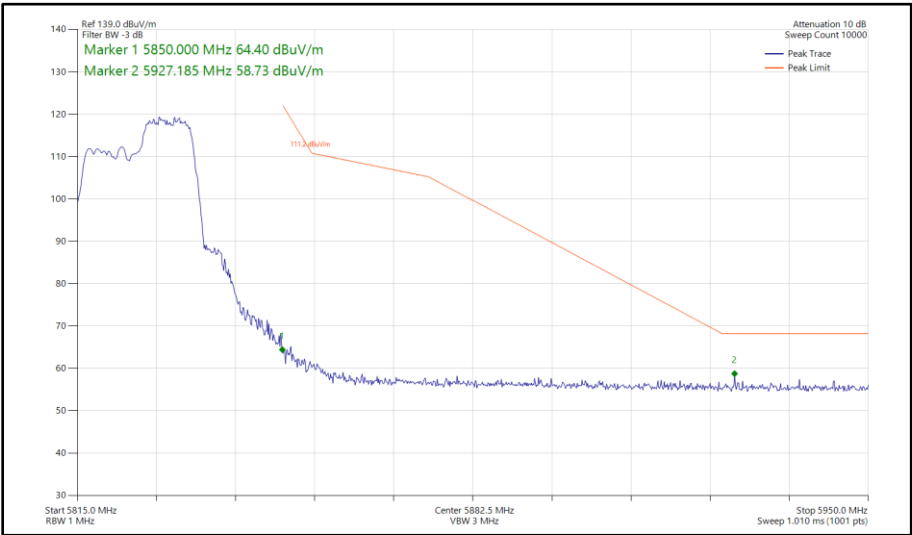
Figure 415 - 802.11ax HE20, RU 106-54, SISO, Core 1 - 5825 MHz Band Edge Frequency 5850 MHz
