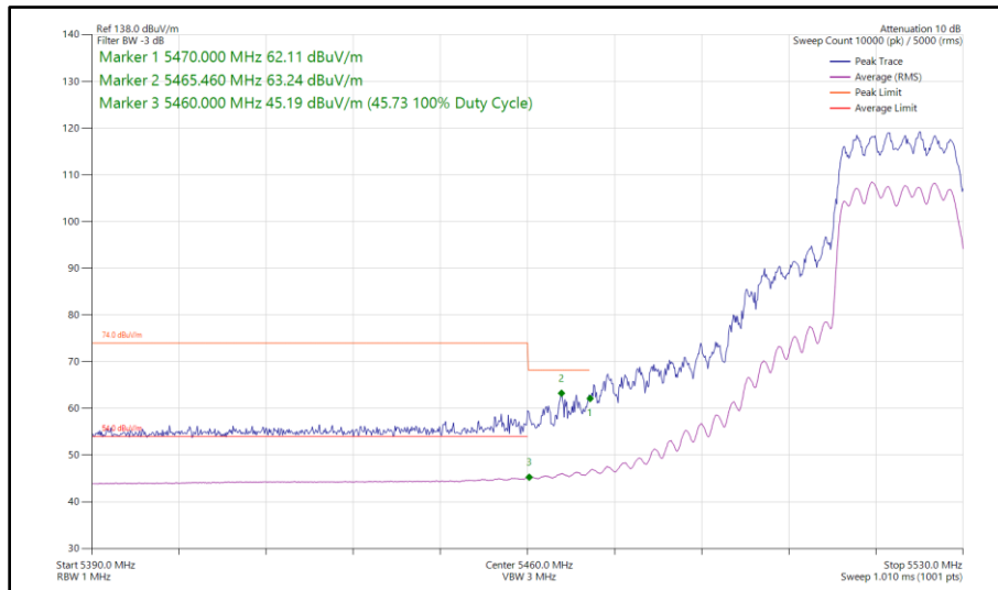
Figure 420 - 802.11ax HE20, SU, CDD, Core 0 - Core 1 - 5520 MHz Band Edge Frequency 5470 MHz
