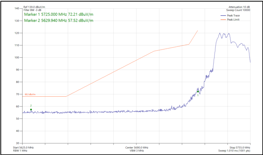
Figure 447 - 802.11ax HE20, RU 106-53, SDM, Core 0 - Core 1 - 5745 MHz Band Edge Frequency 5725 MHz
