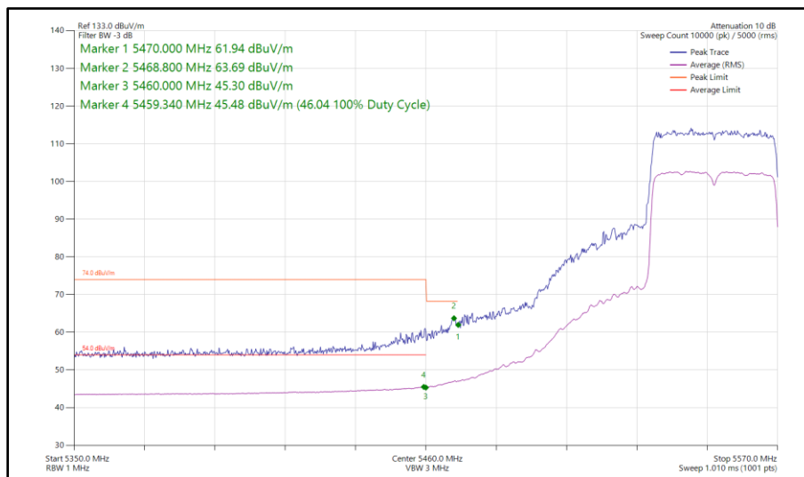
Figure 484 - 802.11ax HE40, SU, SISO, Core 0 - 5550 MHz Band Edge Frequency 5470 MHz
