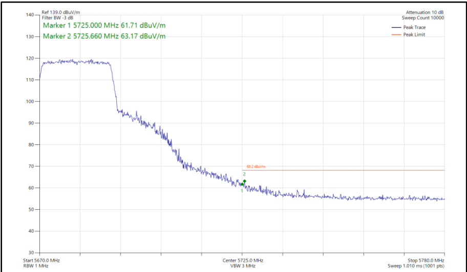
Figure 472 - 802.11ax HE20, SU, TxBF, Core 0 - Core 1 - 5680 MHz Band Edge Frequency 5725 MHz
