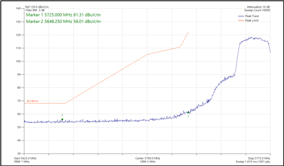
Figure 467 - 802.11ac VHT20, TxBF, Core 0 - Core 1 - 5765 MHz Band Edge Frequency 5725 MHz
