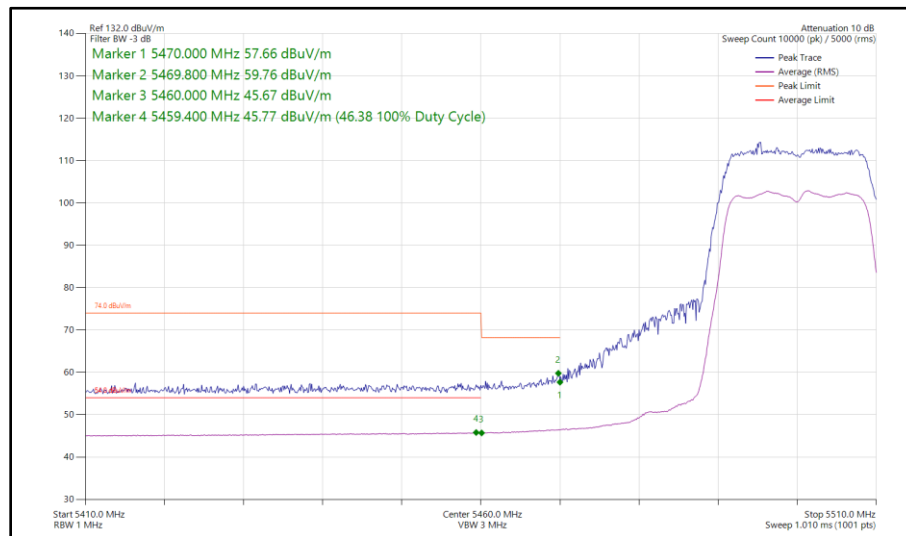
Figure 441 - 802.11n HT20, SDM, Core 0-1 - 5500 MHz Band Edge Frequency 5470 MHz
