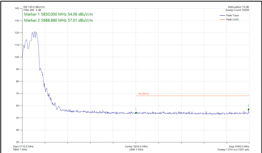
Figure 437 - 802.11ax HE20, RU 106-54, CDD, Core 0 - Core 1 - 5720 MHz Band Edge Frequency 5850 MHz
