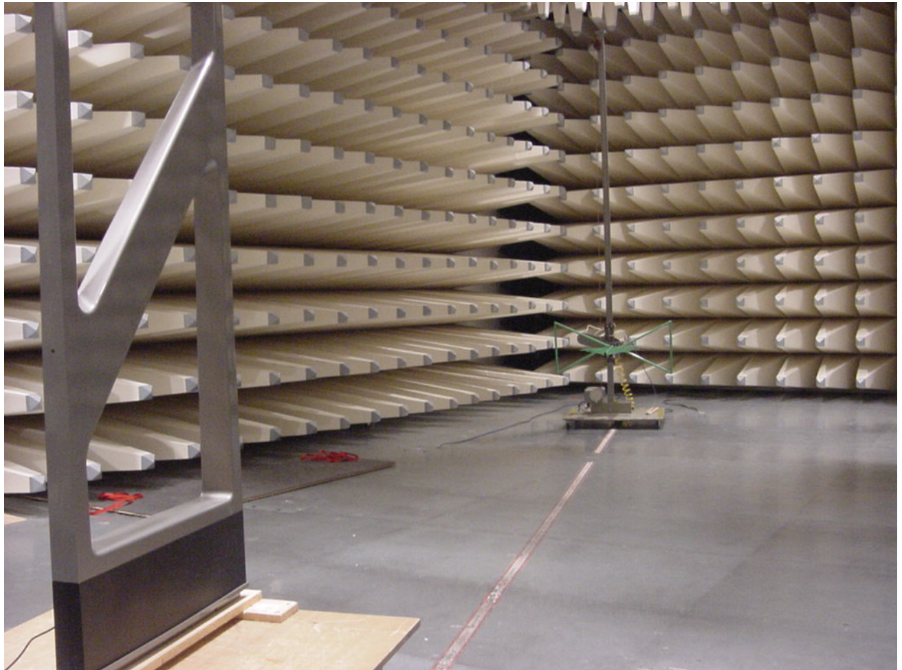
Photo 2 (Radiated Emissions):
