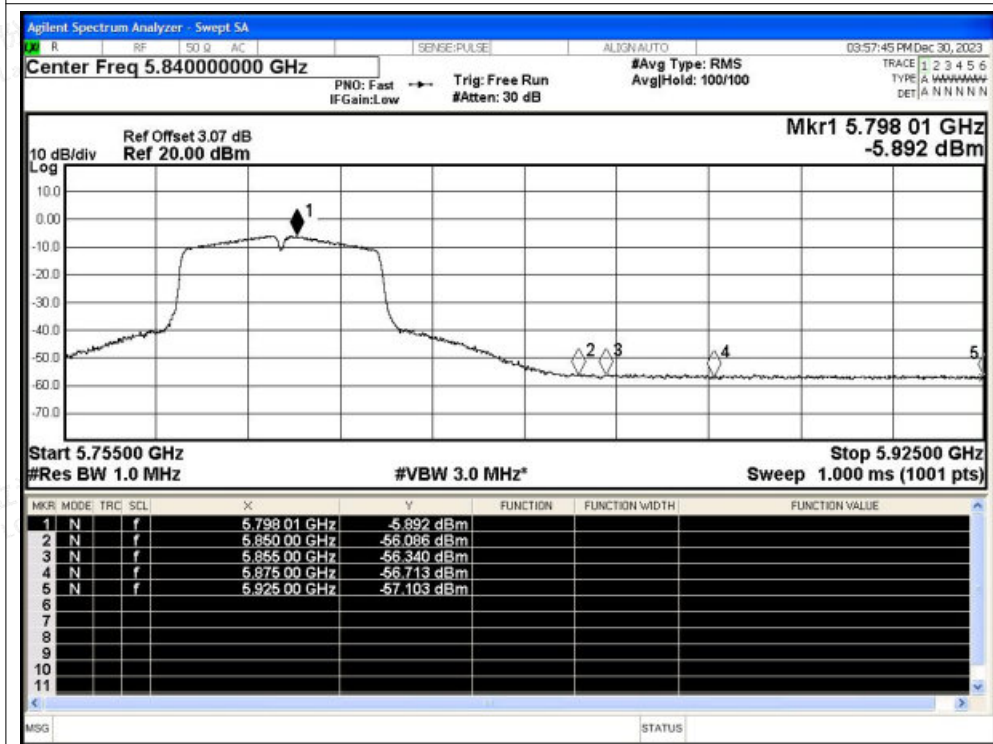
Restrict Band NVNT n40 5795MHz Ant1 Average
