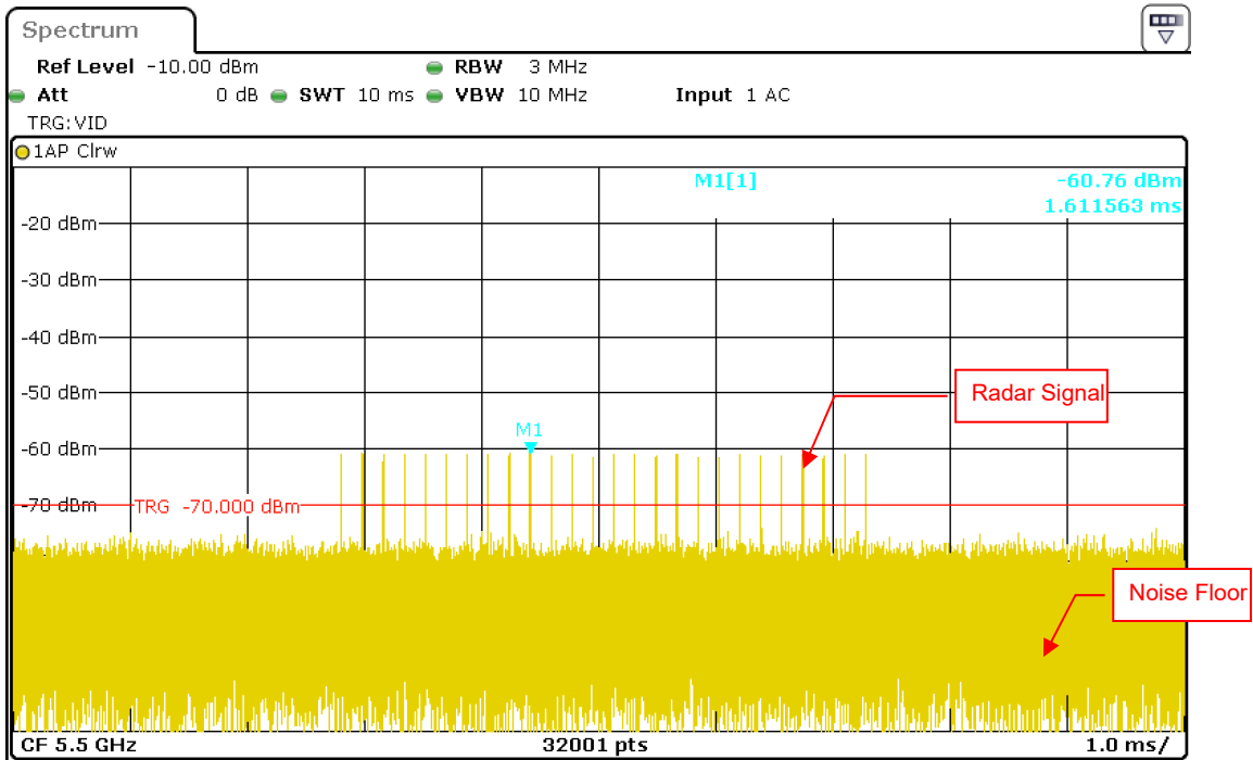
Radar Signal 2
