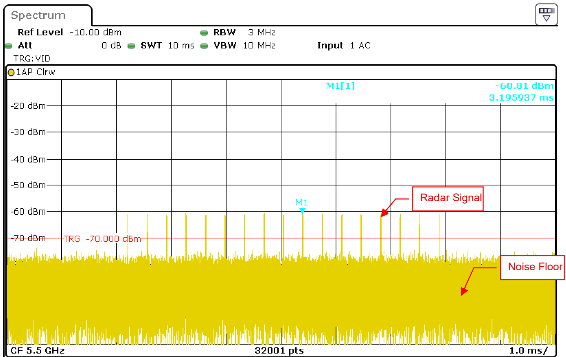
Radar Signal 3
