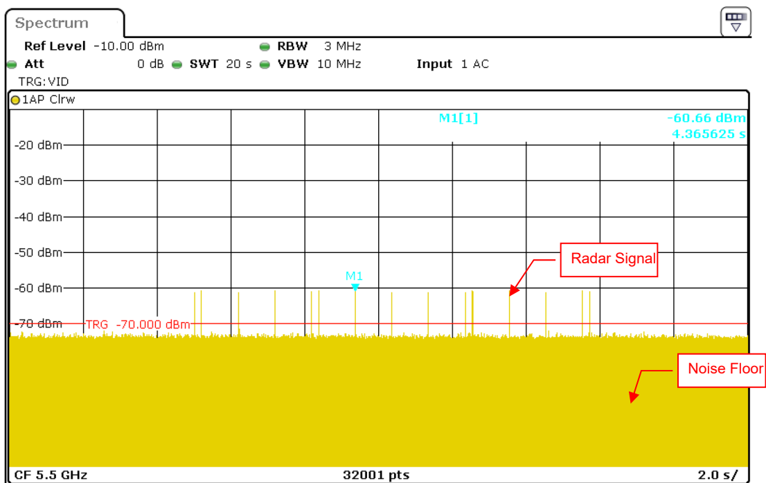
Radar Signal 5
