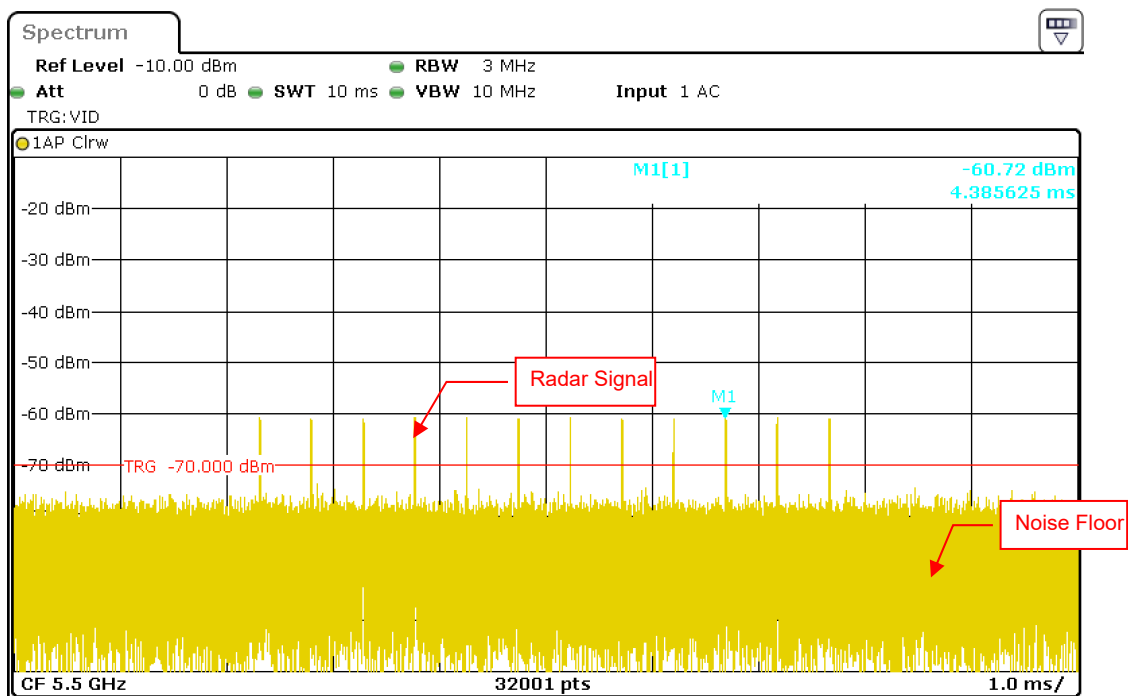
Radar Signal 4
