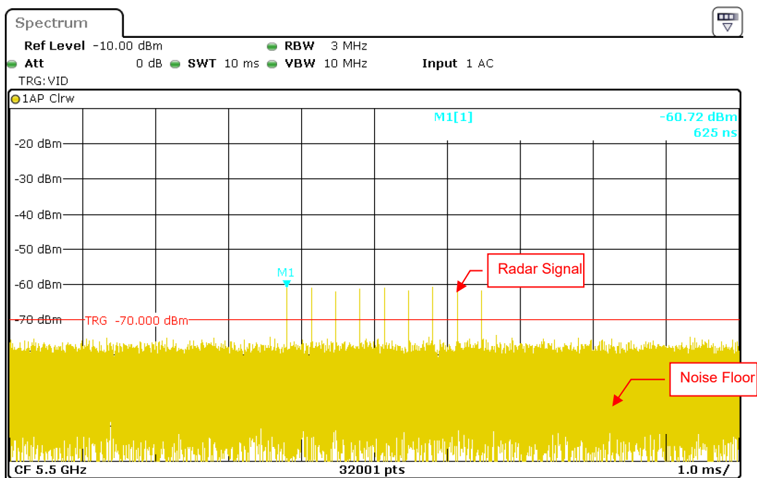
Radar Signal 6
