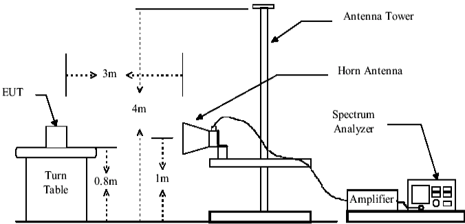
Above 1GHz
