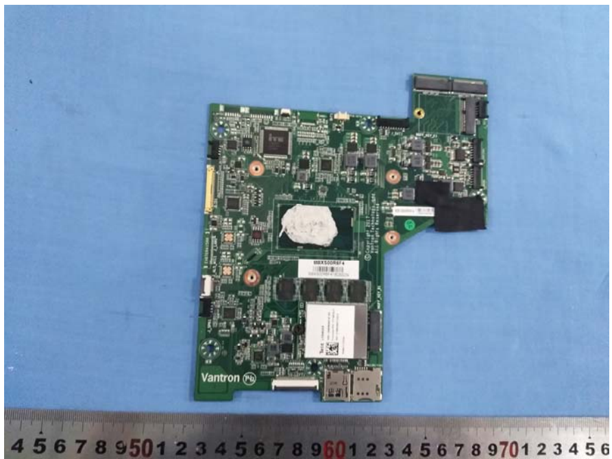
EUT – Mainboard Uncovered View
