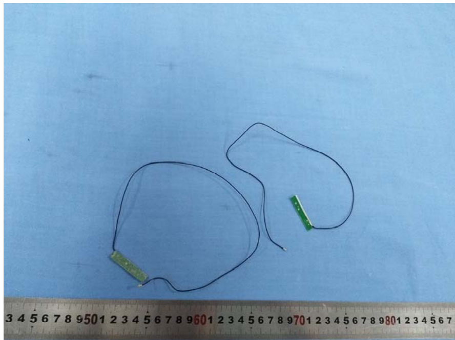
EUT – 7265NGW Wi-Fi Antenna View
