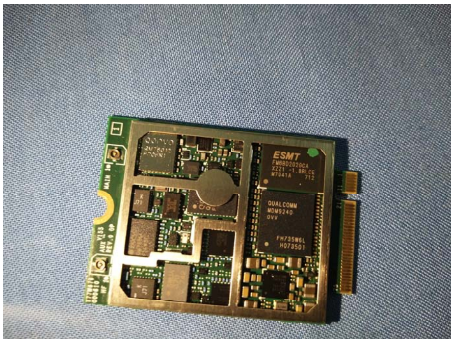
EUT – LTE Module Chip View
