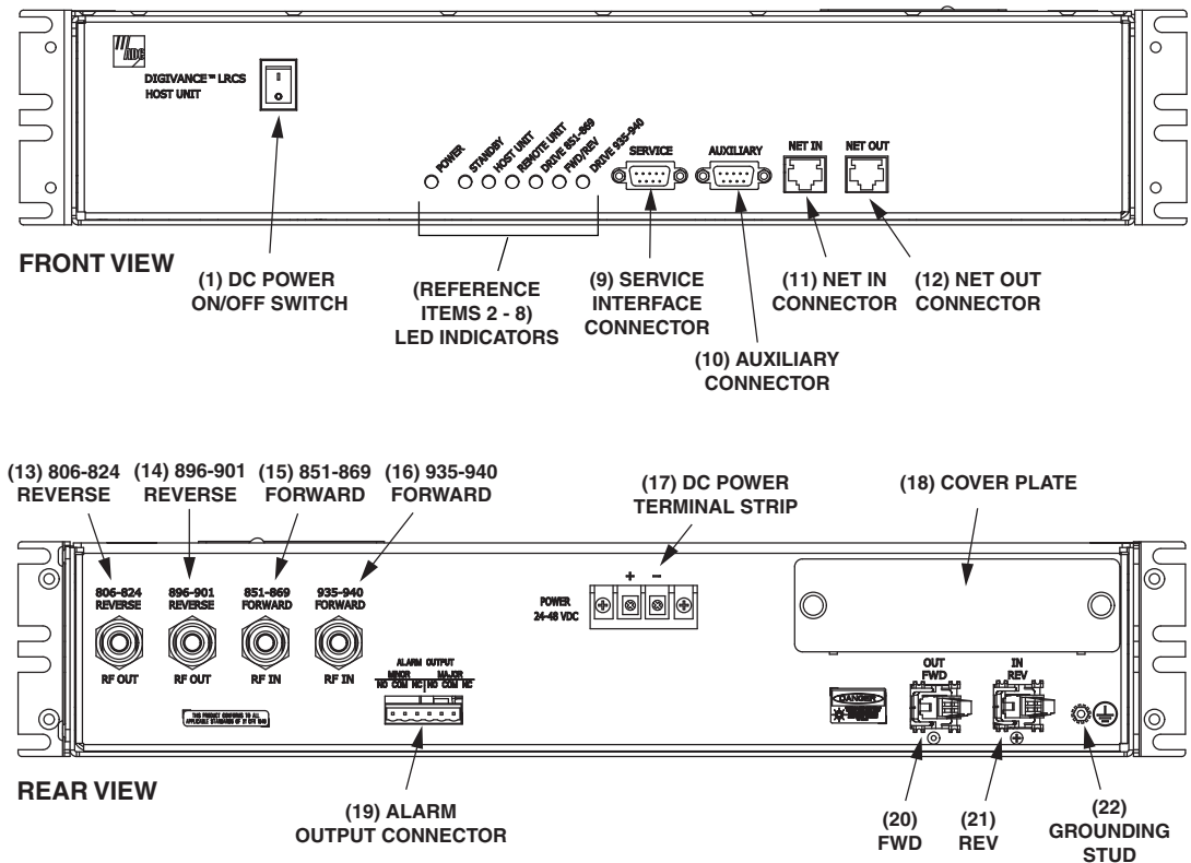
Figure 2-2. Typical Host Unit User Interface
