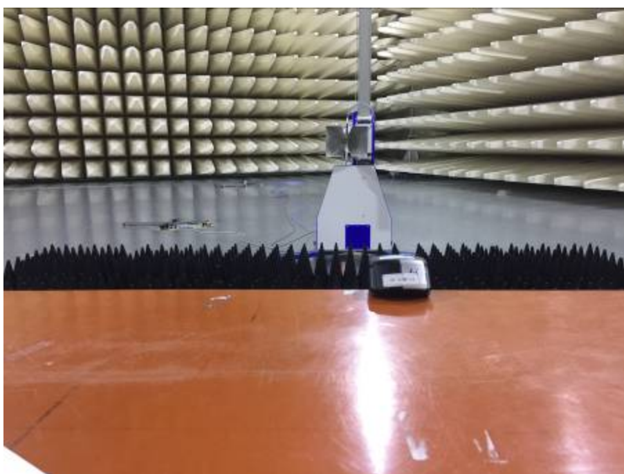
Spurious Radiated Emissions Test setup (>1GHz with charger)
