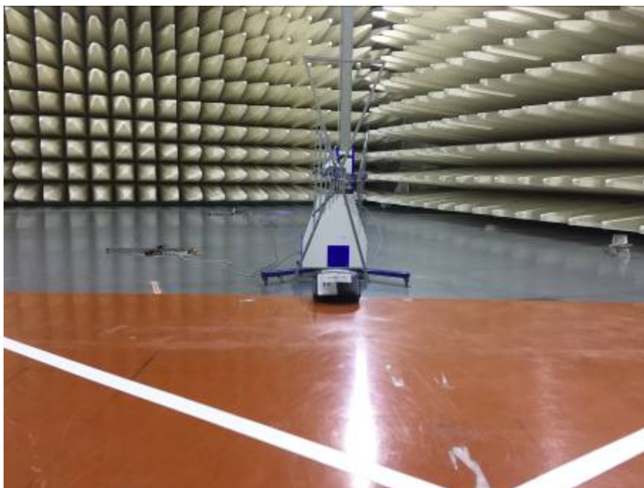
Spurious Radiated Emissions Test setup (30MHz~1GHz with charger)
