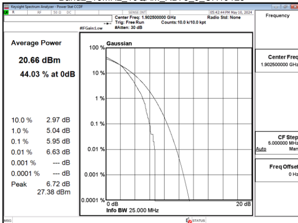
Band2_15MHz_16QAM_RB75_0_CH19125
