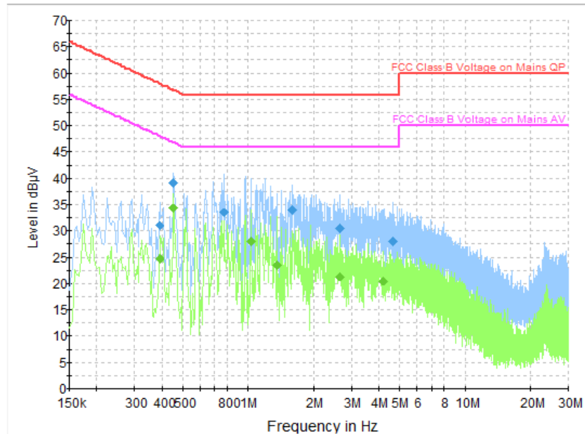
Fig.B.11.3 AC Powerline Conducted Emission-Idle
